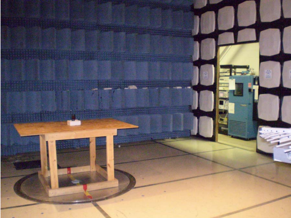
EMC Report #20813-1, Tx Radiated slider up
