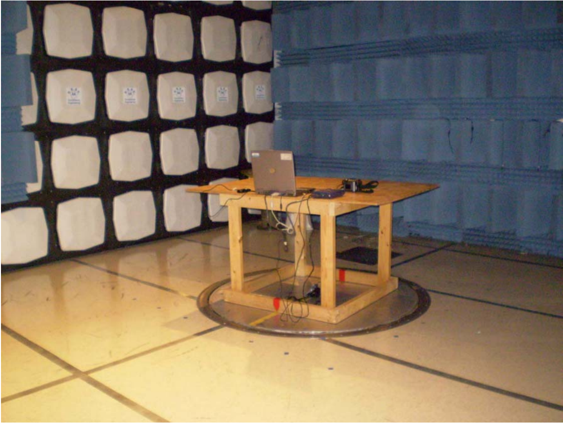
EMC Report #20813 Part 15, PC Peripheral
