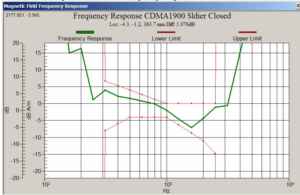
Graph 4: CDMA 1900 Frequency Response with Slider Closed
