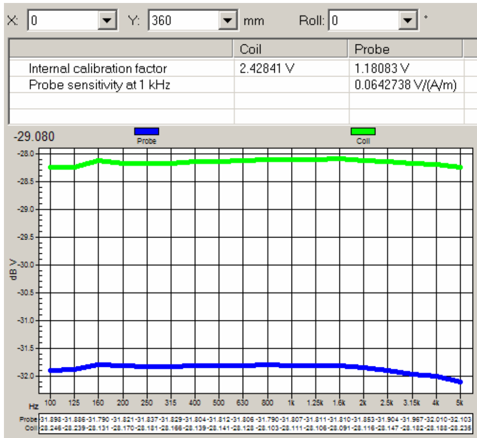
Graph 1: Frequency Response measured in AMCC
