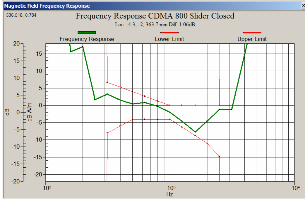
Graph 3: CDMA 800 Frequency Response with Slider Closed
