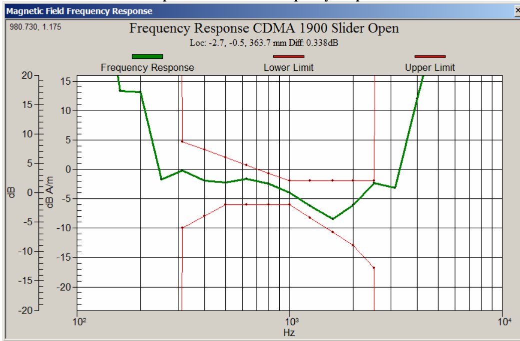
Graph 3: CDMA 1900 Frequency Response
