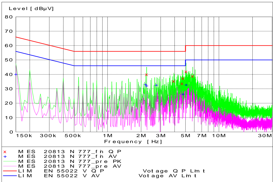
CDMA 800 Channel 777 - Tx Mode - Neutral Coupling
