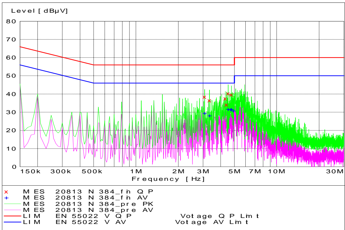
CDMA 800 Channel 384 - Tx Mode - Neutral Coupling
