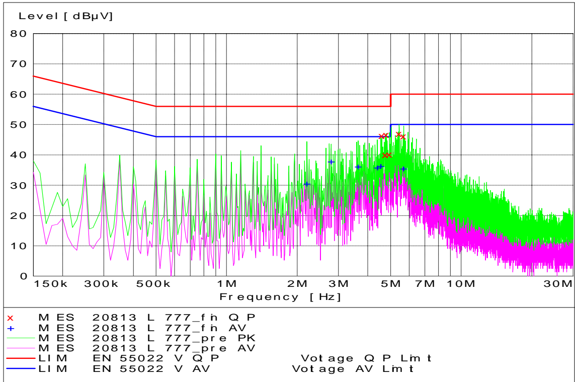
CDMA 800 Channel 777 - Tx Mode - Line Coupling
