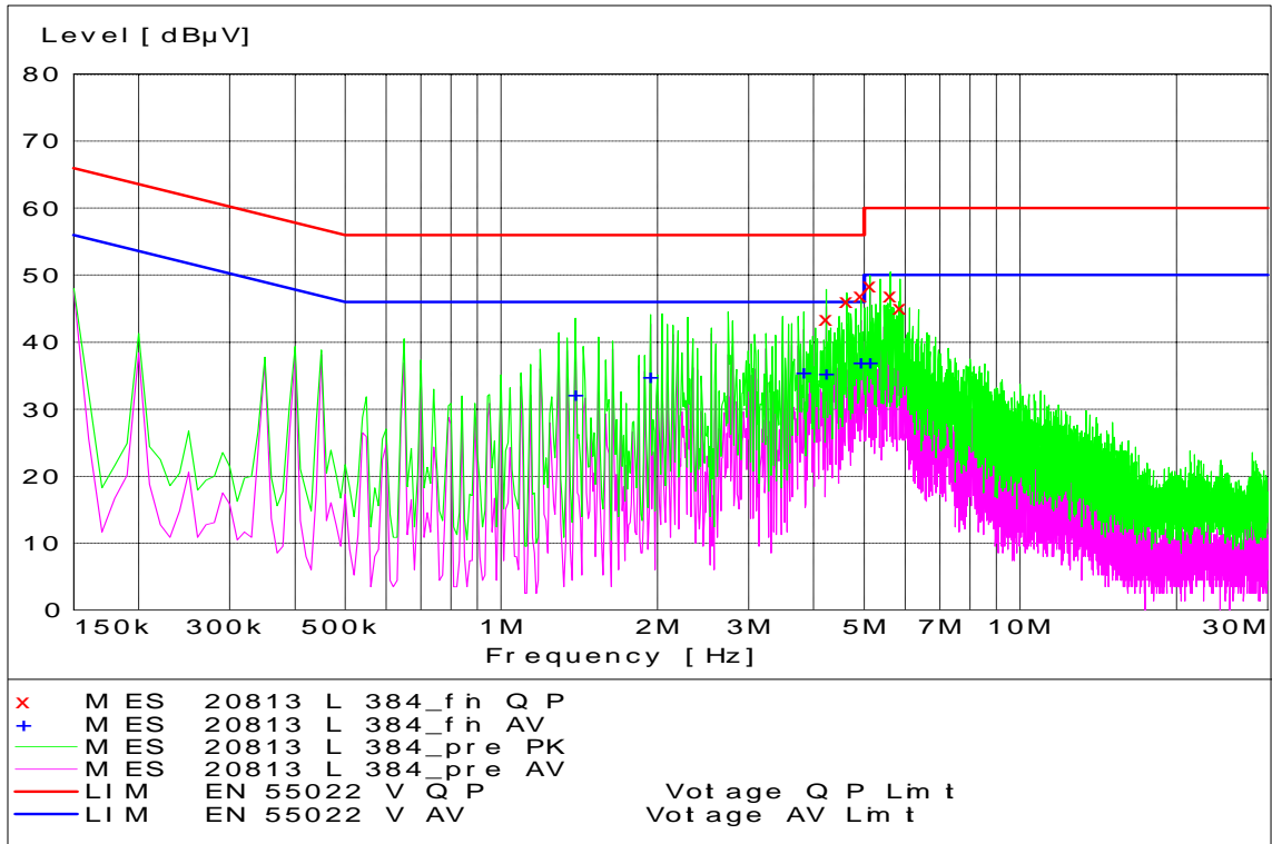
CDMA 800 Channel 384 - Tx Mode - Line Coupling
