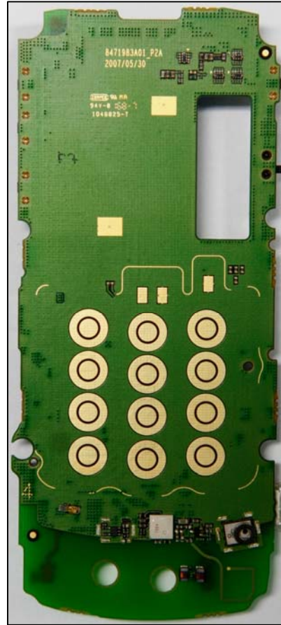
Main Board Top Without Popples
