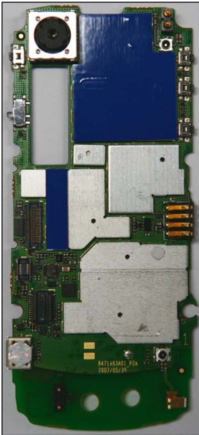
Main Board Bottom With Shields
