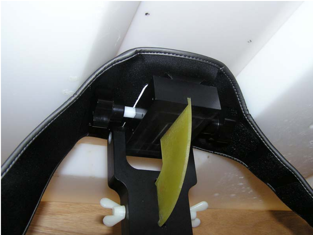
Figure 4 – Armband SYN2419A and Phone against Flat Phantom
