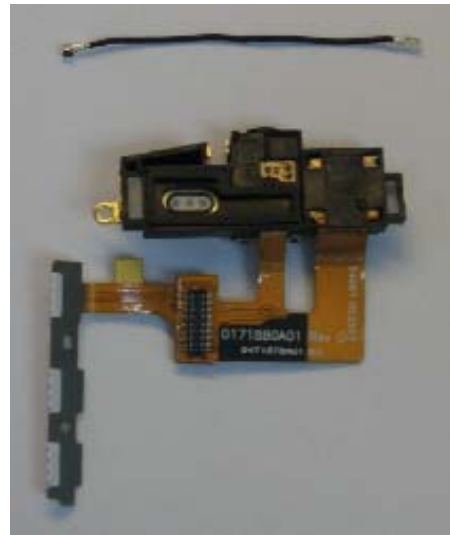
P-Flex Assembly / RF Coaxial Bottom
