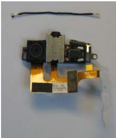
P-Flex Assembly / RF Coaxial Top
