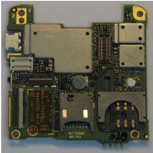
Main Board with shield Bottom
