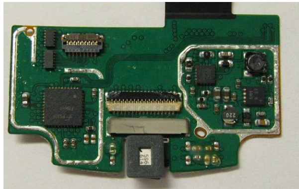
Slide PCB Without Shields
