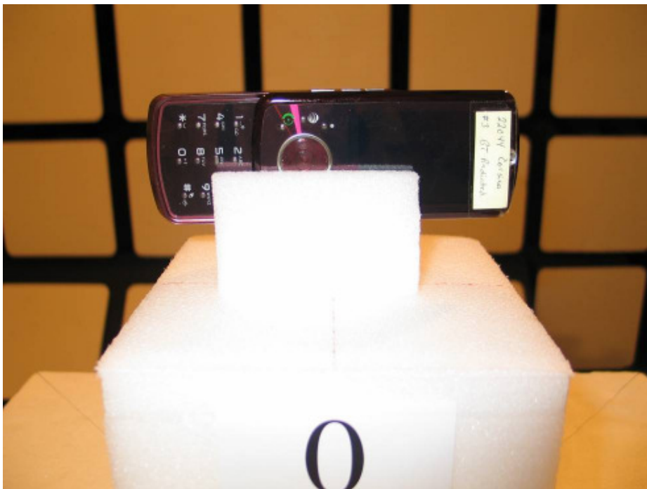
22044-1, IHDP56HA2 placed in test position Y
