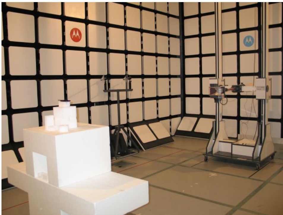
22044-1, IHDP56HA2 setup in semi-anechoic chamber – front view
