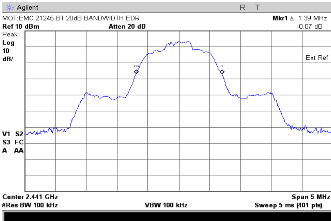
20dB Bandwidth EDR Mode Enabled
