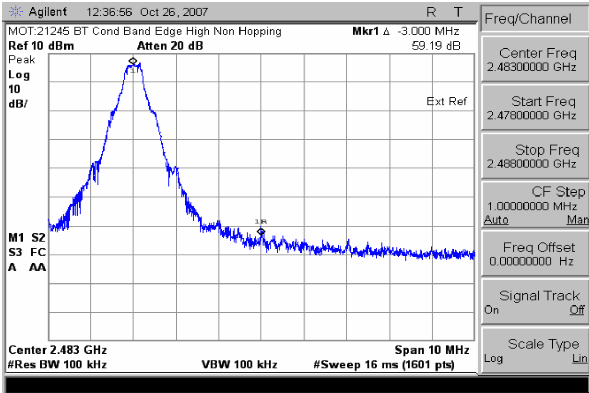
High Bandedge Non-EDR Mode with Hopping Disabled
