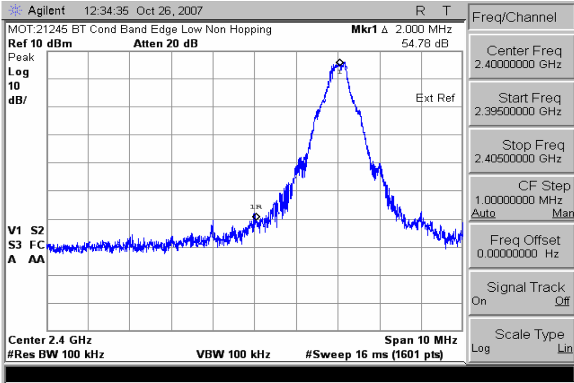
Low Bandedge Non-EDR Mode with Hopping Disabled
