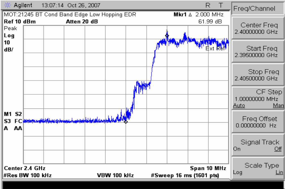
Low Bandedge EDR Mode with Hopping Enabled
