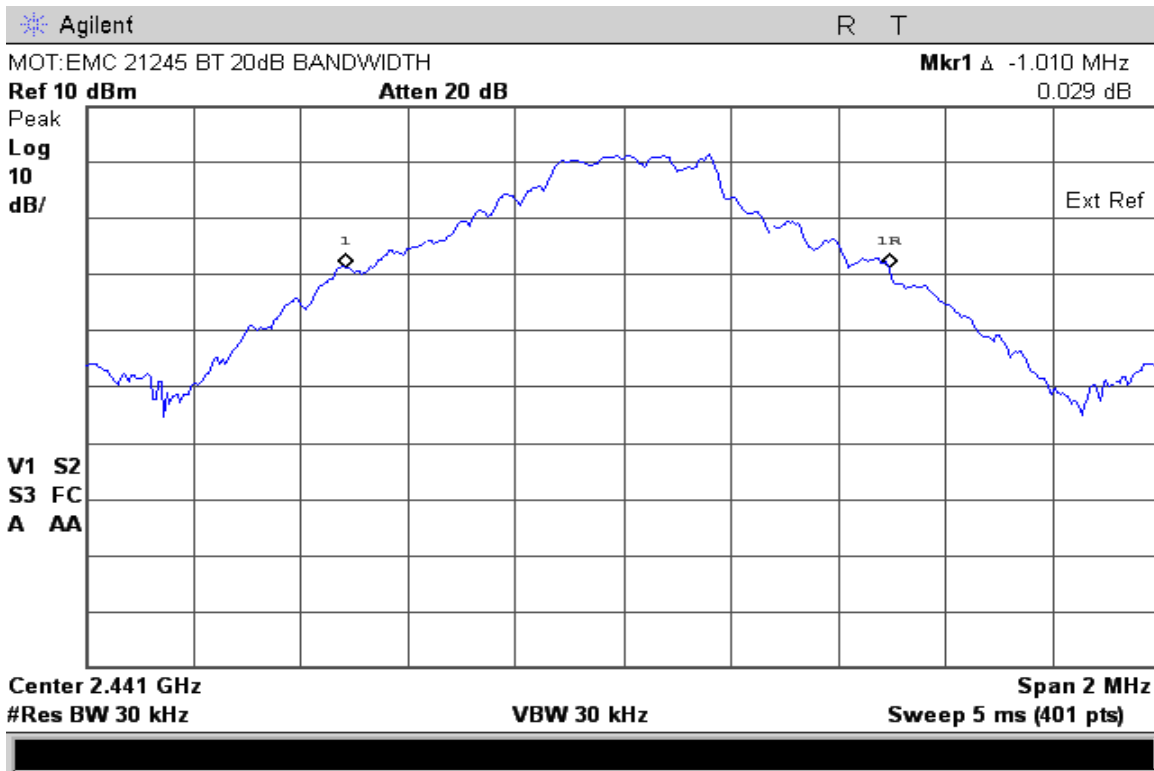
20dB Bandwidth Non-EDR Mode
