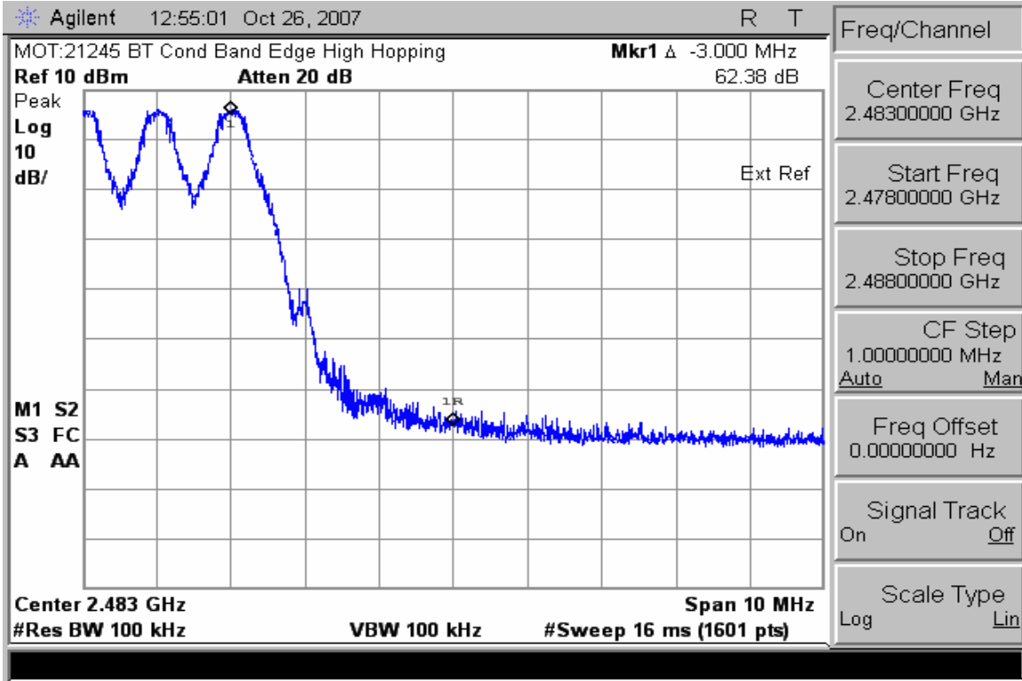
High Bandedge Non-EDR Mode with Hopping Enabled
