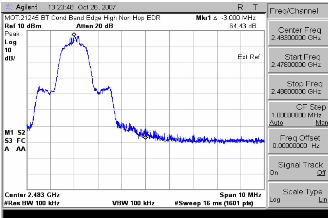
High Bandedge EDR Mode with Hopping Disabled
