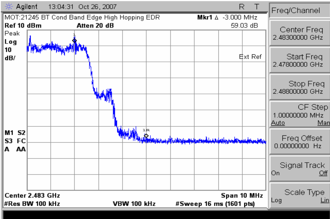
High Bandedge EDR Mode with Hopping Enabled
