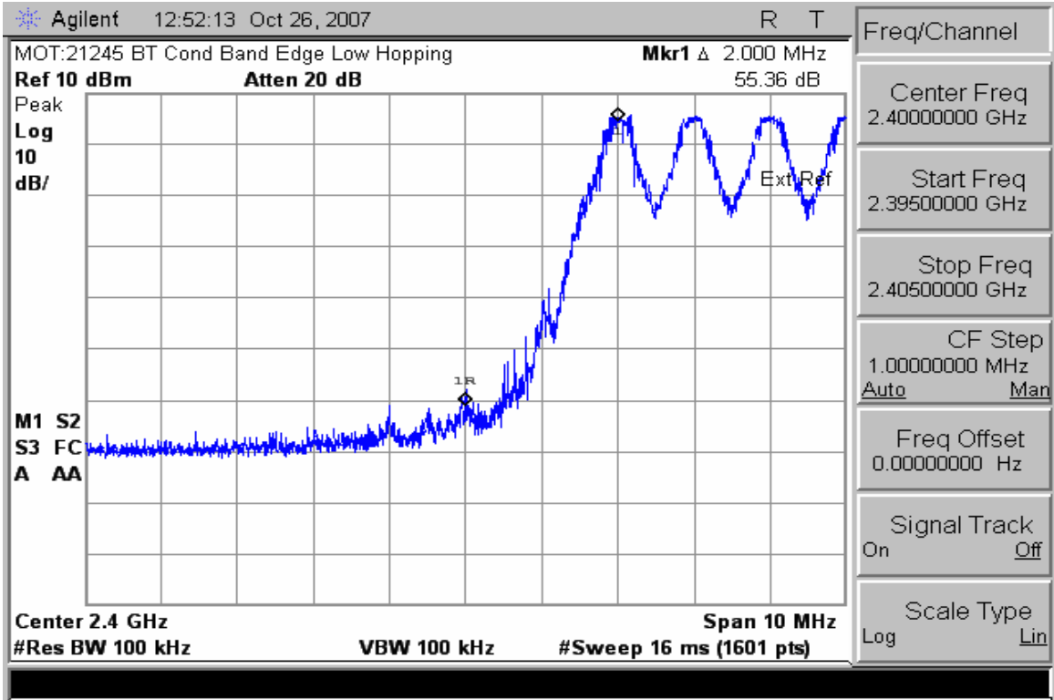
Low Bandedge Non-EDR Mode with Hopping Enabled
