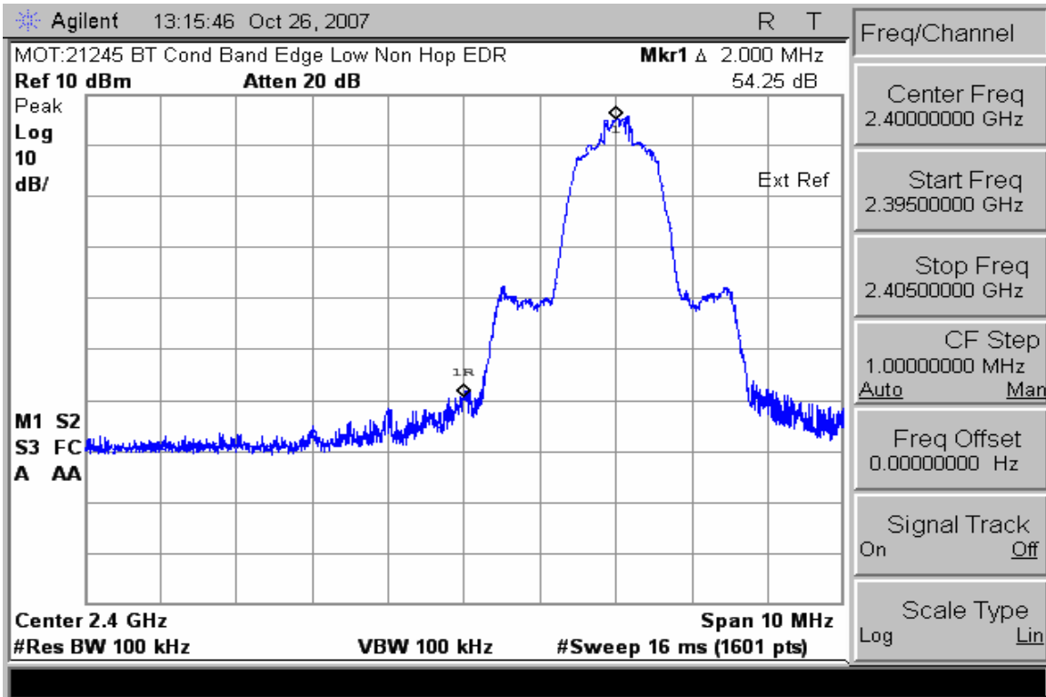
Low Bandedge EDR Mode with Hopping Disabled
