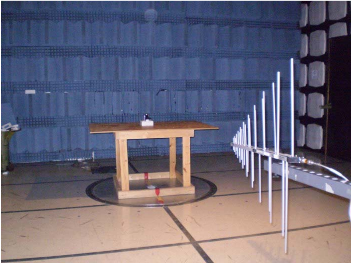
EMC Report #22044 Tx Radiated
