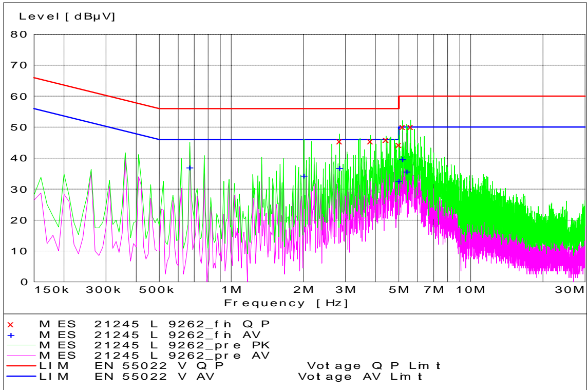
WCDMA 1900 Channel 9262 - Tx Mode - Line Coupling
