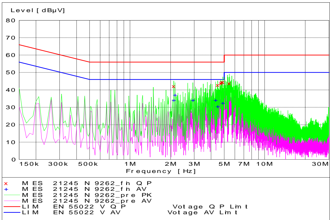
WCDMA 1900 Channel 9262 - Tx Mode - Neutral Coupling
