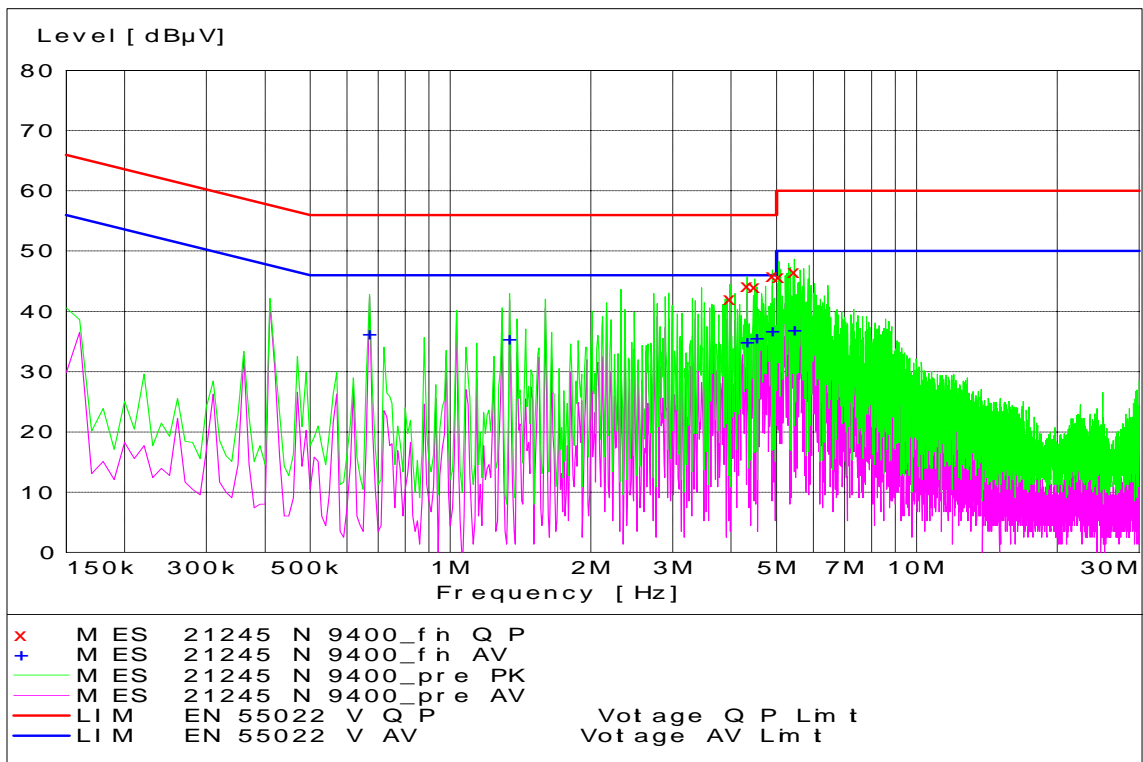
WCDMA 1900 Channel 9400 - Tx Mode - Neutral Coupling
