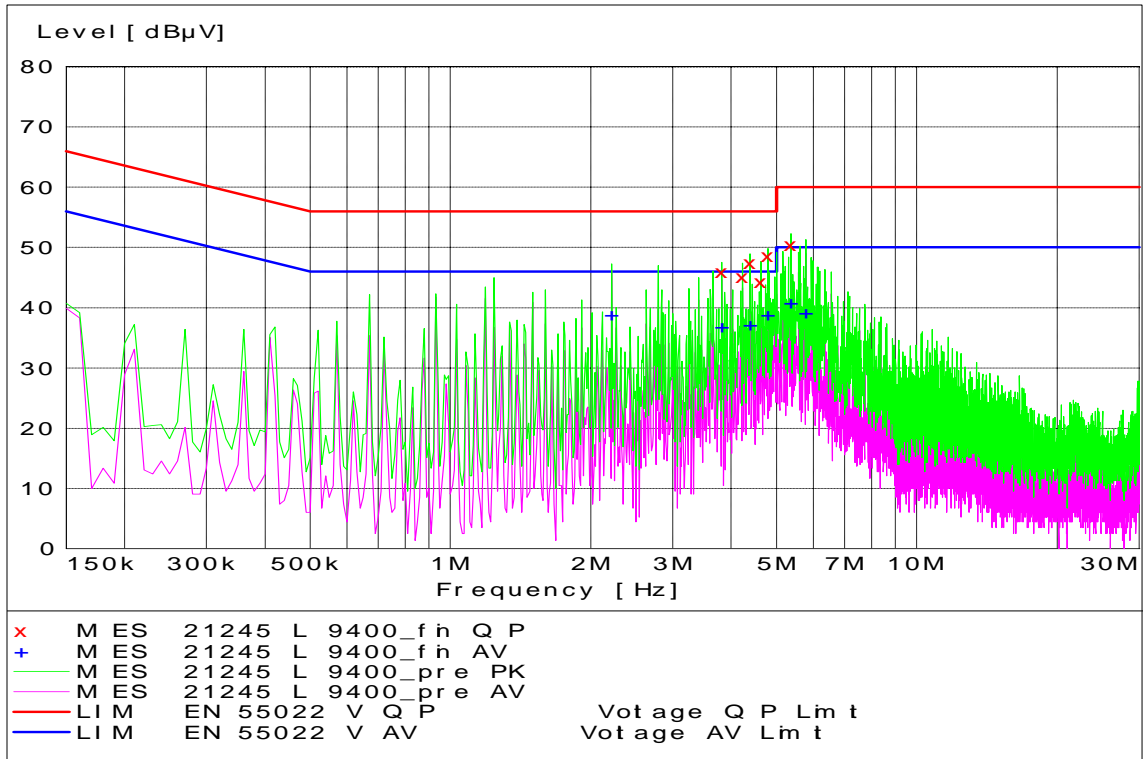
WCDMA 1900 Channel 9400 - Tx Mode - Line Coupling
