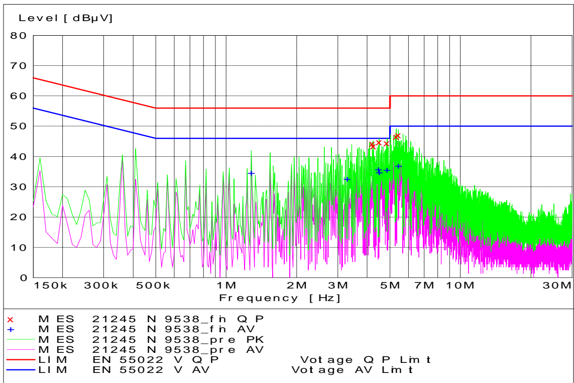
WCDMA 1900 Channel 9538 - Tx Mode - Neutral Coupling
