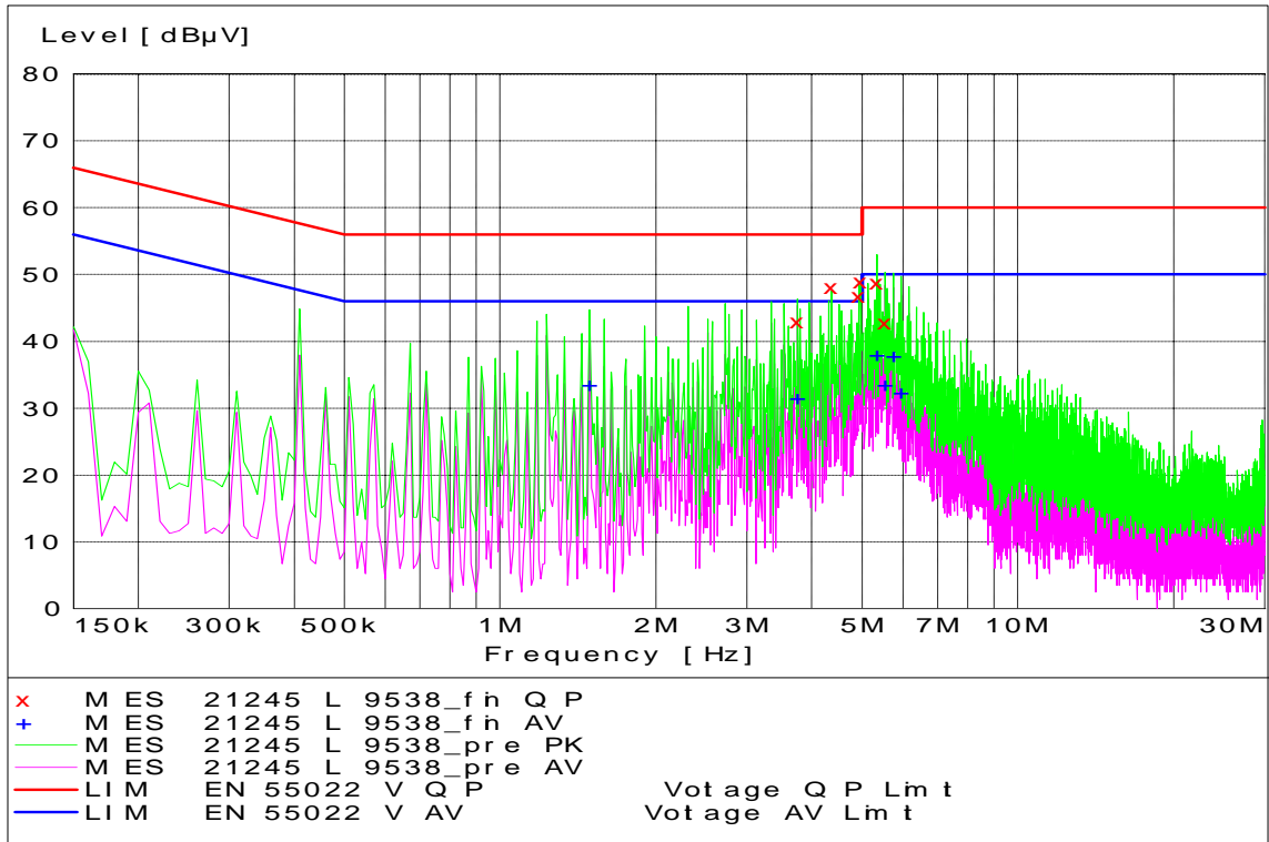
WCDMA 1900 Channel 9538 - Tx Mode - Line Coupling
