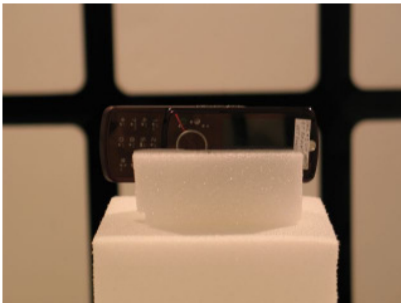
21245-1, IHDP56HA1 placed in test position Y
