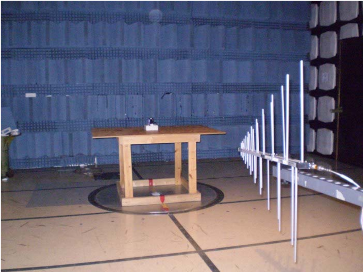
EMC Report #21245 Tx Radiated
