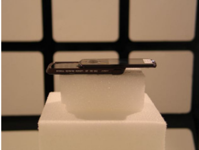
21245-1, IHDP56HA1 placed in test position X
