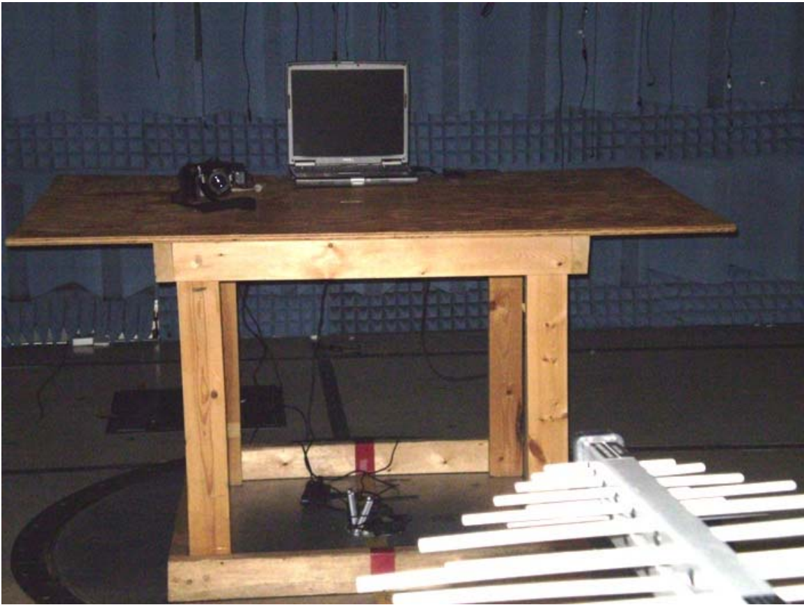
EMC Report #21245 Part 15, PC Peripheral
