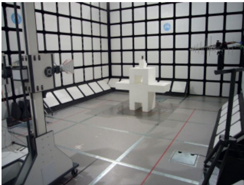
21245-1, IHDP56HA1 setup in semi-anechoic chamber
