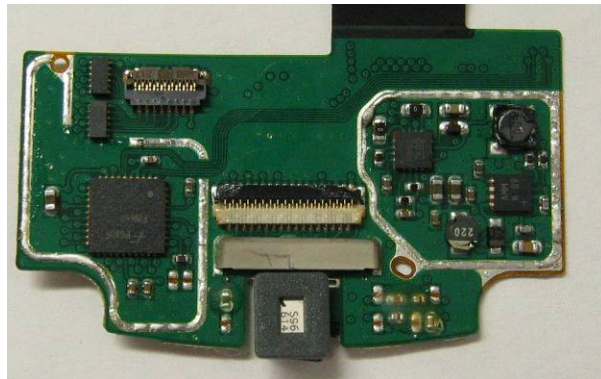
Slide PCB Without Shields
