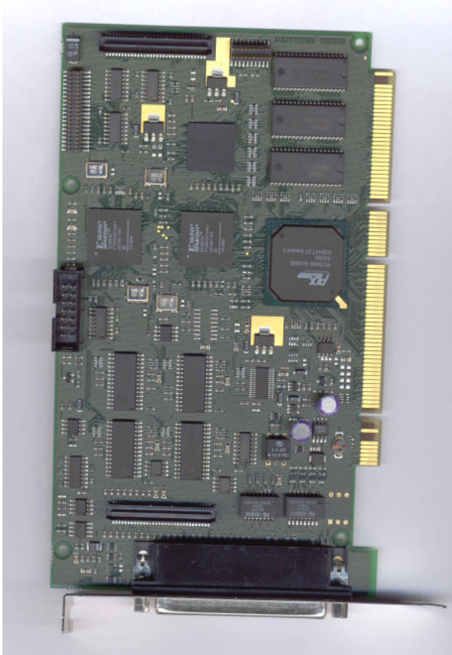
Components side
