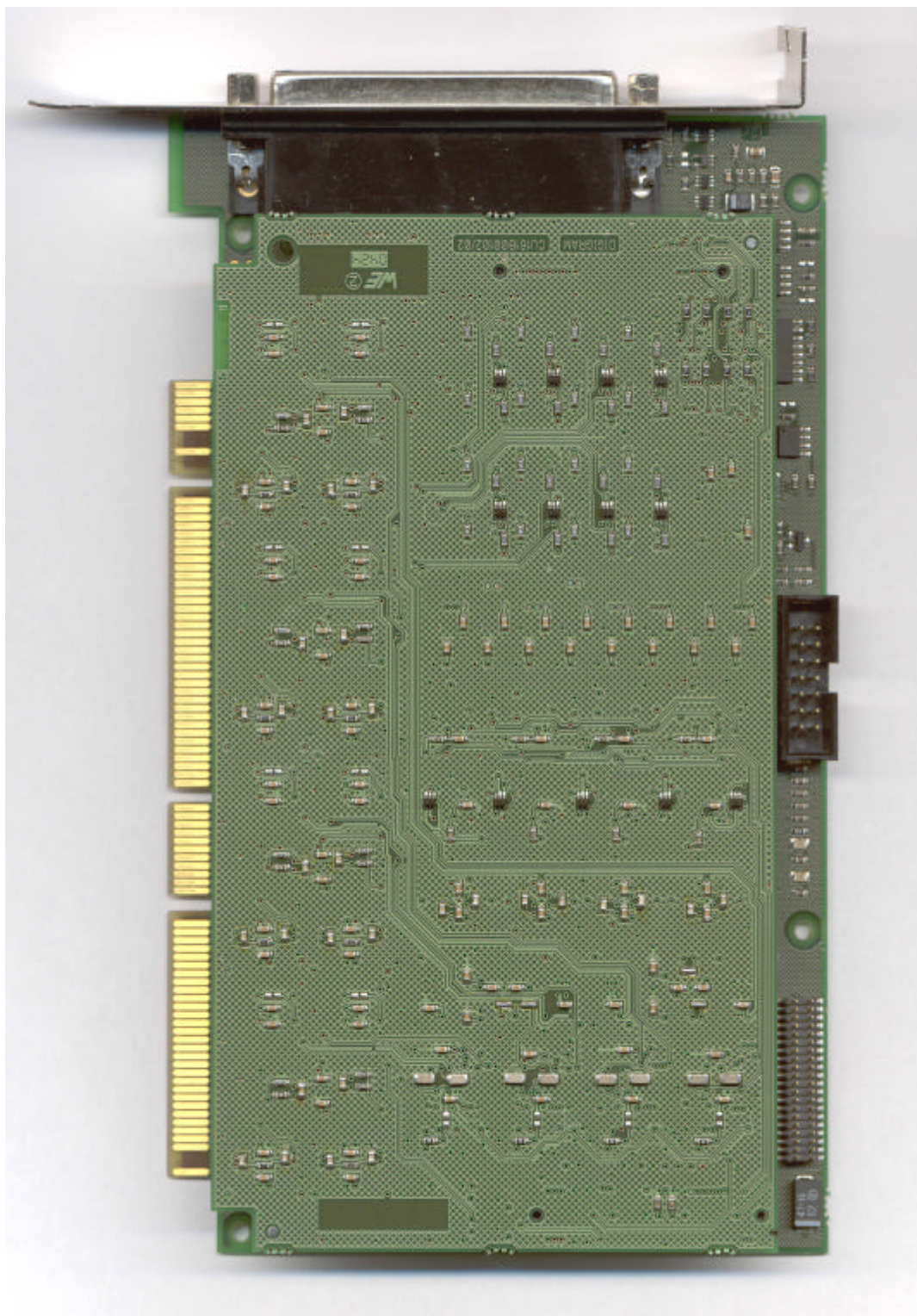
Mother board with daughter board (only for PCX&VX882HR)
