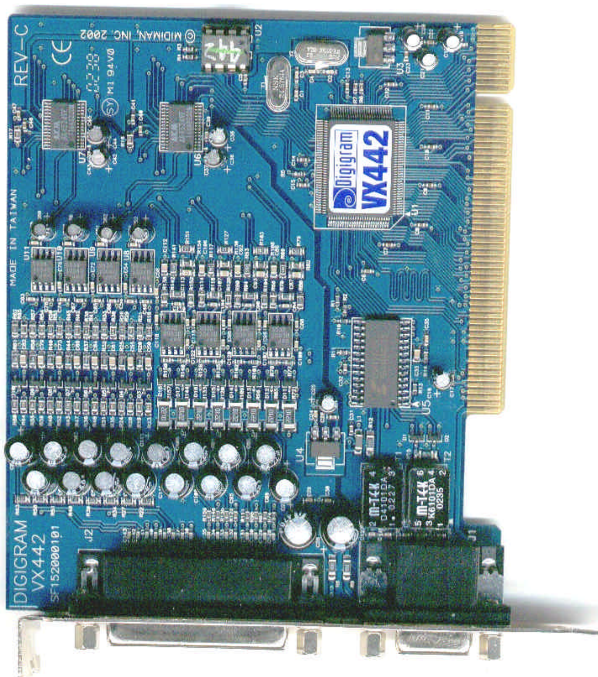
Components side
