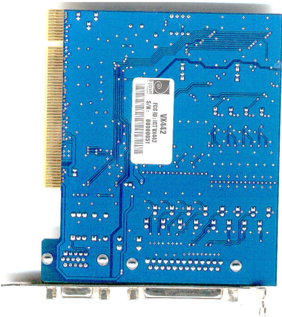
Rear side
