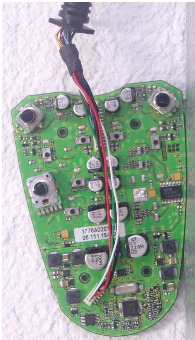
PCB views (UAX220-MIC & UAX220-v2)
