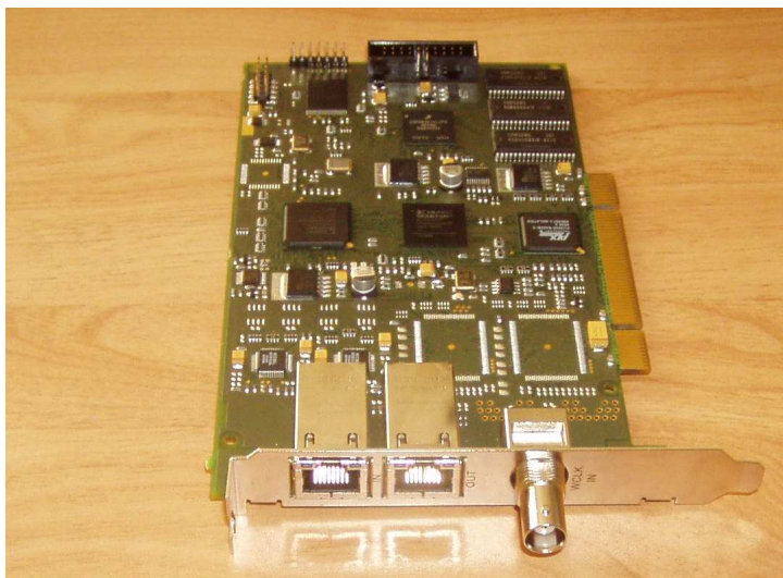
Connectors view
