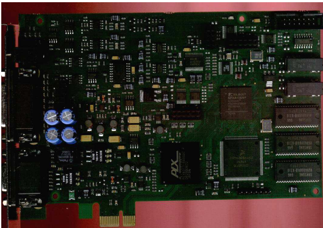
Components view (main board with MIC option)
