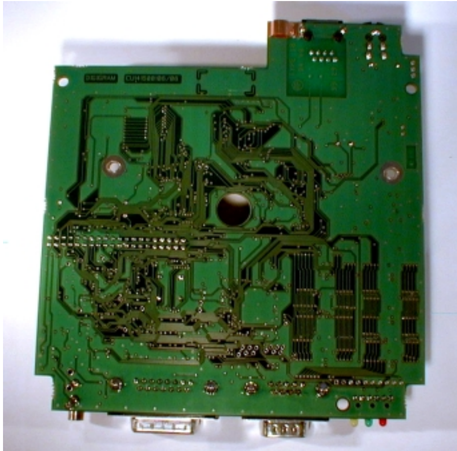
CPU board, foil side
