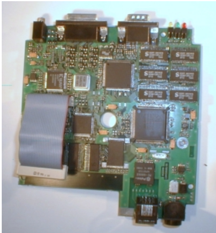
CPU board, component side
