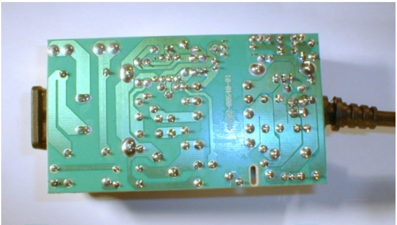
Foil side
