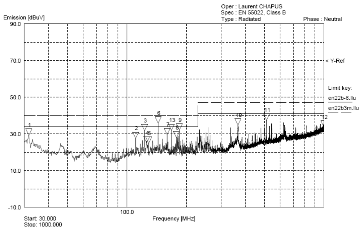
RADIATED EMISSIONS - DIGIGRAM
