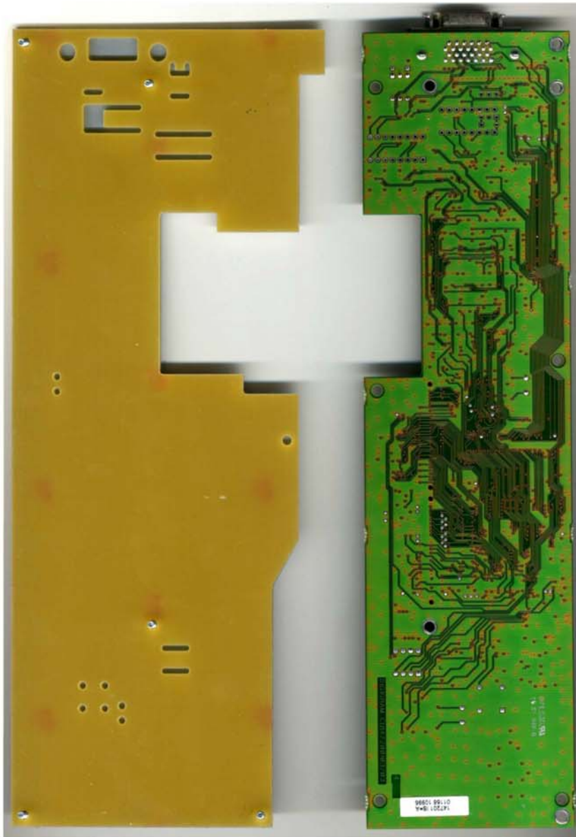
miXart8 AES-EBU (optional card), front panel removed and view of copper side
