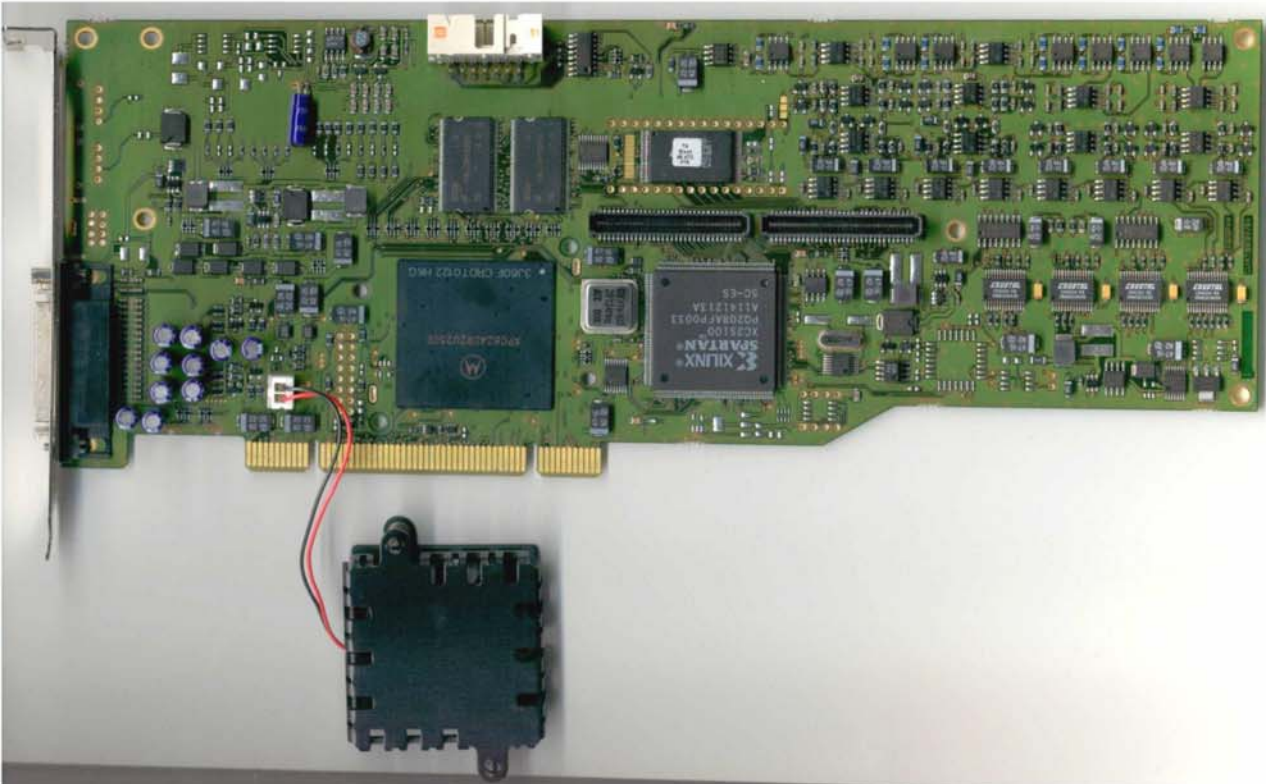
miXart8 (main card), components side with CPU fan removed.
