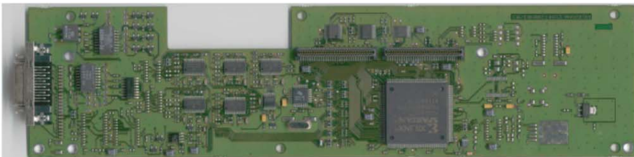
miXart8 AES-EBU (optional card), view of components side
