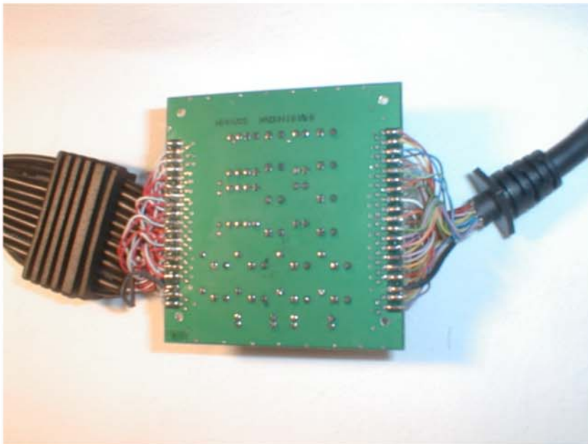
Breakout analog cable (copper side)
