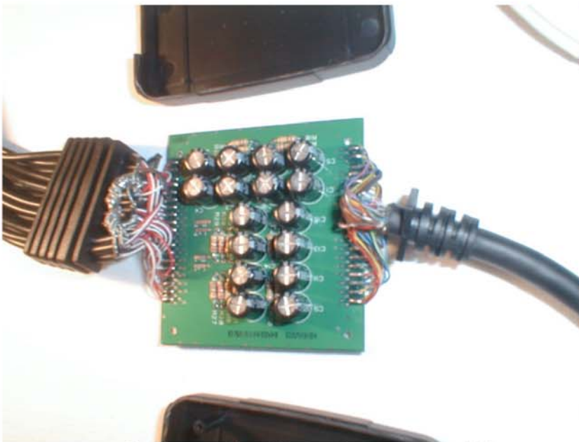
Breakout analog cable (passive components side)
