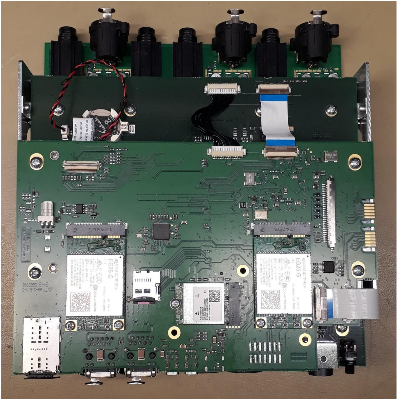
All Boards, all casing removed – view 2
