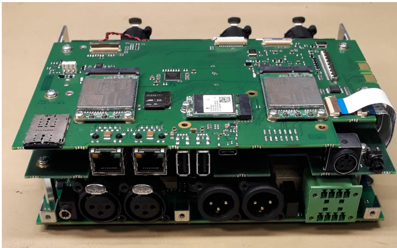
All Boards, all casing removed – view 1
