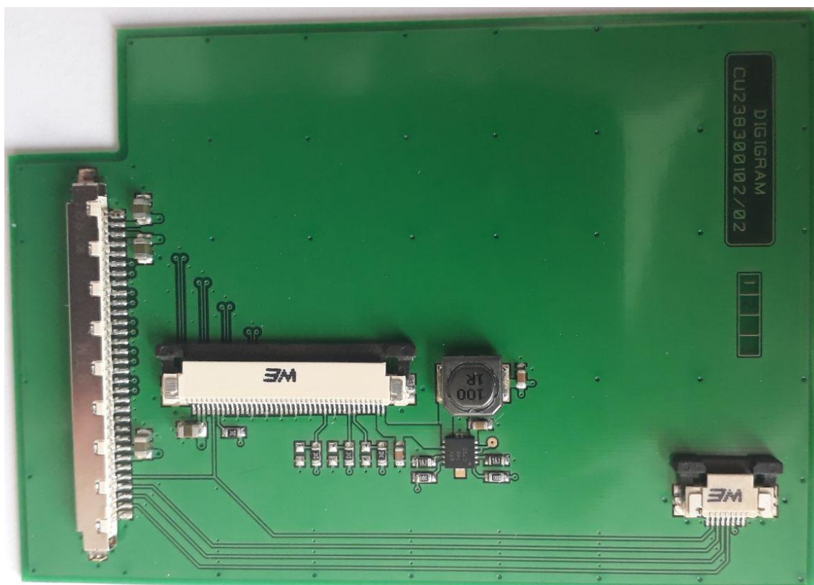
Board 'lcd' top
