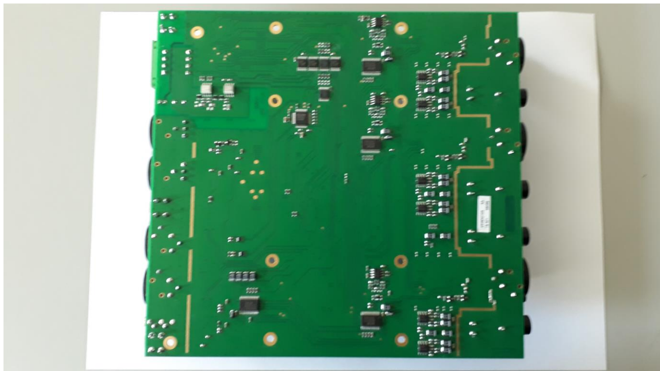
Board 'analog' bottom
