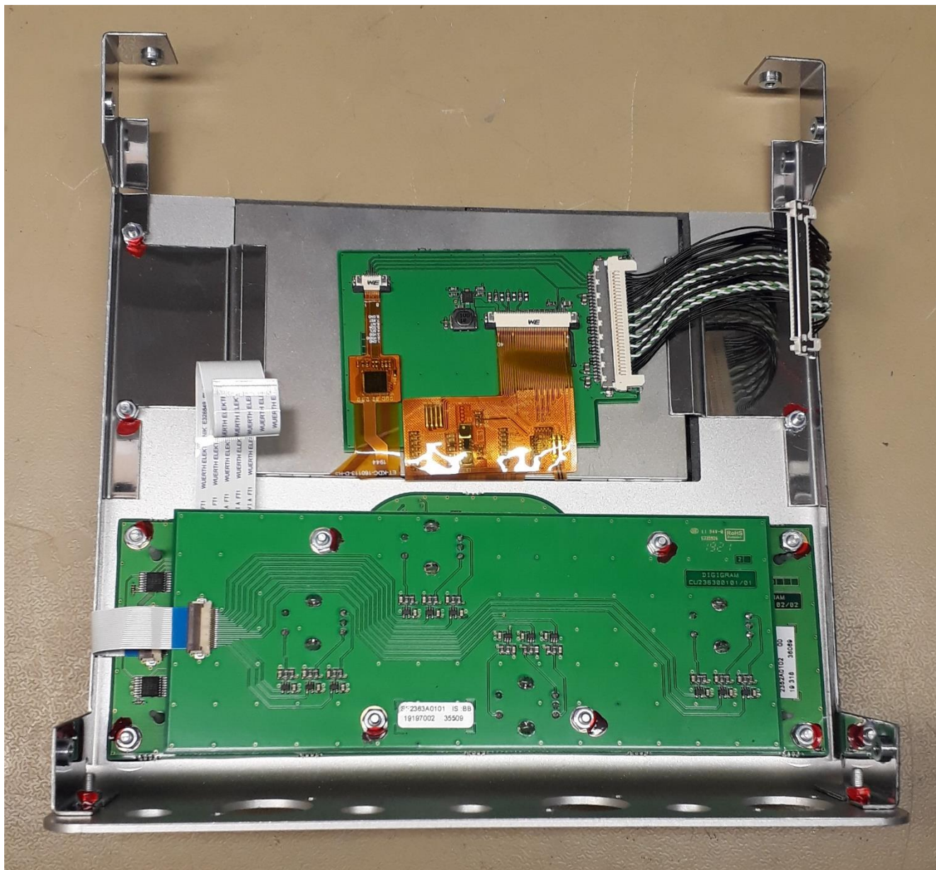
Boards, all casing removed – view 5
