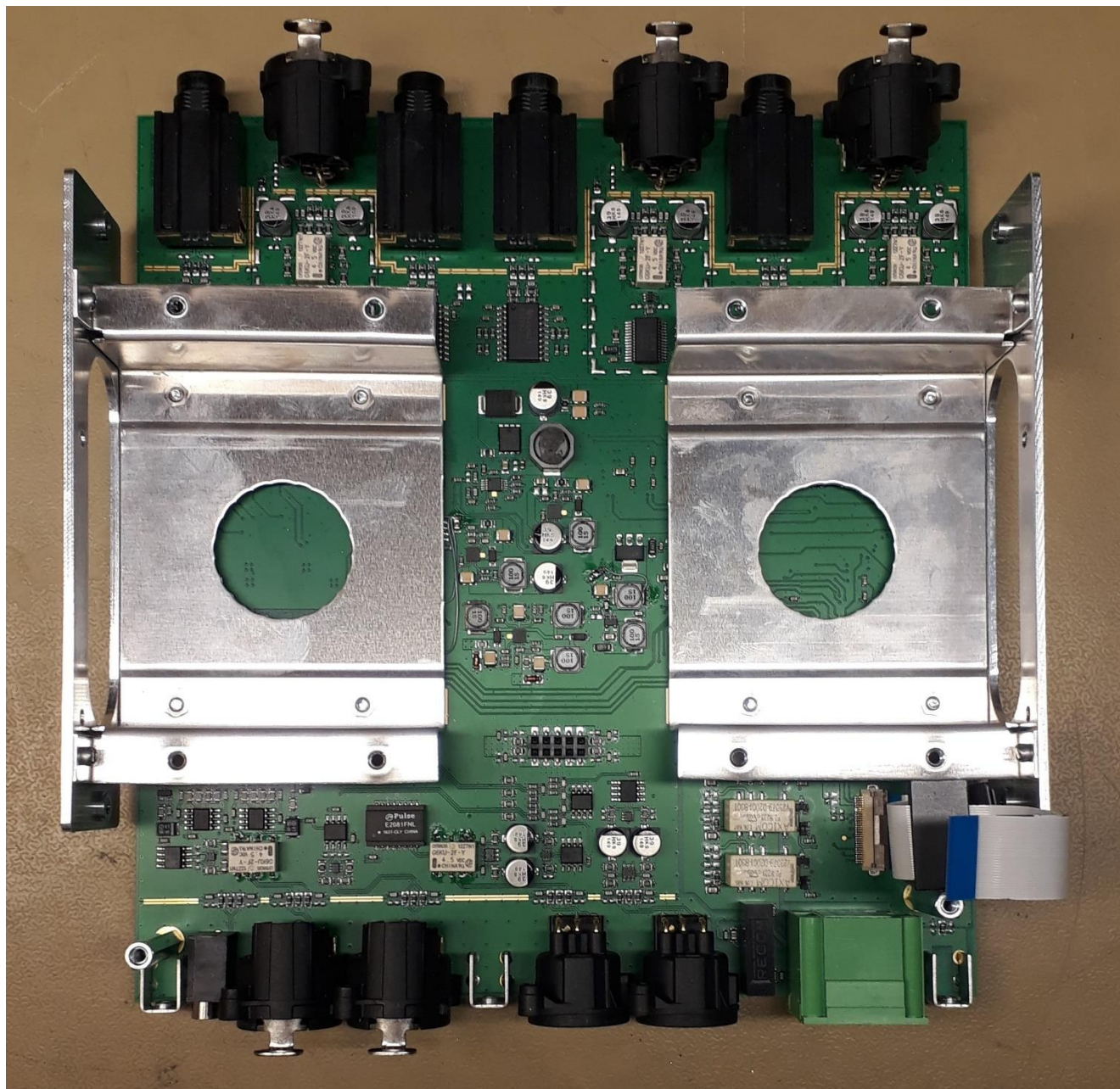
Boards, all casing removed – view 4
