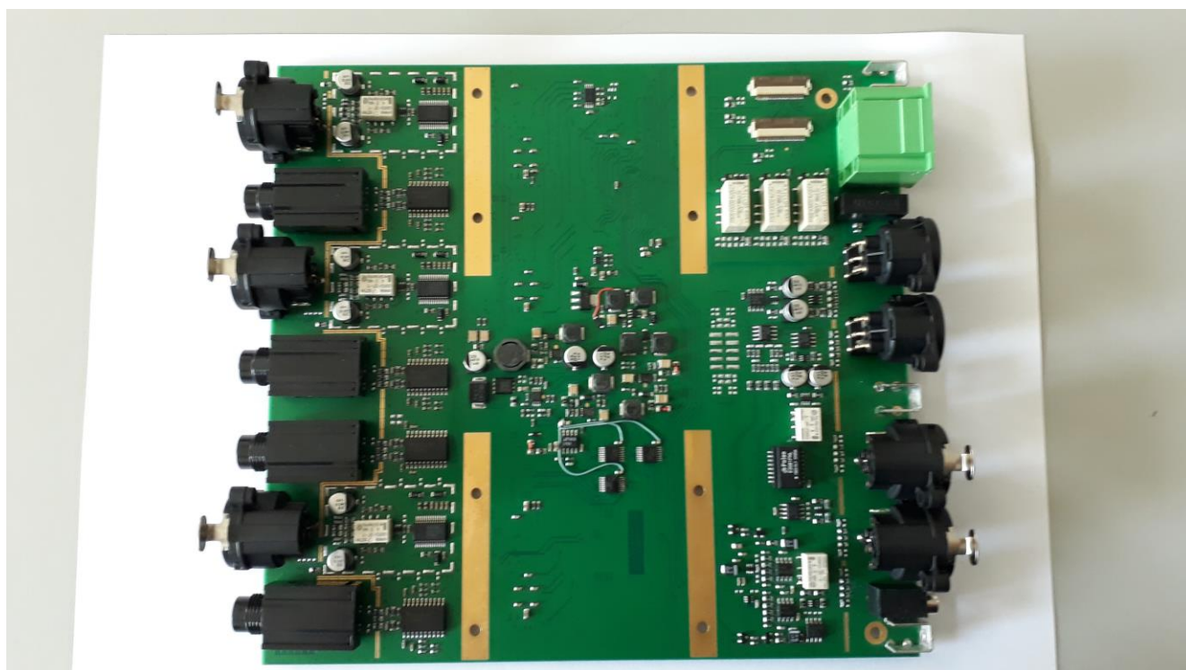
Board 'analog' top
