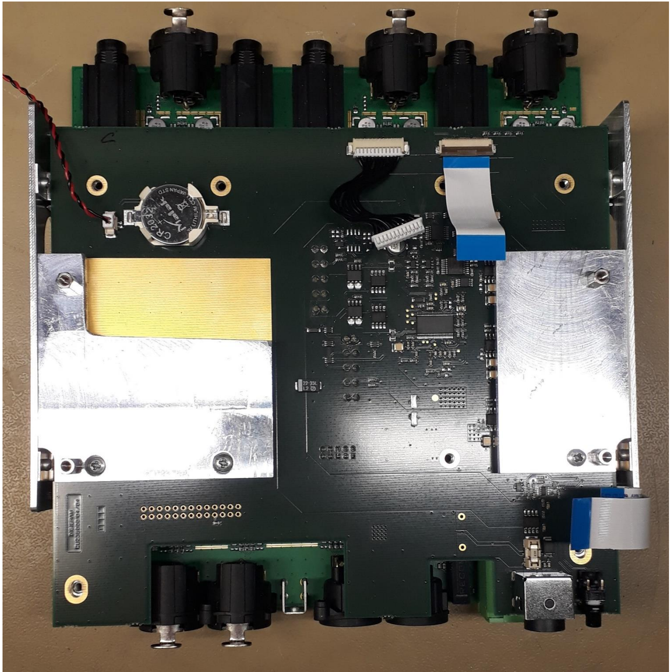
Boards, all casing removed – view 3
