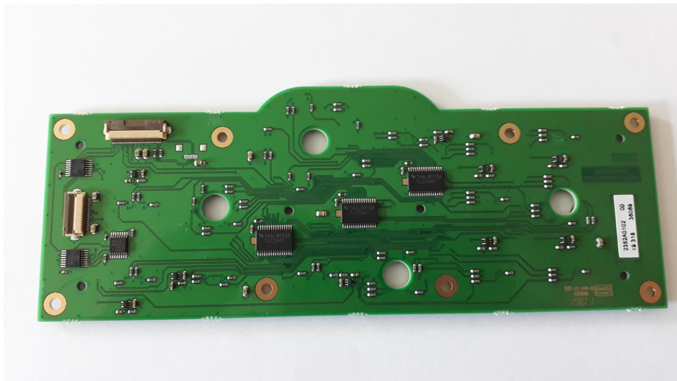
Board 'push button' bottom
