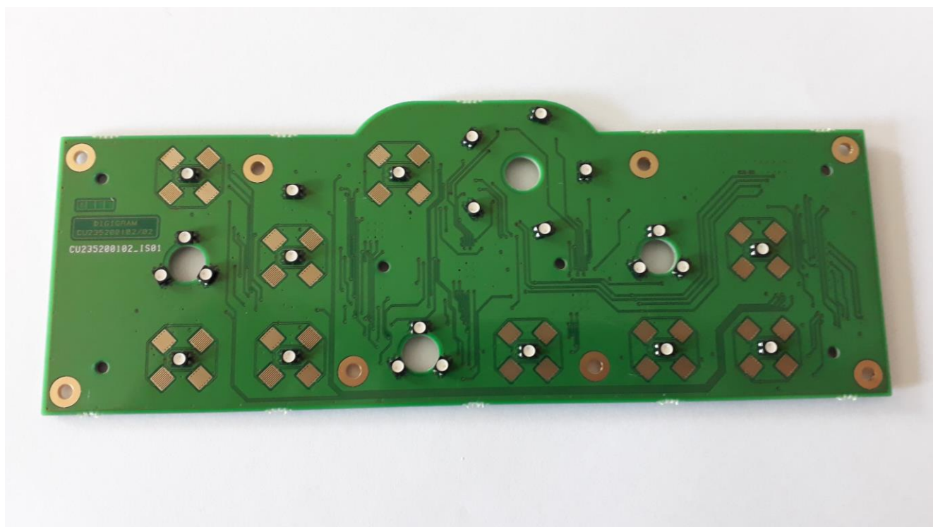
Board 'push button' top
