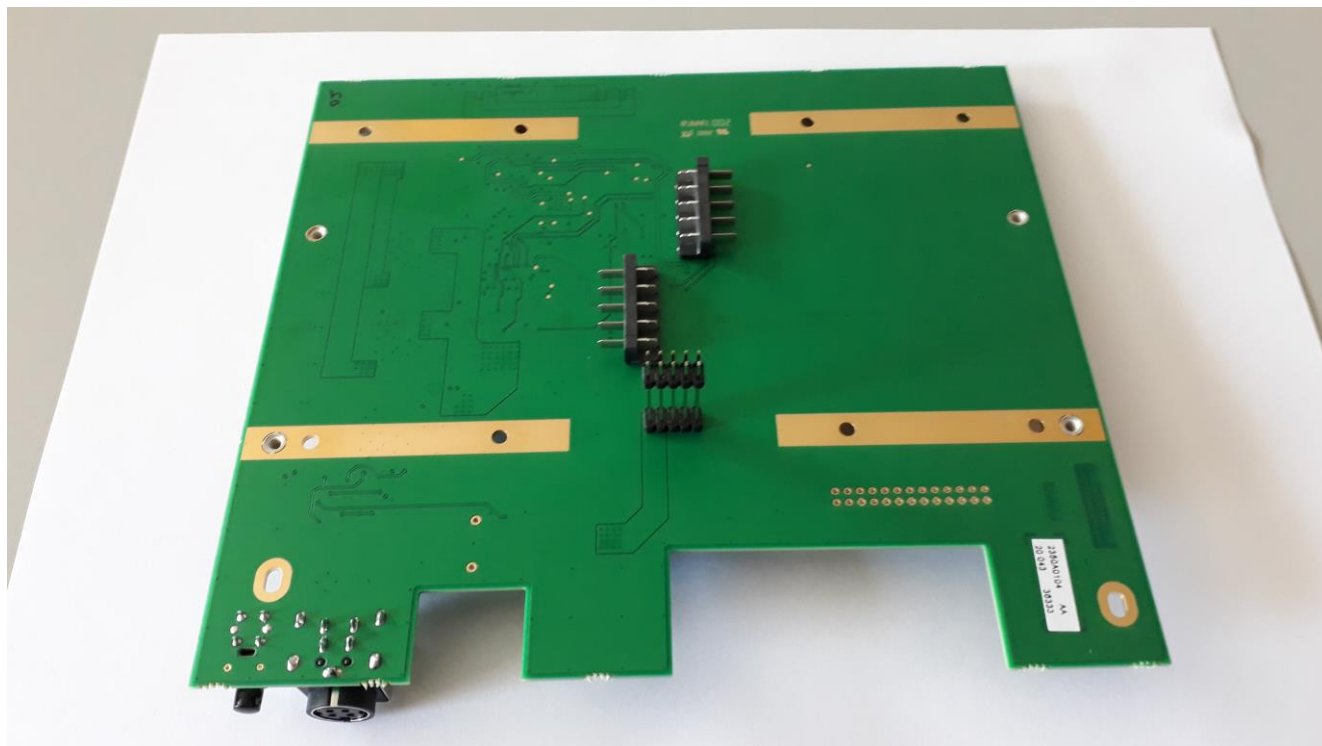
Board 'power' bottom
