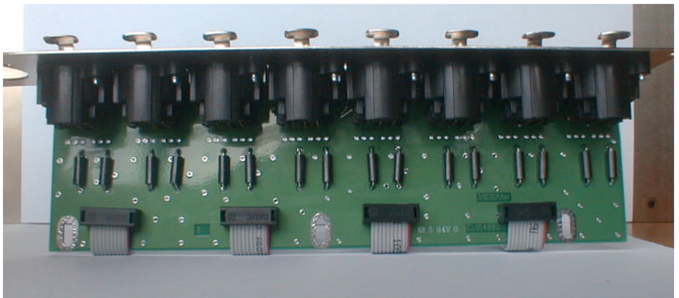
XLR connector board (ES8 IN &OUT)
