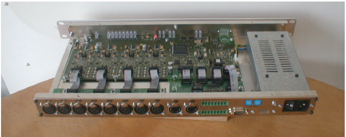
General view, cover removed, rear face (ES8 IN & OUT – XLR connectors)
