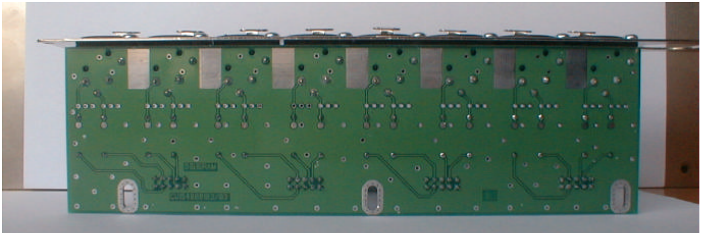
XLR connector board (ES8 IN &OUT)
