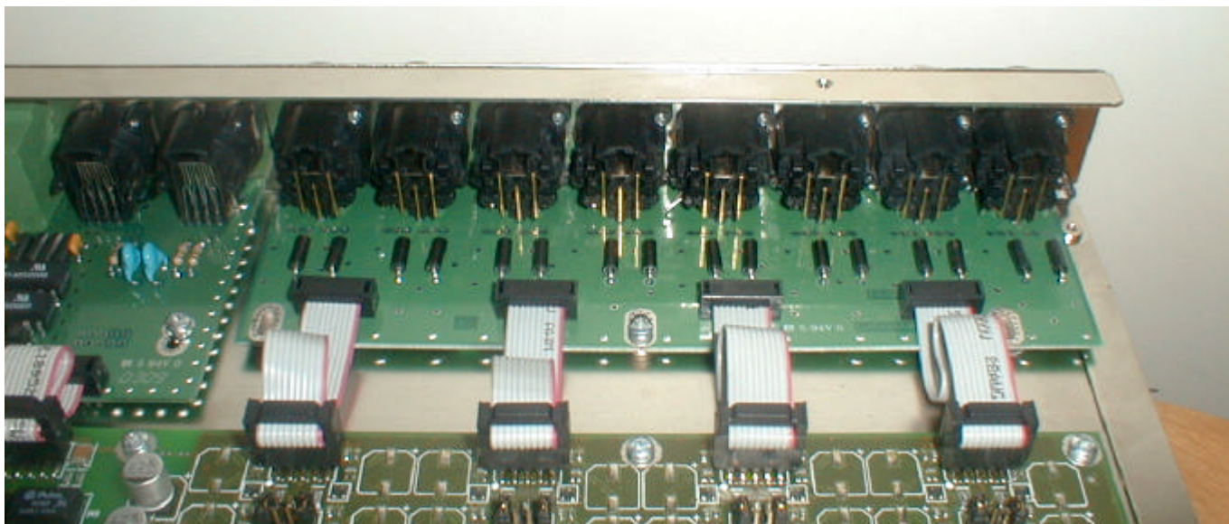
Detail view, ES8 IN & OUT, XLR connector board
