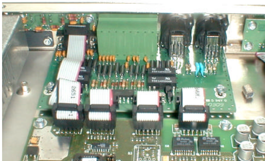
Detail view, ES8 IN & OUT, Ethernet+GPIO+RS232 connector board
