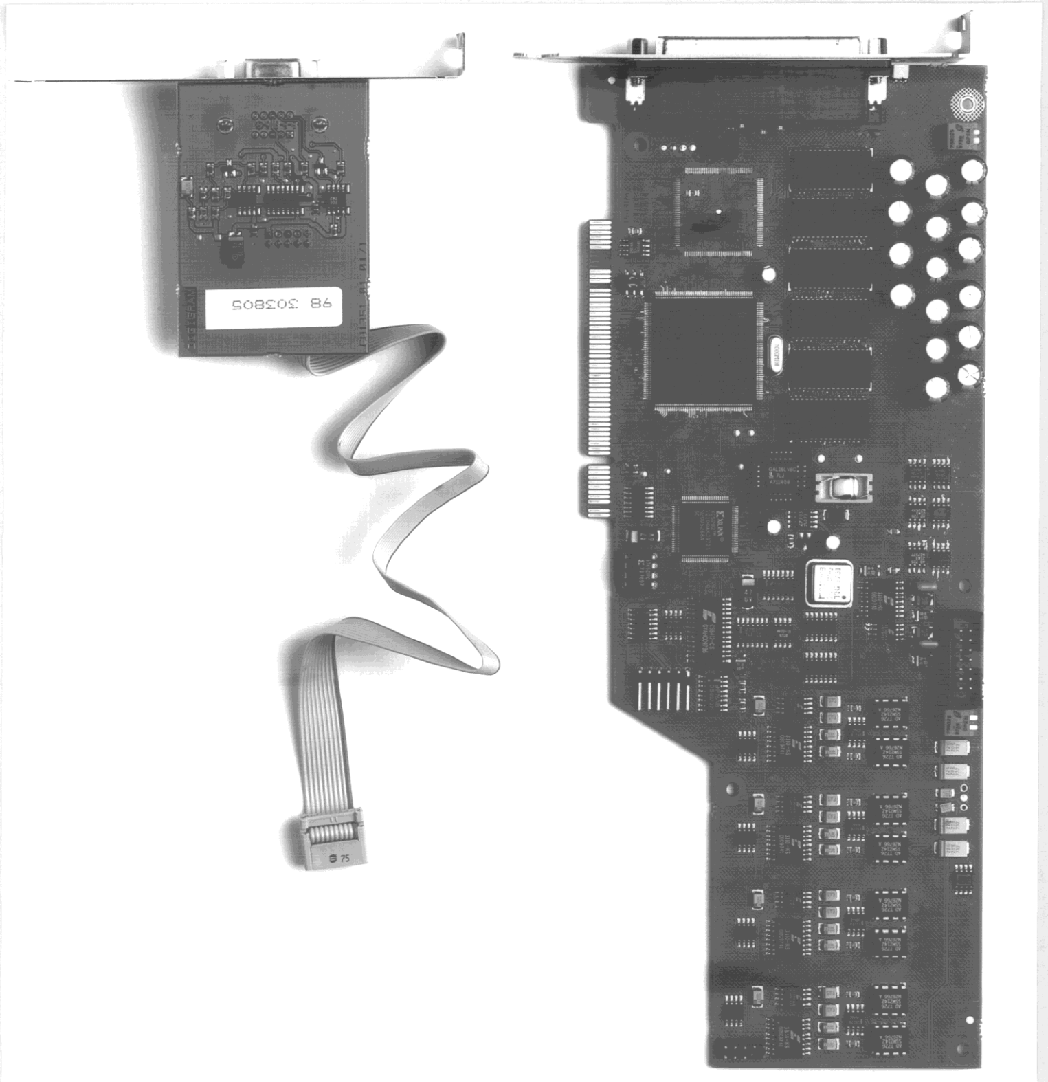
Figure 8.2..PCX820np and option Board, component side
