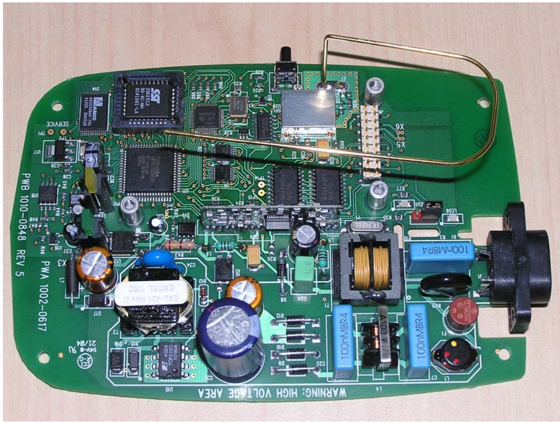
EUT – PCB Top view without GSM module
