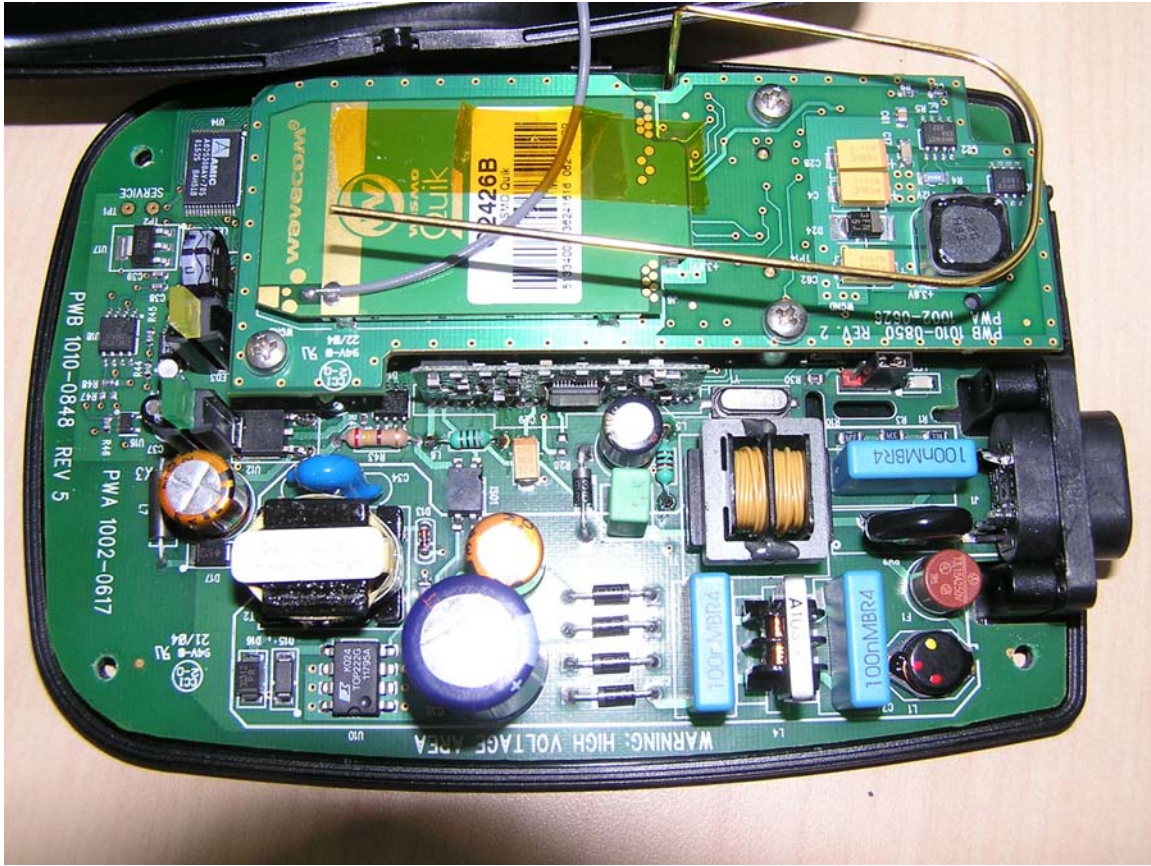
EUT – PCB Top view with GSM module
