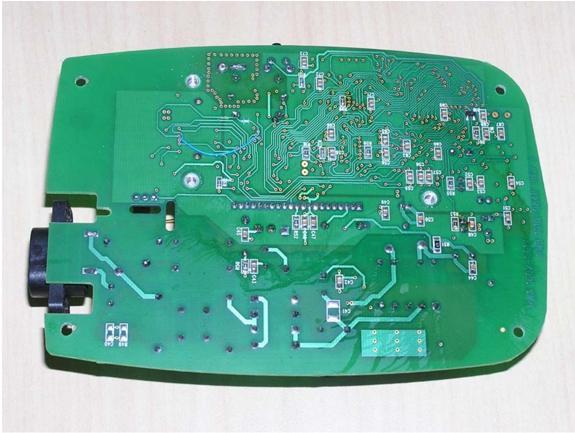
EUT – PCB Bottom view
