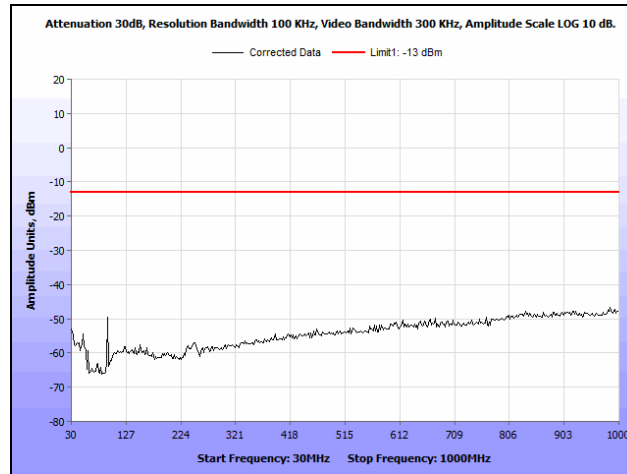
Plot 55. Radiated Spurious Emissions, EGPRS, 1900 MHz Band, Low Channel, 30 MHz – 1 GHz
