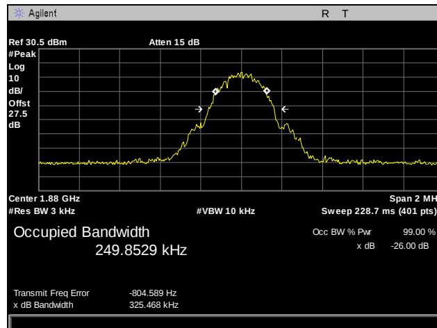
Plot 23. Occupied Bandwidth, GPRS, 1900 MHz Band, Mid Channel
