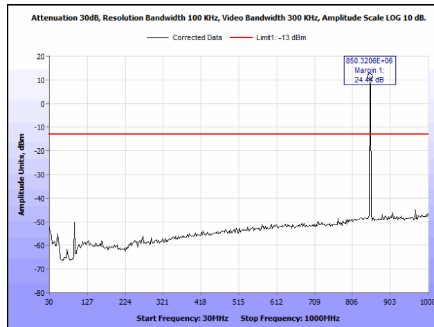
Plot 53. Radiated Spurious Emissions, EGPRS, 850 MHz Band, High Channel, 30 MHz – 1 GHz
