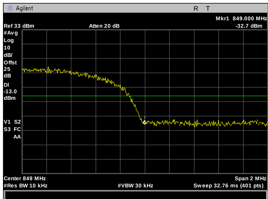
Plot 100. Band Edge Emissions, WCDMA, 850 MHz Band, High Channel
