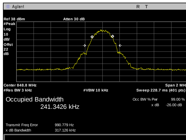
Plot 21. Occupied Bandwidth, GPRS, 850 MHz Band, High Channel
