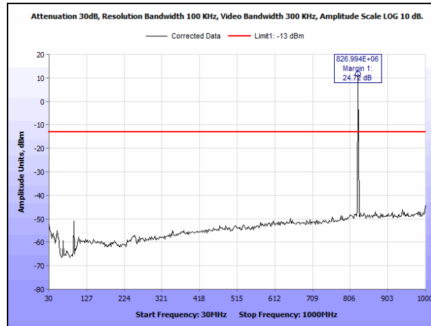
Plot 49. Radiated Spurious Emissions, EGPRS, 850 MHz Band, Low Channel, 30 MHz – 1 GHz
