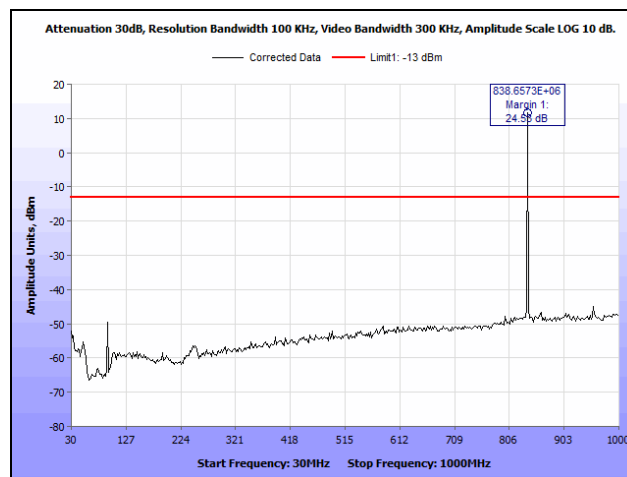
Plot 51. Radiated Spurious Emissions, EGPRS, 850 MHz Band, Mid Channel, 30 MHz – 1 GHz
