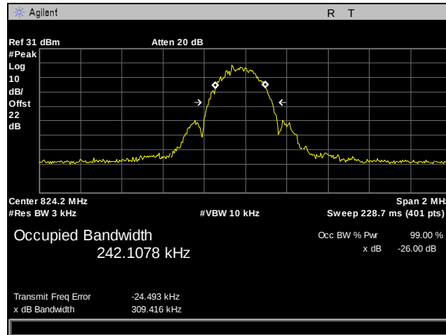
Plot 25. Occupied Bandwidth, EGPRS, 850 MHz Band, Low Channel
