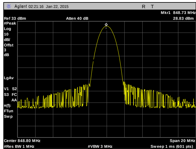
Plot 9. RF Power, EGPRS, 850 MHz Band, High Channel
