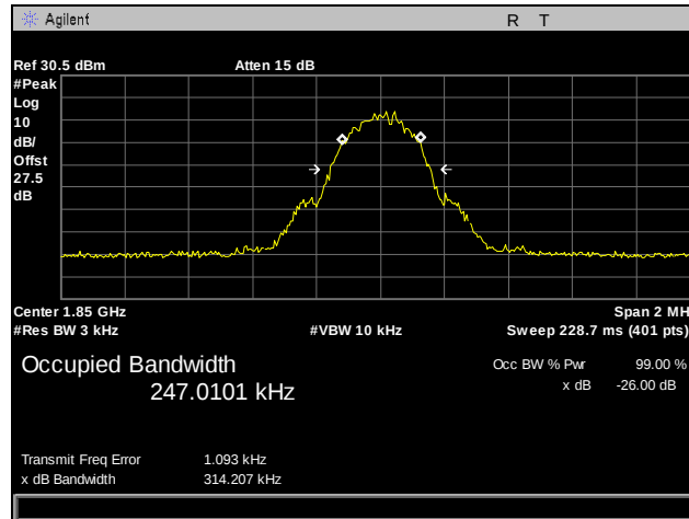
Plot 22. Occupied Bandwidth, GPRS, 1900 MHz Band, Low Channel
