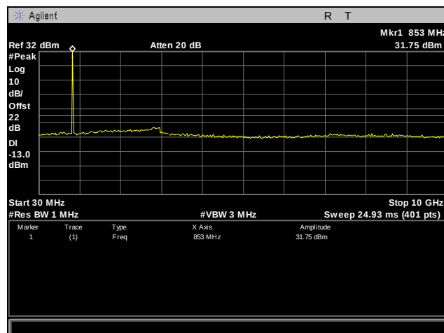
Plot 75. Conducted Spurious Emissions, GPRS, 850 MHz Band, High Channel, 30 MHz – 10 GHz
