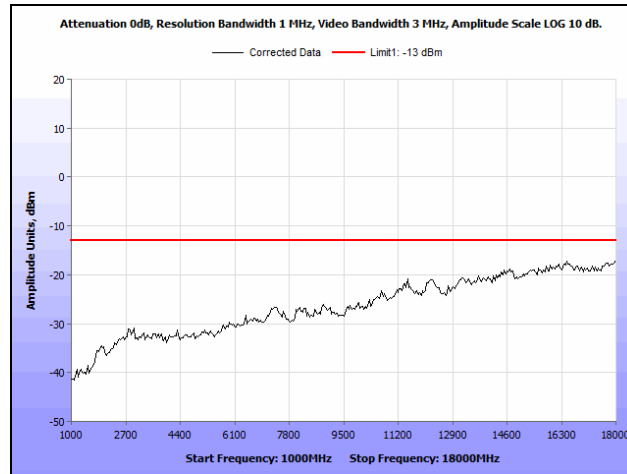
Plot 52. Radiated Spurious Emissions, EGPRS, 850 MHz Band, Mid Channel, 1 GHz – 18 GHz
