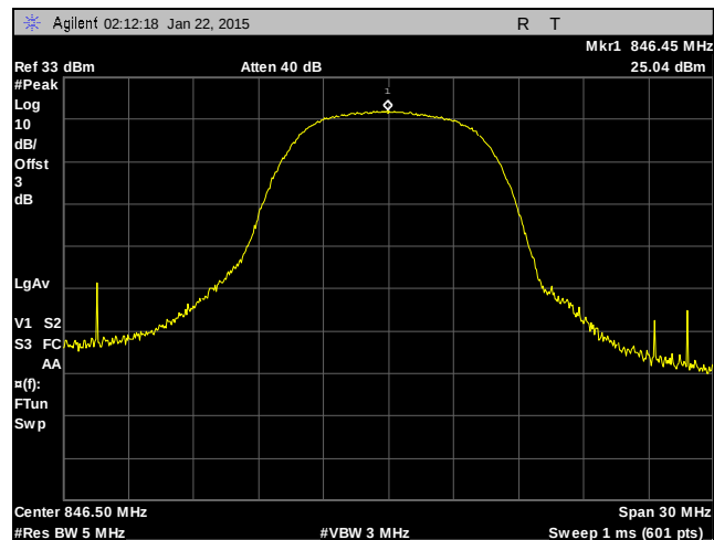
Plot 15. RF Power, WCDMA, 850 MHz Band, High Channel
