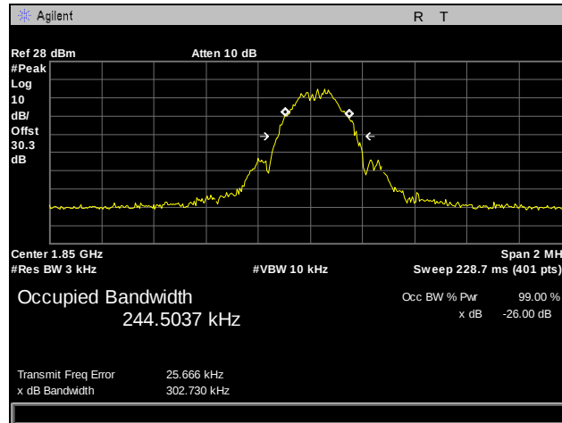
Plot 28. Occupied Bandwidth, EGPRS, 1900 MHz Band, Low Channel
