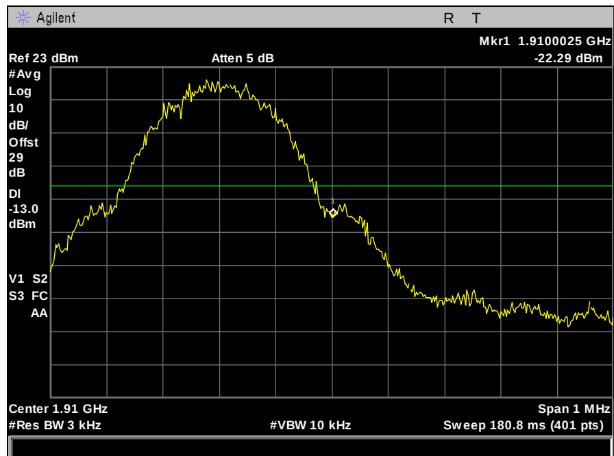
Plot 94. Band Edge Emissions, GPRS, 1900 MHz Band, High Channel
