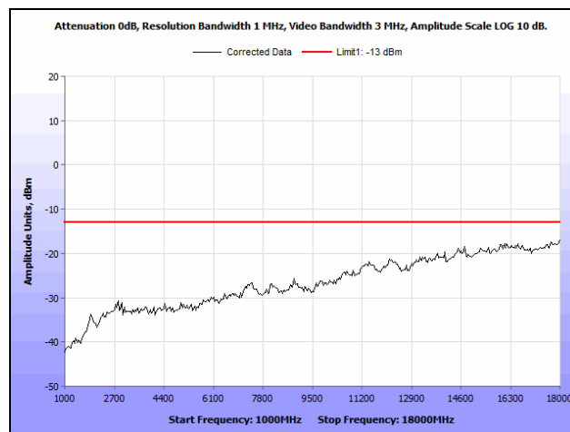
Plot 42. Radiated Spurious Emissions, GPRS, 850 MHz Band, High Channel, 1 GHz – 18 GHz
