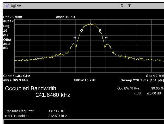
Plot 30. Occupied Bandwidth, EGPRS, 1900 MHz Band, High Channel
