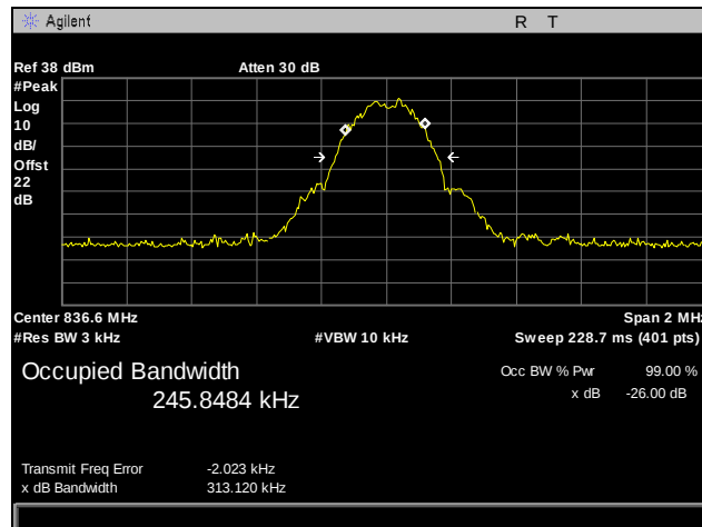
Plot 20. Occupied Bandwidth, GPRS, 850 MHz Band, Mid Channel
