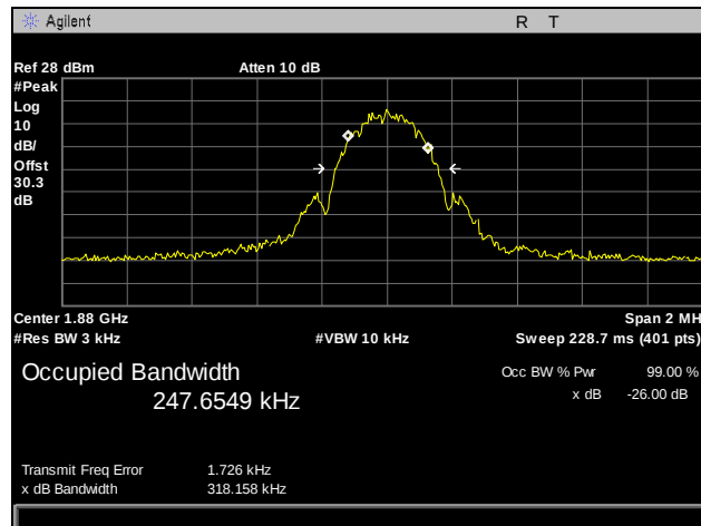
Plot 29. Occupied Bandwidth, EGPRS, 1900 MHz Band, Mid Channel
