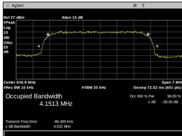
Plot 32. Occupied Bandwidth, WCDMA, 850 MHz Band, Mid Channel
