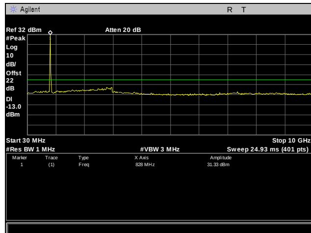
Plot 74. Conducted Spurious Emissions, GPRS, 850 MHz Band, Mid Channel, 30 MHz – 10 GHz
