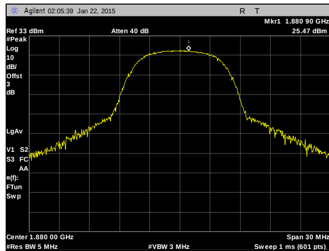
Plot 17. RF Power, WCDMA, 1900 MHz Band, Mid Channel
