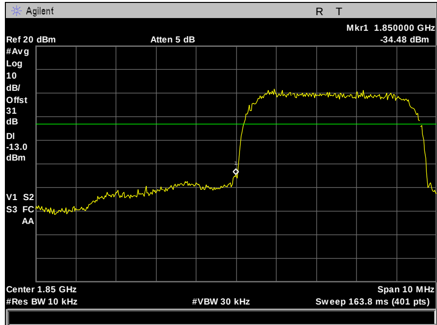
Plot 101. Band Edge Emissions, WCDMA, 1900 MHz Band, Low Channel
