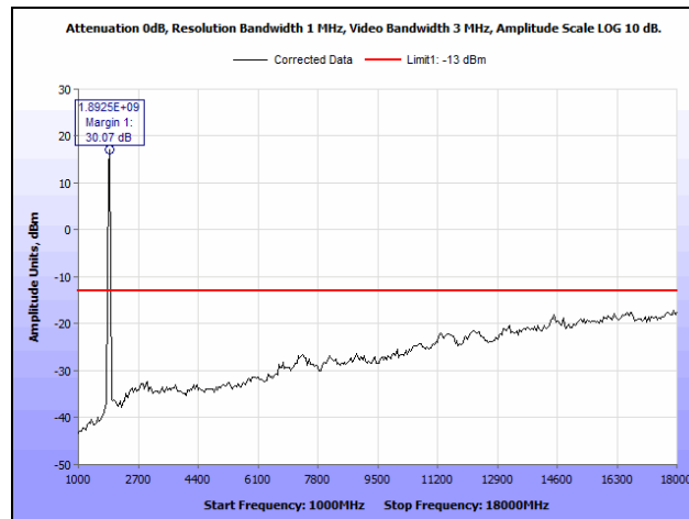
Plot 56. Radiated Spurious Emissions, EGPRS, 1900 MHz Band, Low Channel, 1 GHz – 18 GHz
