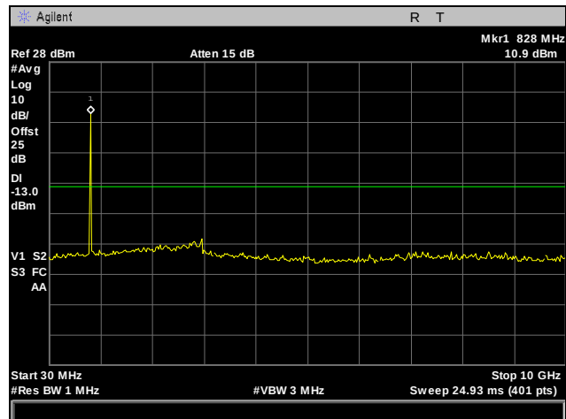
Plot 86. Conducted Spurious Emissions, WCDMA, 850 MHz Band, Mid Channel, 30 MHz – 10 GHz
