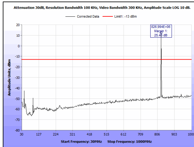
Plot 37. Radiated Spurious Emissions, GPRS, 850 MHz Band, Low Channel, 30 MHz – 1 GHz
