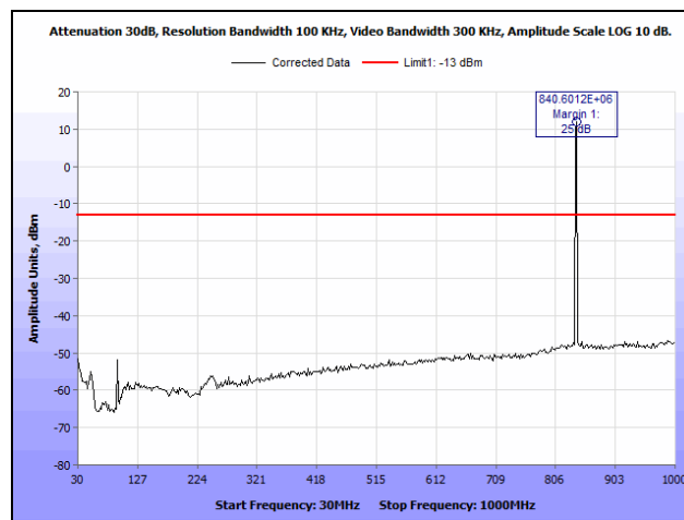
Plot 63. Radiated Spurious Emissions, WCDMA, 850 MHz Band, Mid Channel, 30 MHz – 1 GHz
