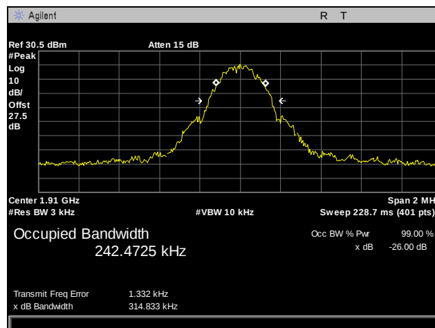
Plot 24. Occupied Bandwidth, GPRS, 1900 MHz Band, High Channel
