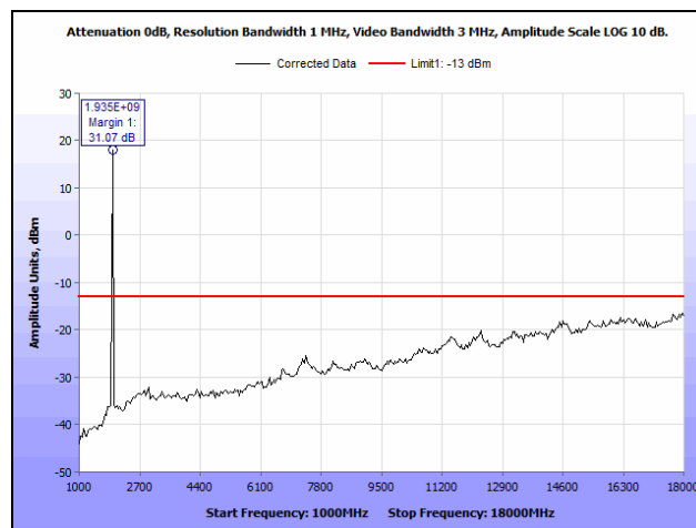
Plot 60. Radiated Spurious Emissions, EGPRS, 1900 MHz Band, High Channel, 1 GHz – 18 GHz
