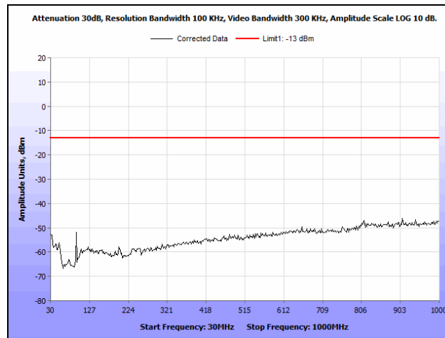
Plot 67. Radiated Spurious Emissions, WCDMA, 1900 MHz Band, Low Channel, 30 MHz – 1 GHz
