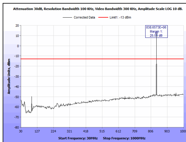
Plot 39. Radiated Spurious Emissions, GPRS, 850 MHz Band, Mid Channel, 30 MHz – 1 GHz
