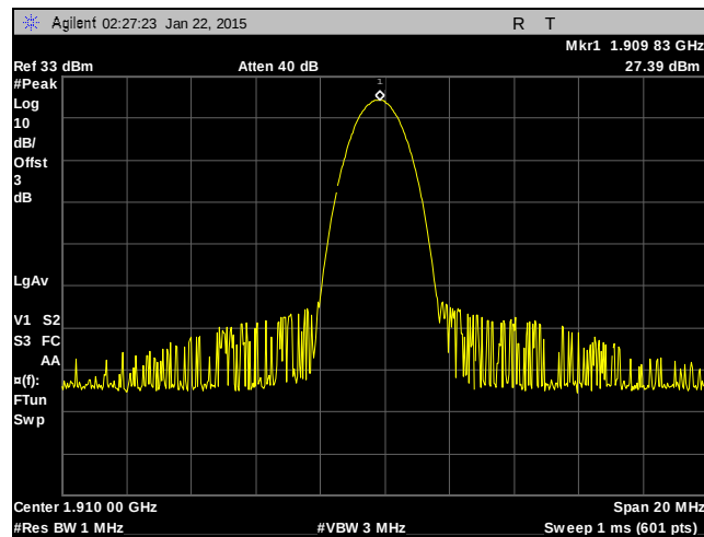
Plot 12. RF Power, EGPRS, 1900 MHz Band, High Channel
