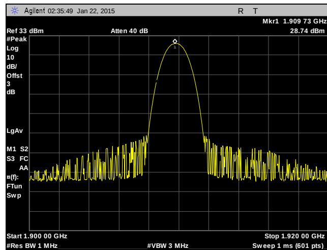
Plot 6. RF Power, GPRS, 1900 MHz Band, High Channel
