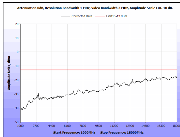
Plot 62. Radiated Spurious Emissions, WCDMA, 850 MHz Band, Low Channel, 1 GHz – 18 GHz
