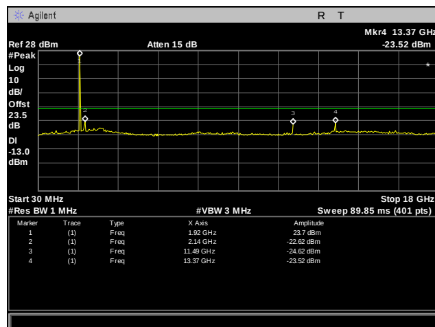
Plot 84. Conducted Spurious Emissions, EGPRS, 1900 MHz Band, High Channel, 30 MHz – 18 GHz
