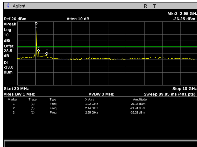
Plot 83. Conducted Spurious Emissions, EGPRS, 1900 MHz Band, Mid Channel, 30 MHz – 18 GHz
