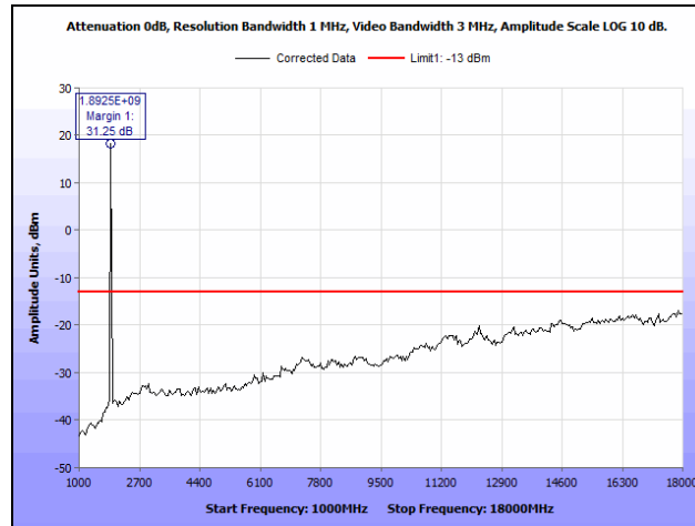
Plot 58. Radiated Spurious Emissions, EGPRS, 1900 MHz Band, Mid Channel, 1 GHz – 18 GHz
