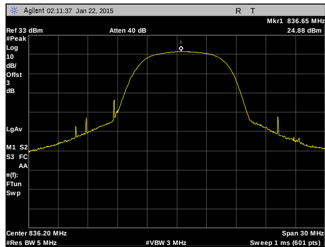
Plot 14. RF Power, WCDMA, 850 MHz Band, Mid Channel
