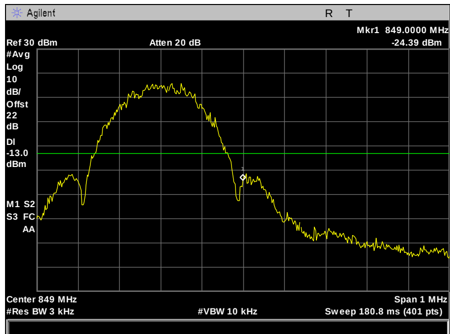
Plot 96. Band Edge Emissions, EGPRS, 850 MHz Band, High Channel
