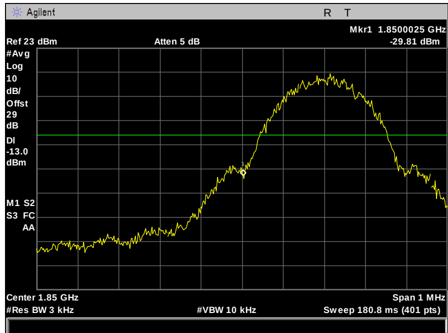
Plot 93. Band Edge Emissions, GPRS, 1900 MHz Band, Low Channel
