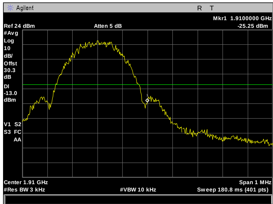
Plot 98. Band Edge Emissions, EGPRS, 1900 MHz Band, High Channel
