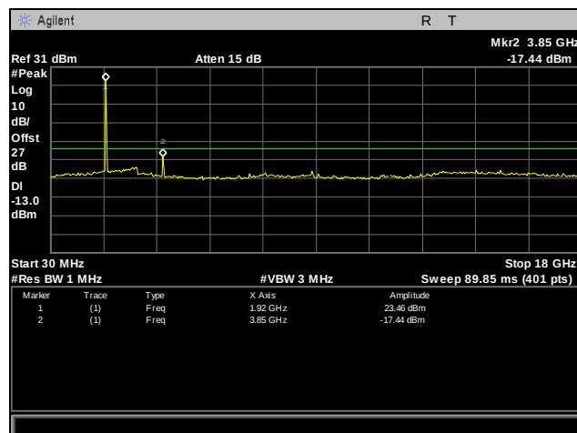
Plot 90. Conducted Spurious Emissions, WCDMA, 1900 MHz Band, High Channel, 30 MHz – 18 GHz
