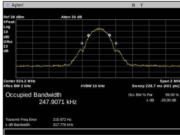
Plot 19. Occupied Bandwidth, GPRS, 850 MHz Band, Low Channel
