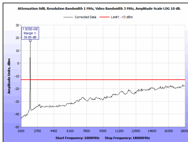
Plot 48. Radiated Spurious Emissions, GPRS, 1900 MHz Band, High Channel, 1 GHz – 18 GHz
