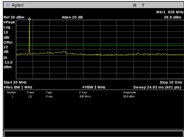
Plot 79. Conducted Spurious Emissions, EGPRS, 850 MHz Band, Low Channel, 30 MHz – 10 GHz
