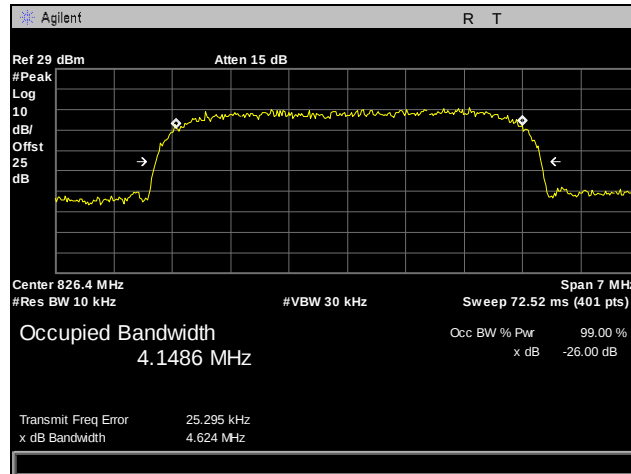
Plot 31. Occupied Bandwidth, WCDMA, 850 MHz Band, Low Channel
