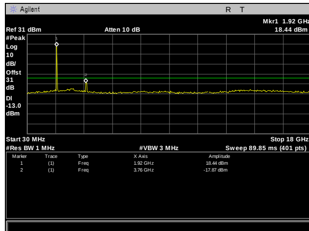
Plot 89. Conducted Spurious Emissions, WCDMA, 1900 MHz Band, Mid Channel, 30 MHz – 18 GHz
