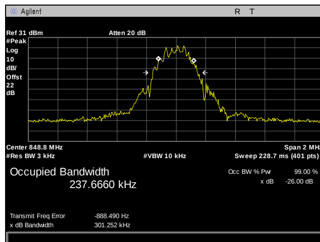
Plot 27. Occupied Bandwidth, EGPRS, 850 MHz Band, High Channel
