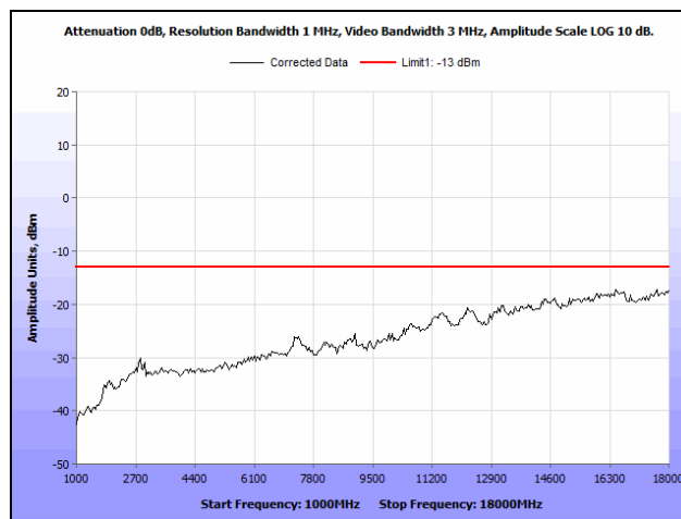
Plot 38. Radiated Spurious Emissions, GPRS, 850 MHz Band, Low Channel, 1 GHz – 18 GHz
