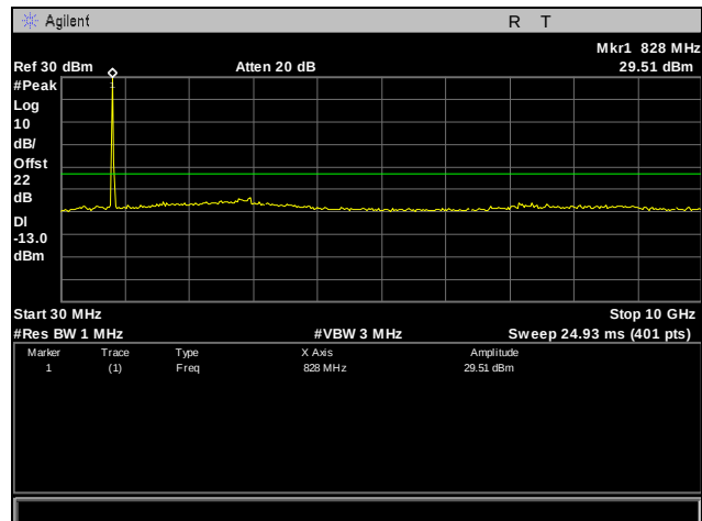
Plot 80. Conducted Spurious Emissions, EGPRS, 850 MHz Band, Mid Channel, 30 MHz – 10 GHz
