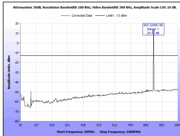
Plot 41. Radiated Spurious Emissions, GPRS, 850 MHz Band, High Channel, 30 MHz – 1 GHz
