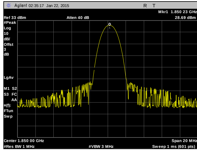
Plot 4. RF Power, GPRS, 1900 MHz Band, Low Channel
