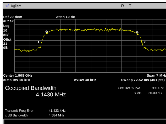
Plot 36. Occupied Bandwidth, WCDMA, 1900 MHz Band, High Channel
