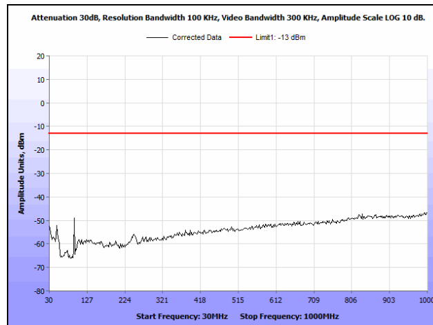
Plot 59. Radiated Spurious Emissions, EGPRS, 1900 MHz Band, High Channel, 30 MHz – 1 GHz
