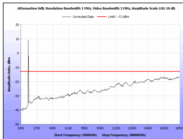
Plot 72. Radiated Spurious Emissions, WCDMA, 1900 MHz Band, High Channel, 1 GHz – 18 GHz
