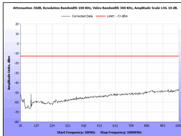
Plot 71. Radiated Spurious Emissions, WCDMA, 1900 MHz Band, High Channel, 30 MHz – 1 GHz
