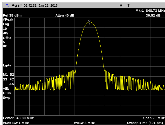
Plot 3. RF Power, GPRS, 850 MHz Band, High Channel
