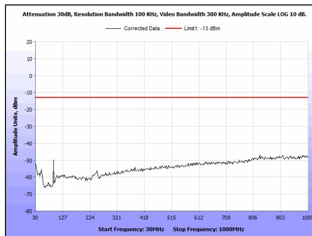
Plot 57. Radiated Spurious Emissions, EGPRS, 1900 MHz Band, Mid Channel, 30 MHz – 1 GHz
