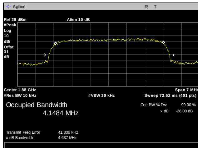
Plot 35. Occupied Bandwidth, WCDMA, 1900 MHz Band, Mid Channel
