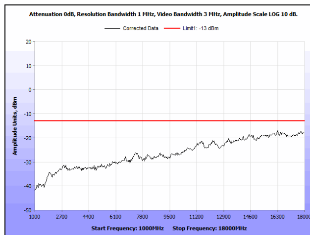
Plot 66. Radiated Spurious Emissions, WCDMA, 850 MHz Band, High Channel, 1 GHz – 18 GHz
