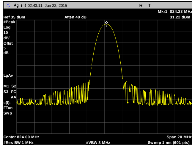
Plot 1. RF Power, GPRS, 850 MHz Band, Low Channel
