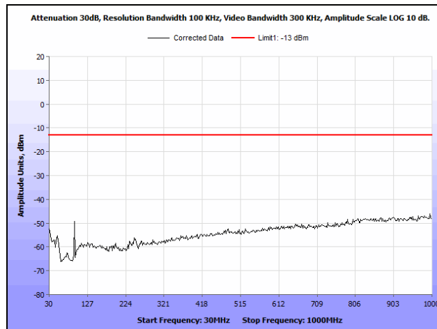
Plot 47. Radiated Spurious Emissions, GPRS, 1900 MHz Band, High Channel, 30 MHz – 1 GHz
