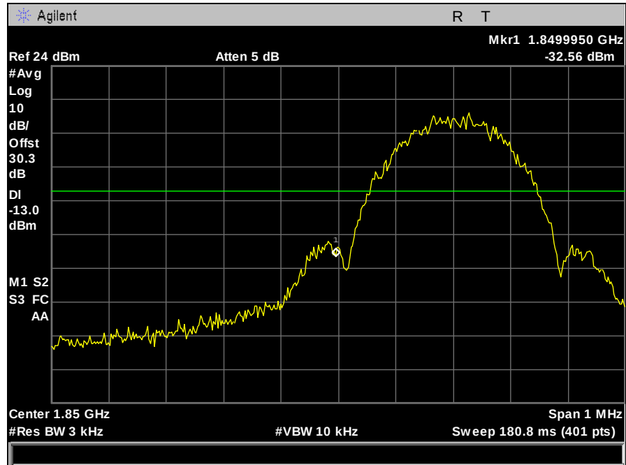
Plot 97. Band Edge Emissions, EGPRS, 1900 MHz Band, Low Channel
