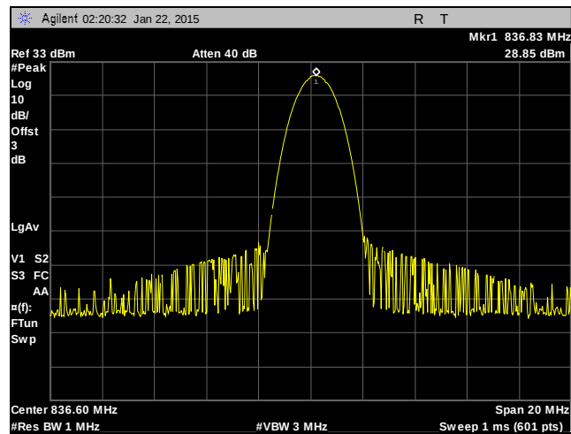
Plot 8. RF Power, EGPRS, 850 MHz Band, Mid Channel
