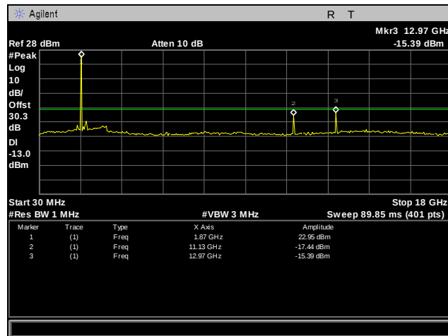
Plot 82. Conducted Spurious Emissions, EGPRS, 1900 MHz Band, Low Channel, 30 MHz – 18 GHz
