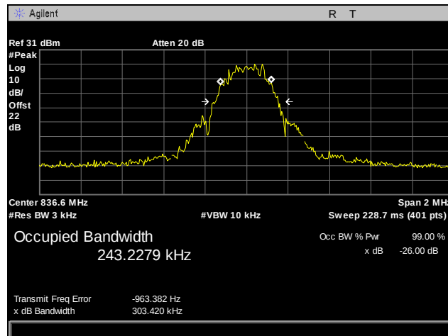
Plot 26. Occupied Bandwidth, EGPRS, 850 MHz Band, Mid Channel
