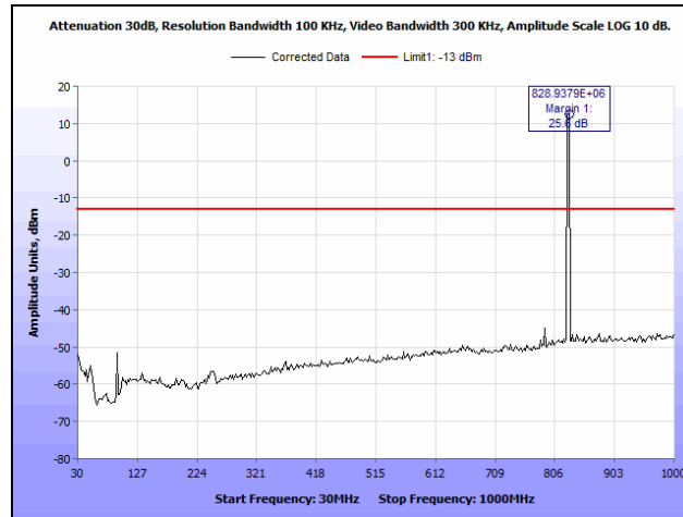
Plot 61. Radiated Spurious Emissions, WCDMA, 850 MHz Band, Low Channel, 30 MHz – 1 GHz
