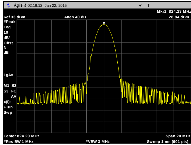
Plot 7. RF Power, EGPRS, 850 MHz Band, Low Channel
