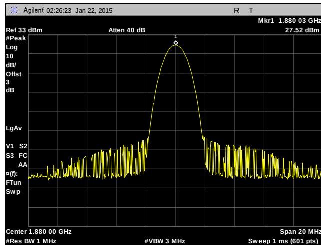
Plot 11. RF Power, EGPRS, 1900 MHz Band, Mid Channel
