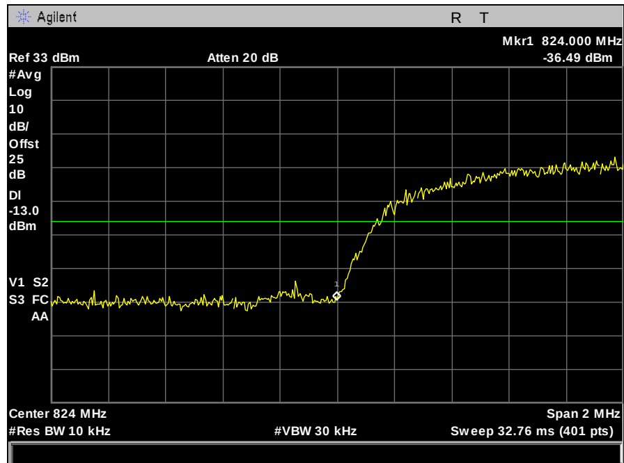
Plot 99. Band Edge Emissions, WCDMA, 850 MHz Band, Low Channel
