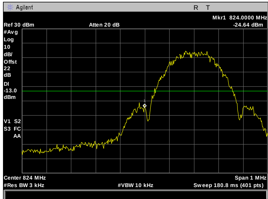
Plot 95. Band Edge Emissions, EGPRS, 850 MHz Band, Low Channel
