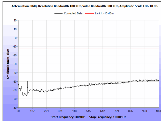
Plot 43. Radiated Spurious Emissions, GPRS, 1900 MHz Band, Low Channel, 30 MHz – 1 GHz
