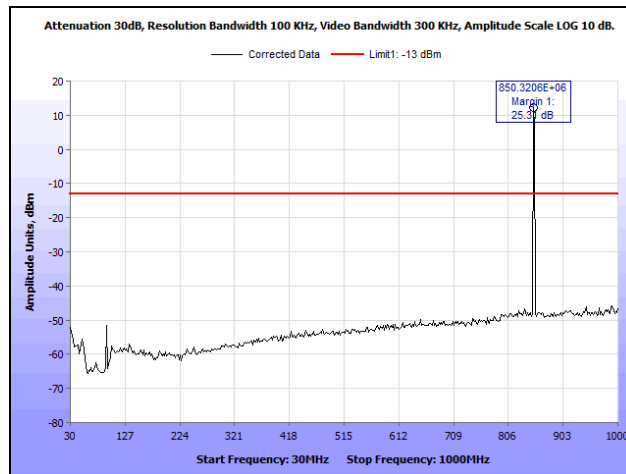
Plot 65. Radiated Spurious Emissions, WCDMA, 850 MHz Band, High Channel, 30 MHz – 1 GHz
