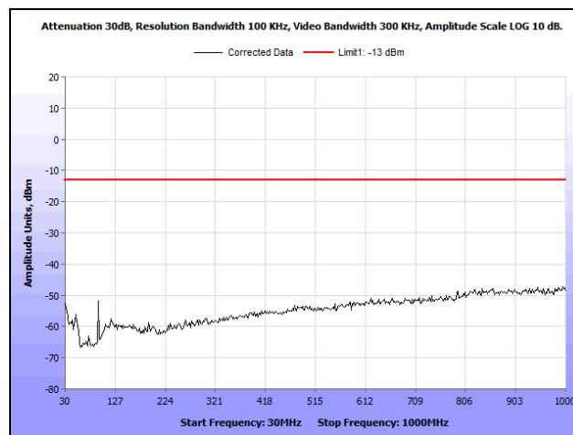
Plot 69. Radiated Spurious Emissions, WCDMA, 1900 MHz Band, Mid Channel, 30 MHz – 1 GHz
