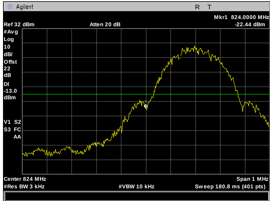
Plot 91. Band Edge Emissions, GPRS, 850 MHz Band, Low Channel
