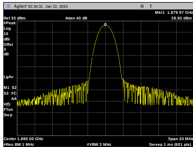
Plot 5. RF Power, GPRS, 1900 MHz Band, Mid Channel
