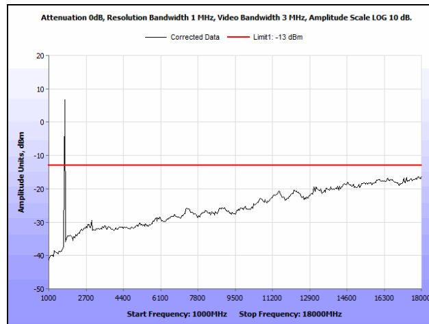
Plot 68. Radiated Spurious Emissions, WCDMA, 1900 MHz Band, Low Channel, 1 GHz – 18 GHz
