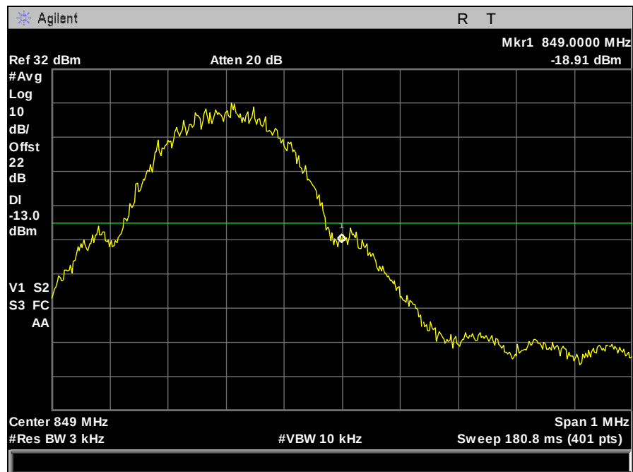
Plot 92. Band Edge Emissions, GPRS, 850 MHz Band, High Channel
