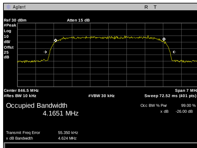
Plot 33. Occupied Bandwidth, WCDMA, 850 MHz Band, High Channel
