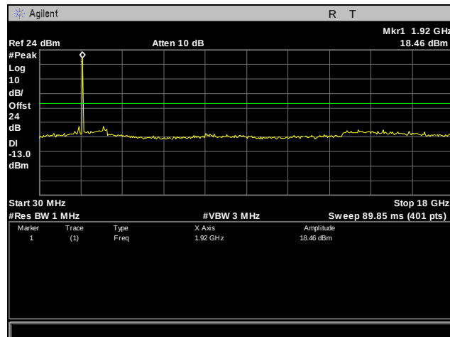
Plot 77. Conducted Spurious Emissions, GPRS, 1900 MHz Band, Mid Channel, 30 MHz – 18 GHz
