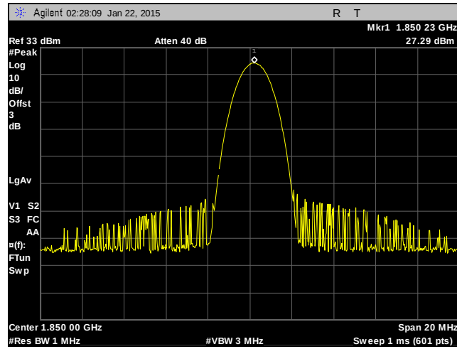
Plot 10. RF Power, EGPRS, 1900 MHz Band, Low Channel
