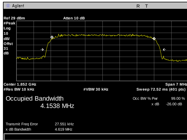
Plot 34. Occupied Bandwidth, WCDMA, 1900 MHz Band, Low Channel
