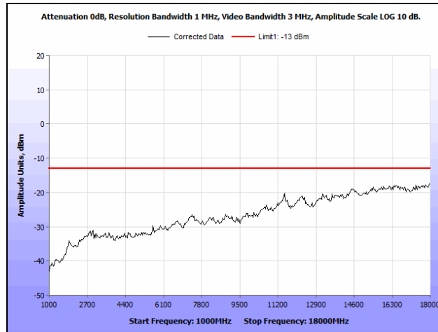
Plot 64. Radiated Spurious Emissions, WCDMA, 850 MHz Band, Mid Channel, 1 GHz – 18 GHz
