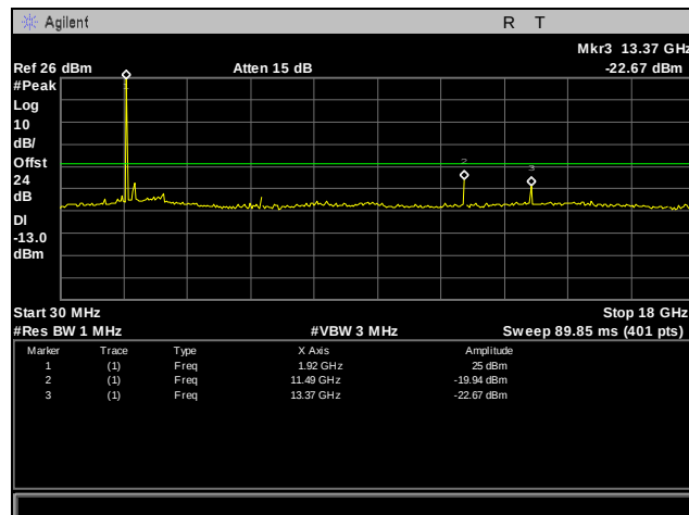
Plot 78. Conducted Spurious Emissions, GPRS, 1900 MHz Band, High Channel, 30 MHz – 18 GHz
