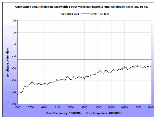
Plot 50. Radiated Spurious Emissions, EGPRS, 850 MHz Band, Low Channel, 1 GHz – 18 GHz
