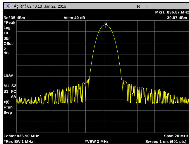
Plot 2. RF Power, GPRS, 850 MHz Band, Mid Channel
