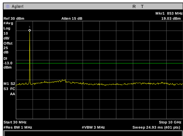
Plot 87. Conducted Spurious Emissions, WCDMA, 850 MHz Band, High Channel, 30 MHz – 10 GHz
