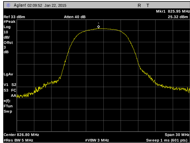
Plot 13. RF Power, WCDMA, 850 MHz Band, Low Channel
