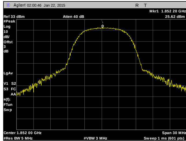
Plot 16. RF Power, WCDMA, 1900 MHz Band, Low Channel
