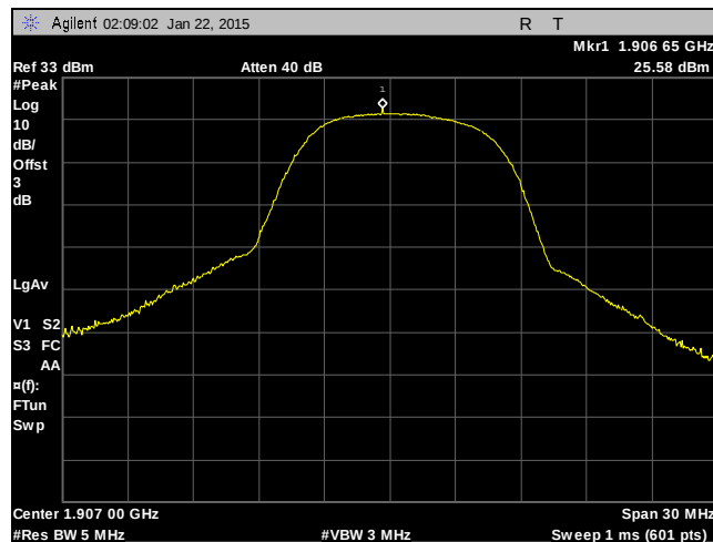
Plot 18. RF Power, WCDMA, 1900 MHz Band, High Channel
