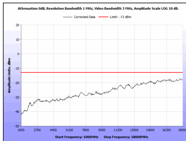
Plot 54. Radiated Spurious Emissions, EGPRS, 850 MHz Band, High Channel, 1 GHz – 18 GHz
