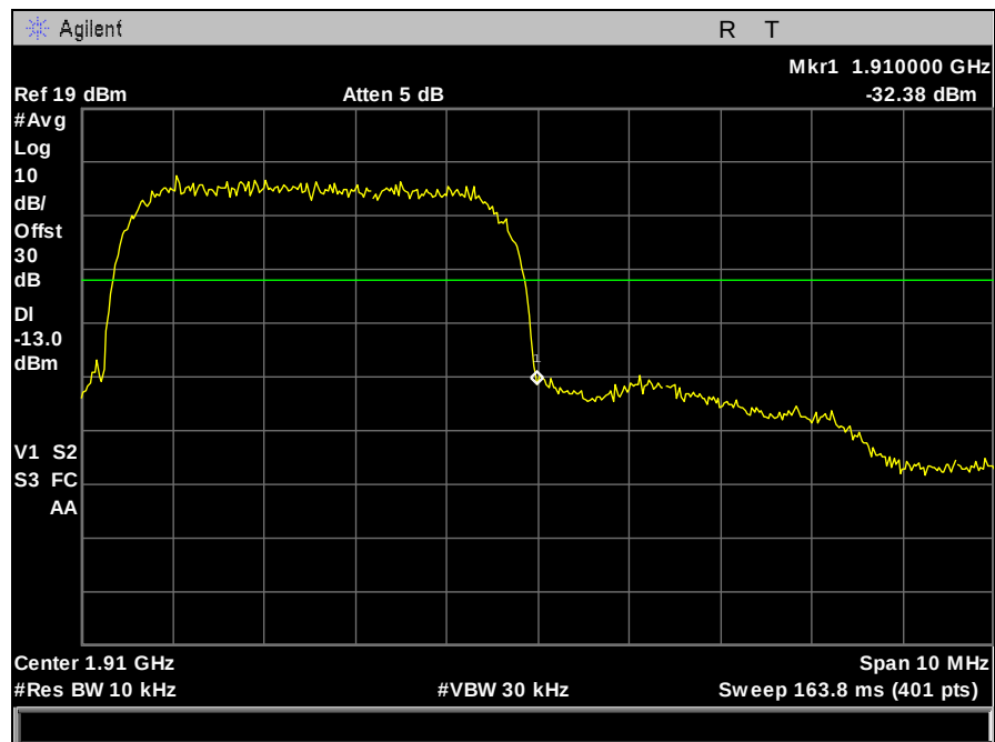
Plot 102. Band Edge Emissions, WCDMA, 1900 MHz Band, High Channel
