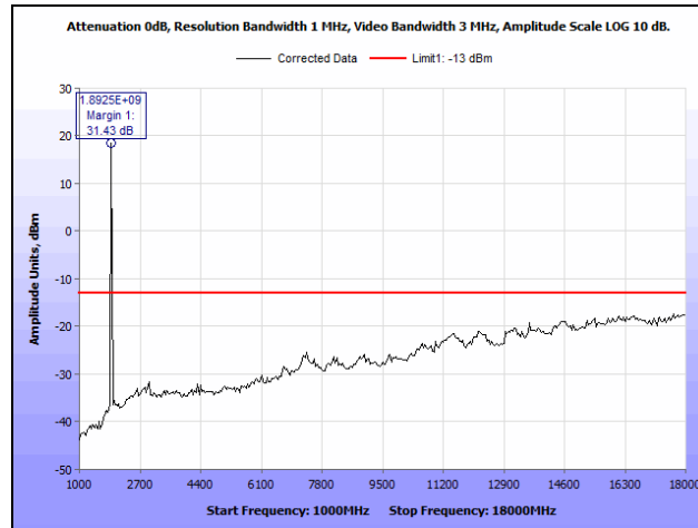
Plot 46. Radiated Spurious Emissions, GPRS, 1900 MHz Band, Mid Channel, 1 GHz – 18 GHz
