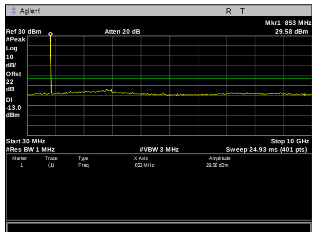
Plot 81. Conducted Spurious Emissions, EGPRS, 850 MHz Band, High Channel, 30 MHz – 10 GHz
