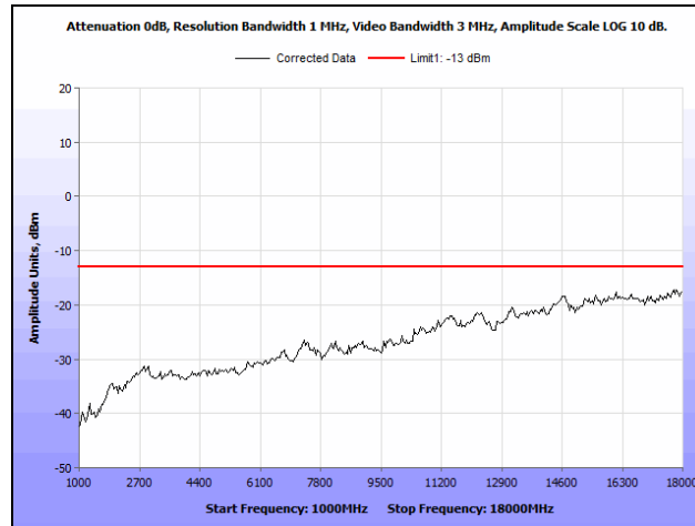
Plot 40. Radiated Spurious Emissions, GPRS, 850 MHz Band, Mid Channel, 1 GHz – 18 GHz
