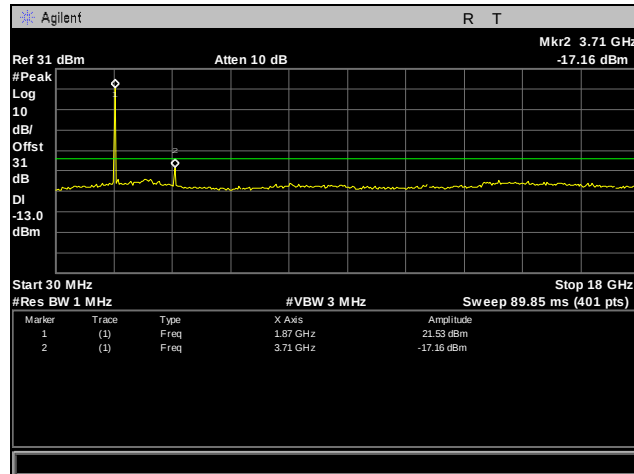
Plot 88. Conducted Spurious Emissions, WCDMA, 1900 MHz Band, Low Channel, 30 MHz – 18 GHz
