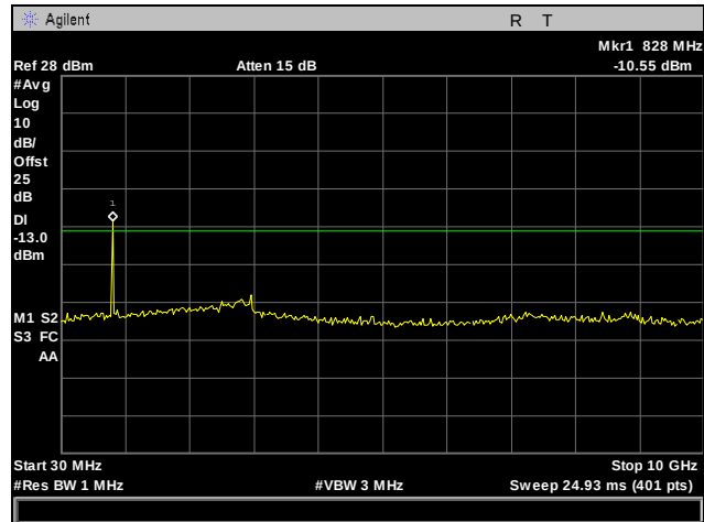
Plot 85. Conducted Spurious Emissions, WCDMA, 850 MHz Band, Low Channel, 30 MHz – 10 GHz
