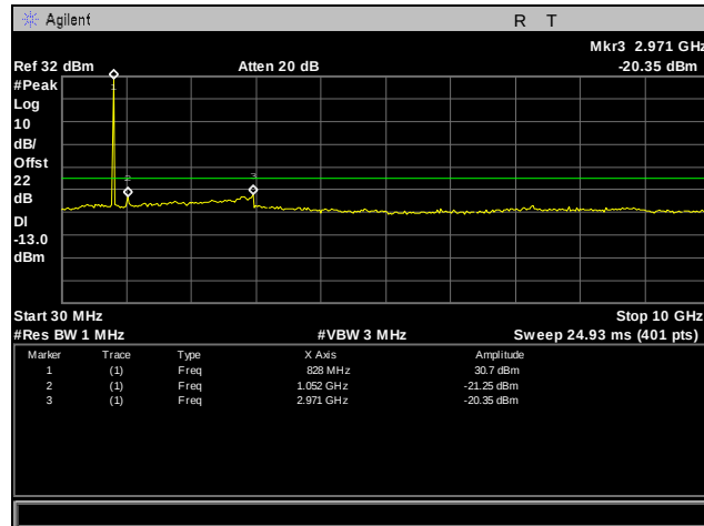
Plot 73. Conducted Spurious Emissions, GPRS, 850 MHz Band, Low Channel, 30 MHz – 10 GHz
