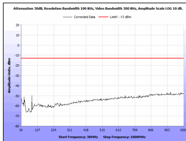
Plot 45. Radiated Spurious Emissions, GPRS, 1900 MHz Band, Mid Channel, 30 MHz – 1 GHz
