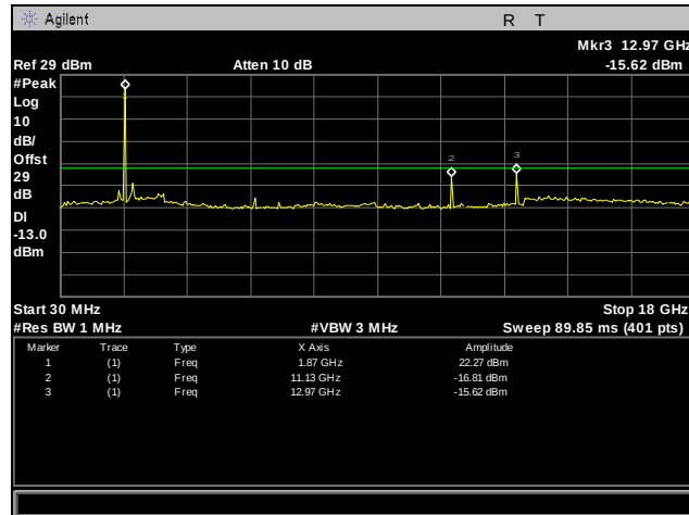
Plot 76. Conducted Spurious Emissions, GPRS, 1900 MHz Band, Low Channel, 30 MHz – 18 GHz
