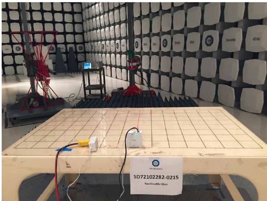
Radiated Emissions Test Setup (above 1GHz)
