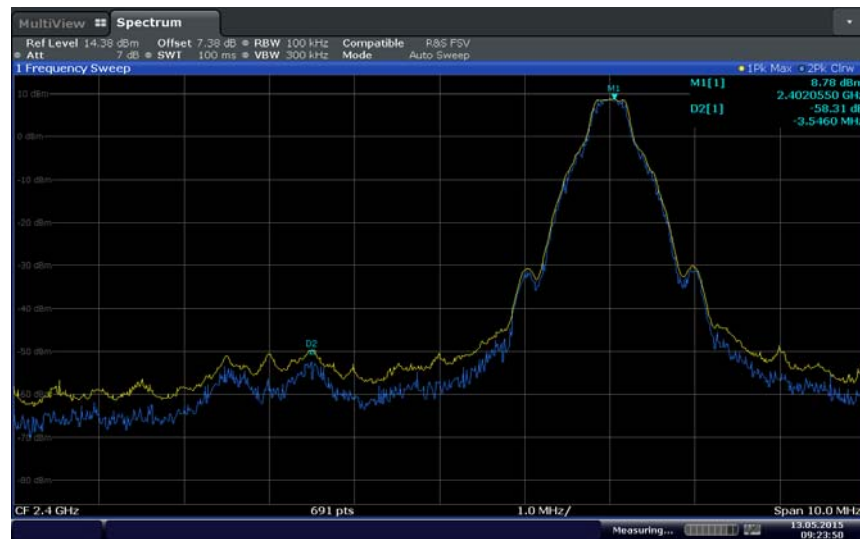
Non-hopping lower band edge (GFSK)
