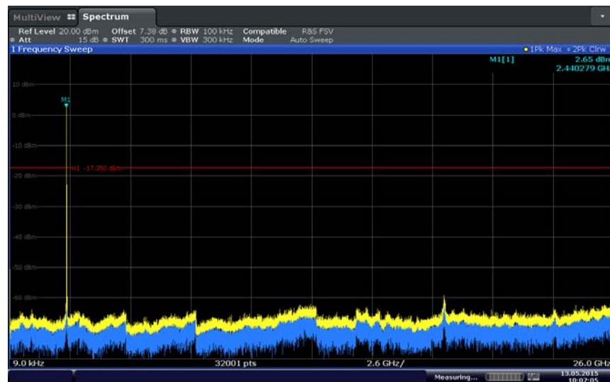
Mid Channel (8DPSK)
