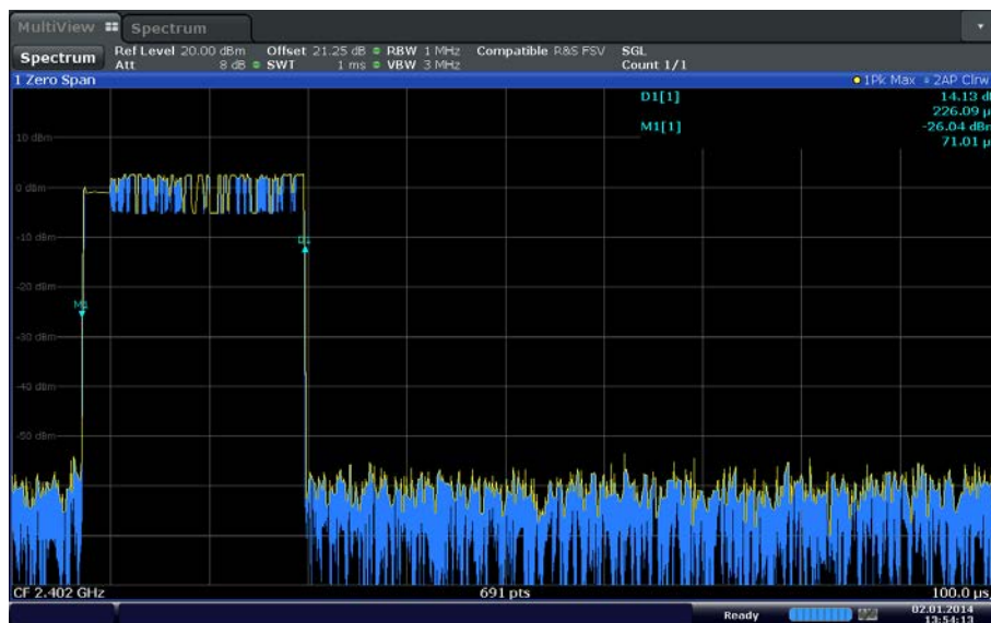
GFSK width of single pulse (0.226ms)
