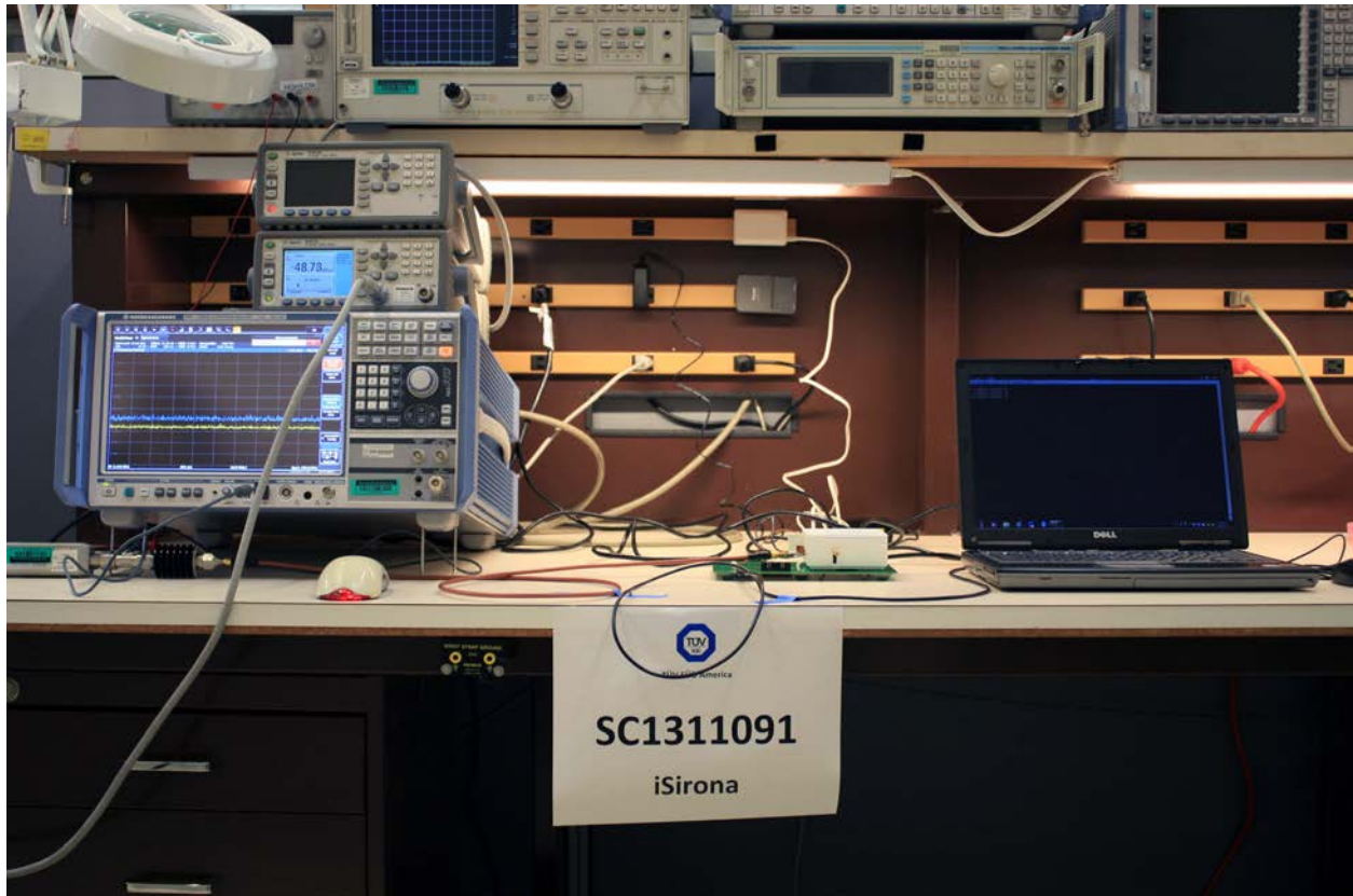
Conducted Port Test Setup
