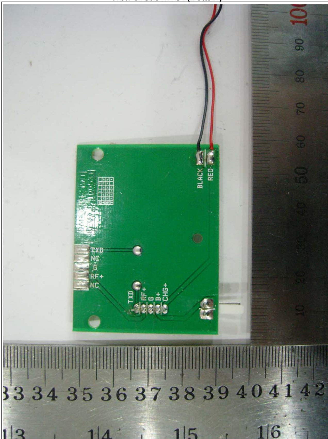
View of Sub 1 PCB(Bottom)
