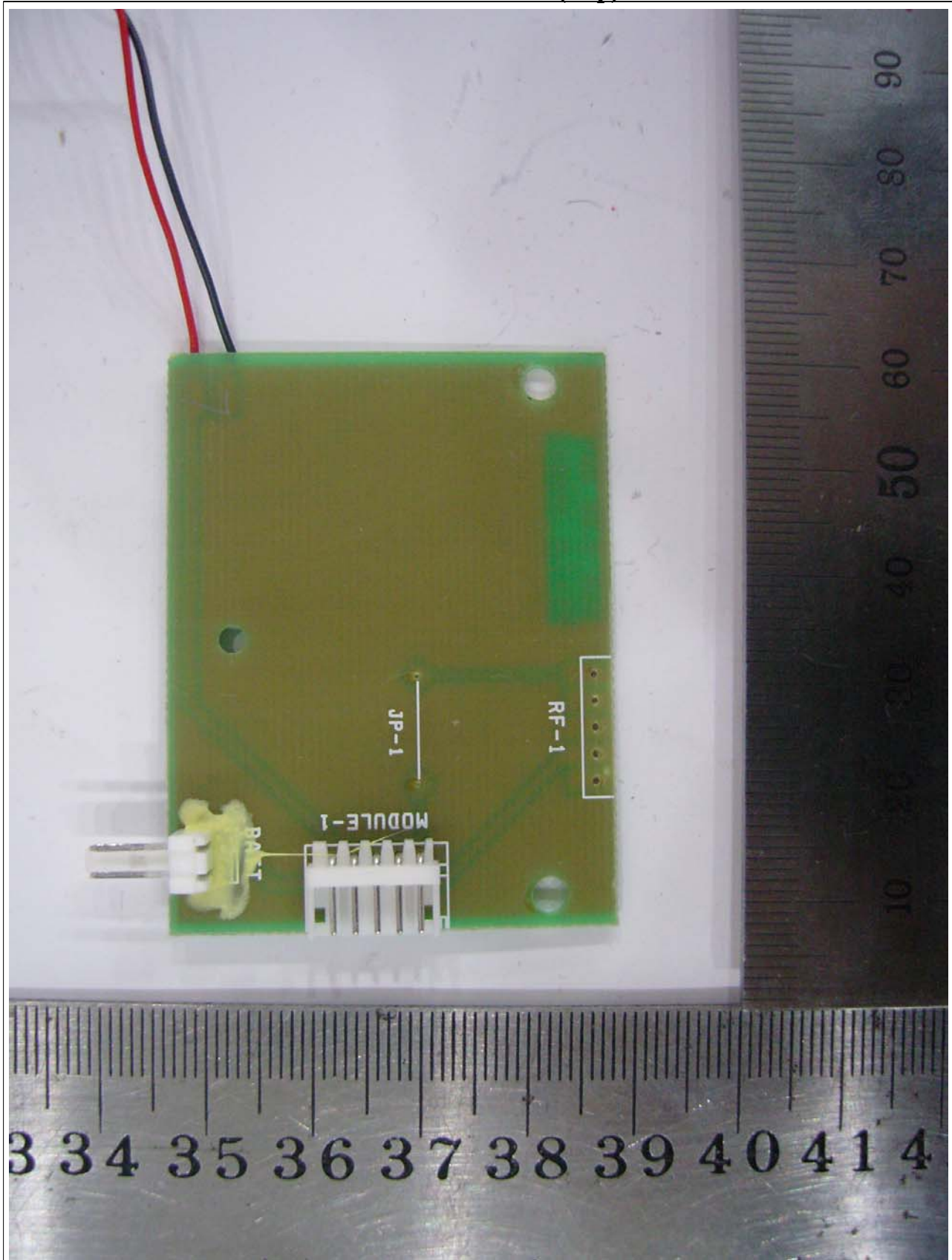
View of Sub 1 PCB(Top)
