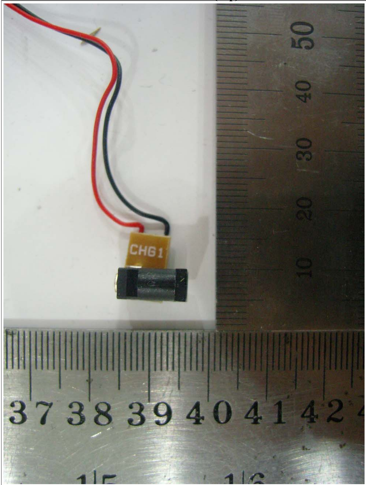
View of Sub 2 PCB(Top)
