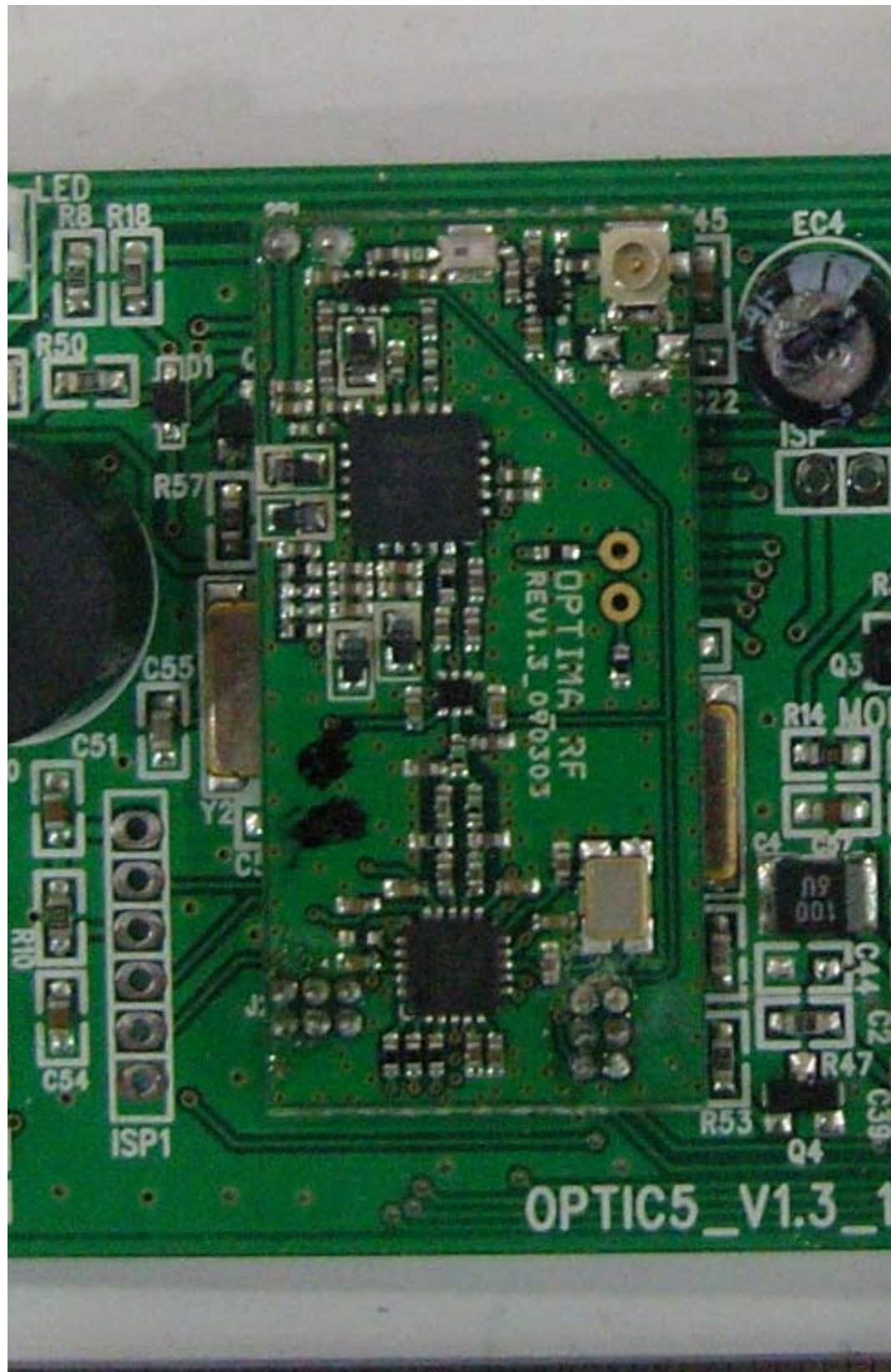
View of Module (Top)
