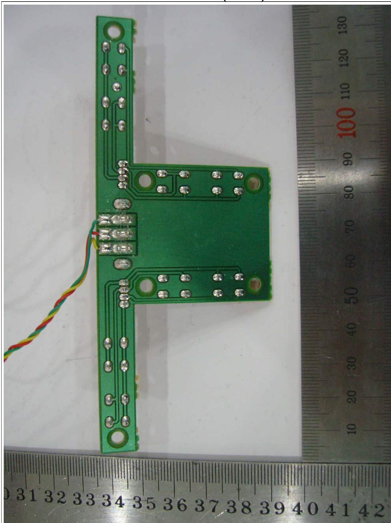
View of Sub 5 PCB(Bottom)
