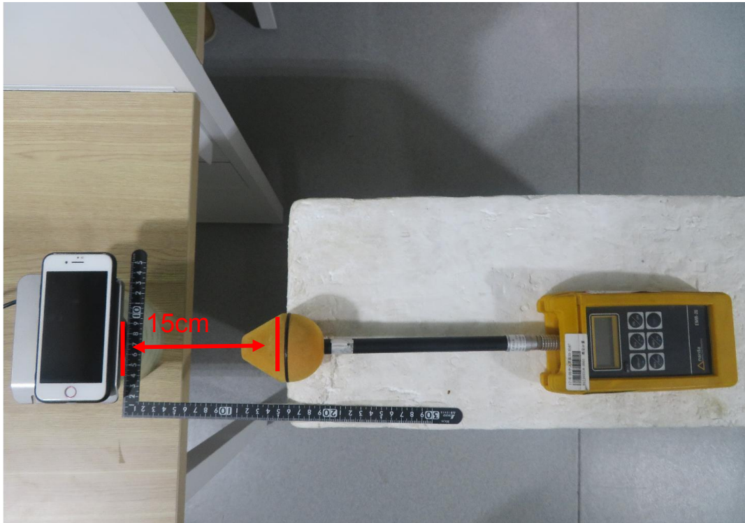
Description: RF Exposure Test Setup (Left Side: 15cm)
