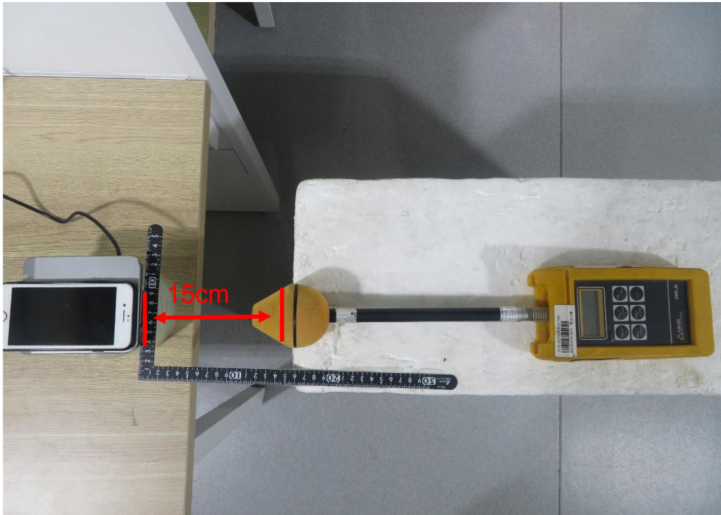
Description: RF Exposure Test Setup (Rear Side: 15cm)
