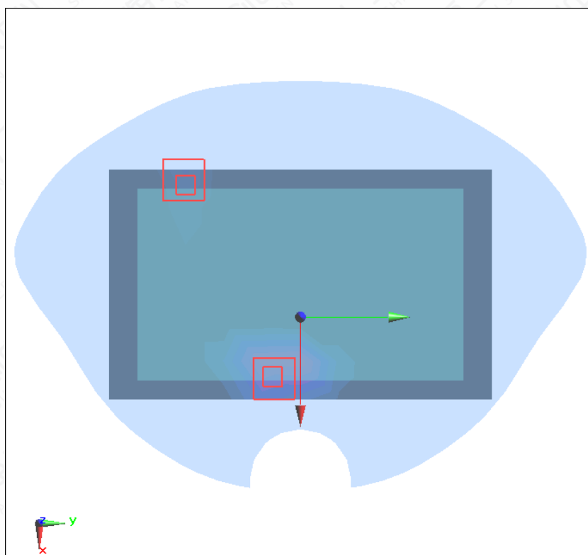
Figure A.1-18 WCDMA Band IV + Wi-Fi 5G Back 0mm
