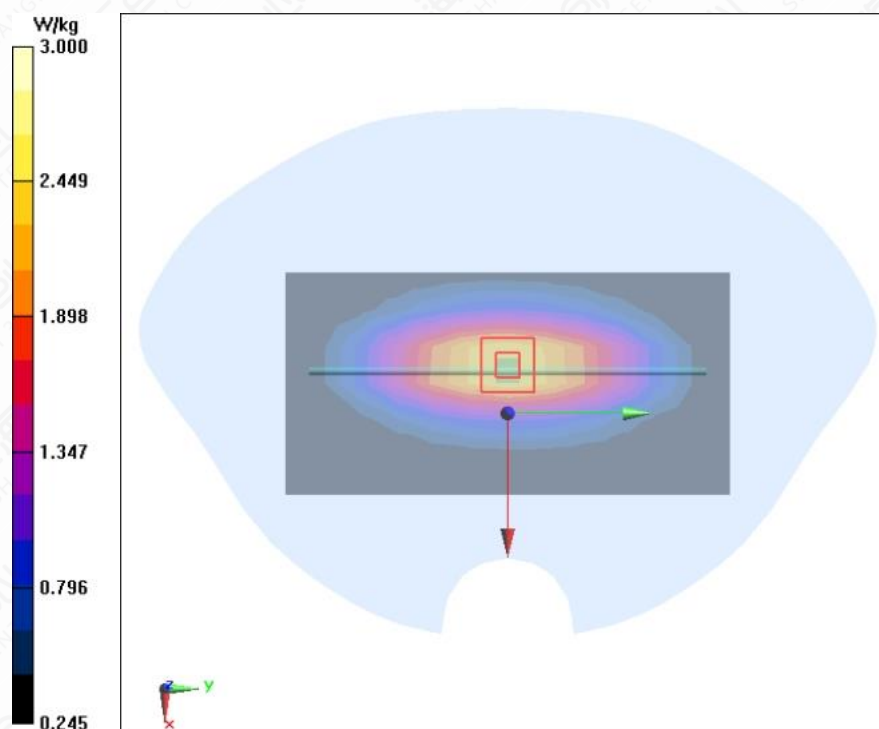
Figure A.2-2 System Check 750MHz
