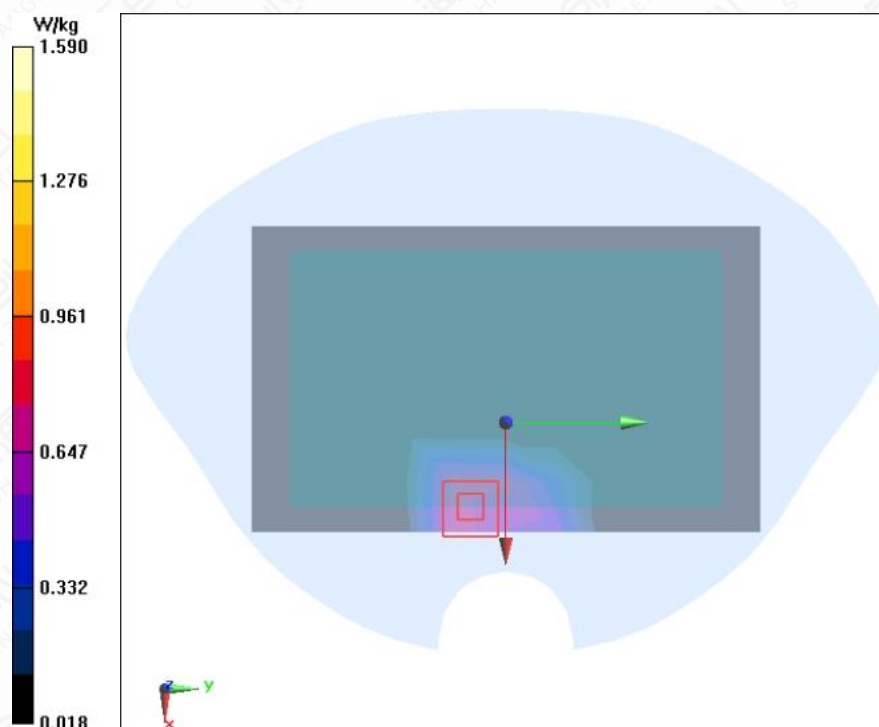
Figure A.1-4 LTE B2 20MHz 1RB 50offset Back Side Mode Middle 0mm
