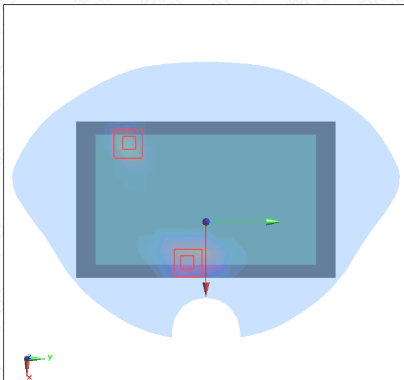
Figure A.1-17 WCDMA Band IV + Wi-Fi 2.4G Back 0mm
