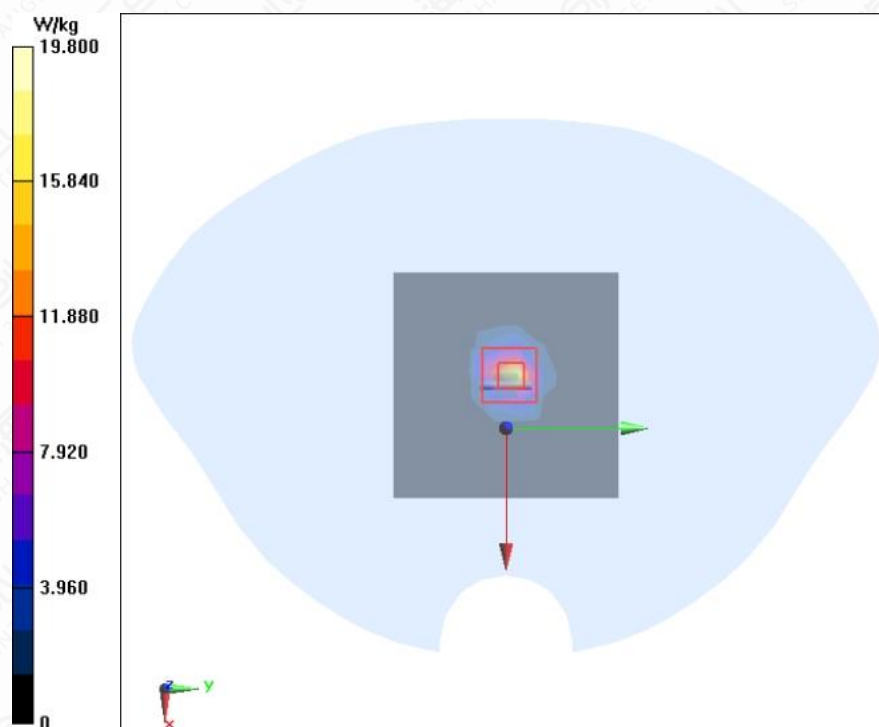
Figure A.2-7 System Check 5200MHz
