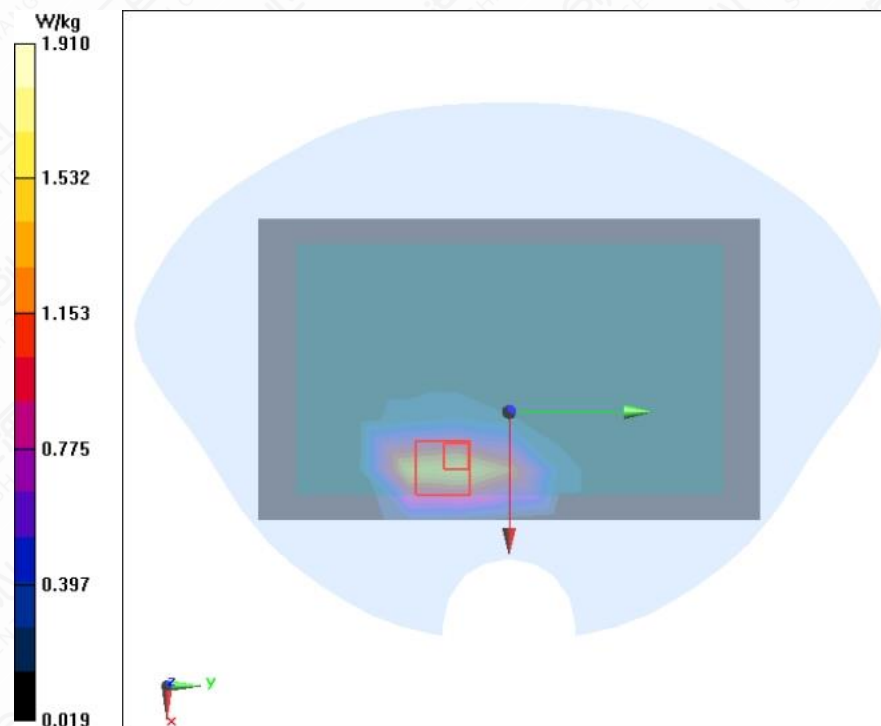
Figure A.1-7 LTE B13 10MHz 1RB 25offset Back Side Mode Middle 0mm
