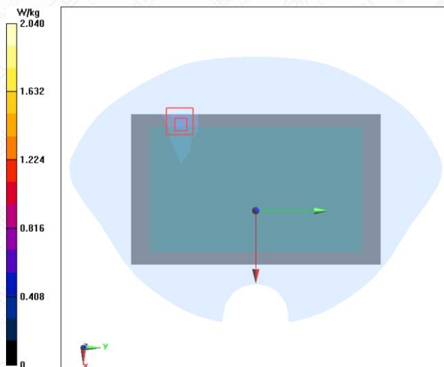
Figure A.1-12 Wi-Fi5G U-NII-1 802.11a Back Side Mode High 0mm
