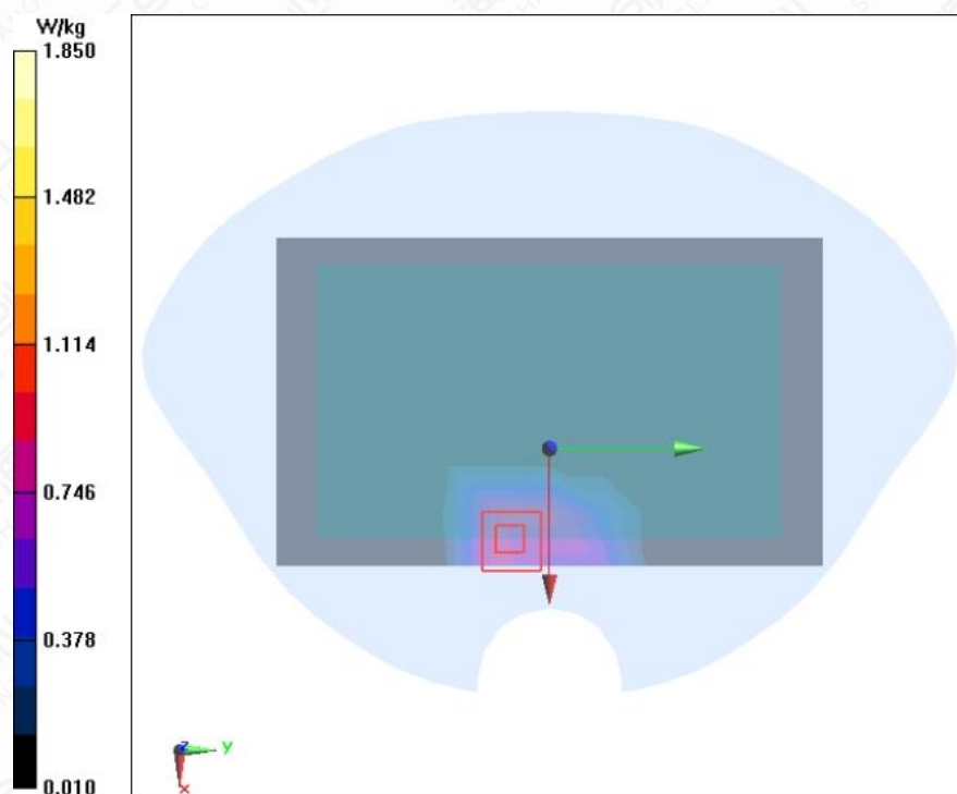
Figure A.1-6 LTE B12 10MHz 1RB 25offset Back Side Mode High 0mm
