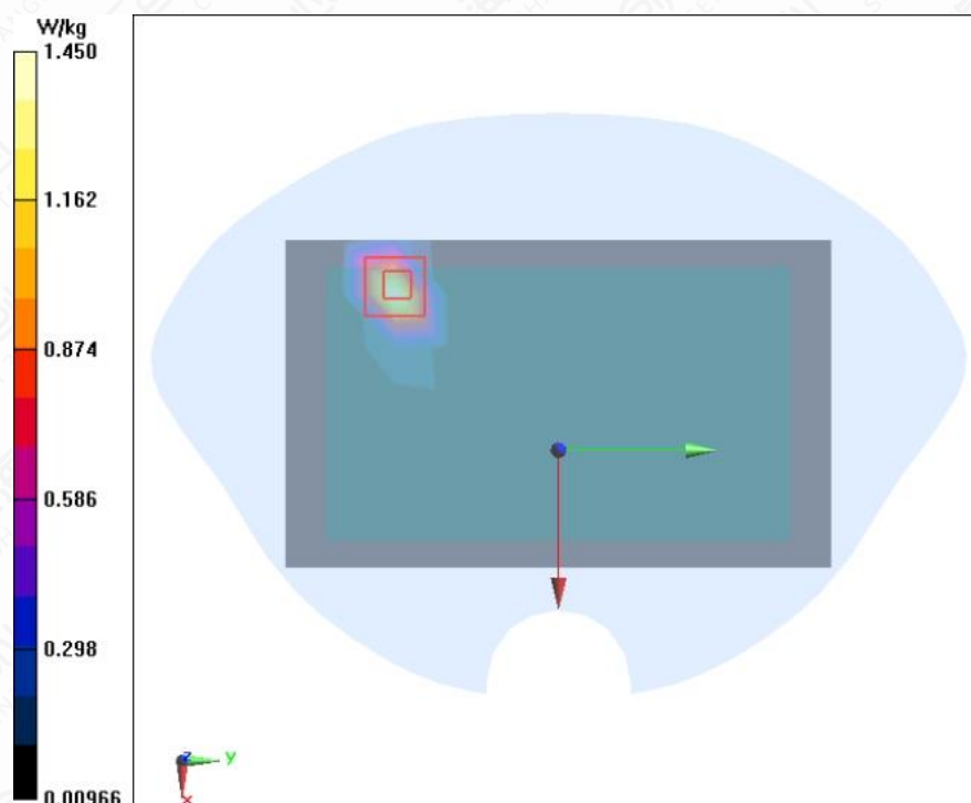
Figure A.1-11 Wi-Fi2.4G 802.11b Back Side Mode Middle 0mm
