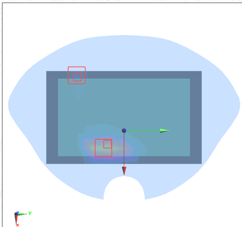
Figure A.1-26 LTE Band 13+Wi-Fi5G Back 0mm
