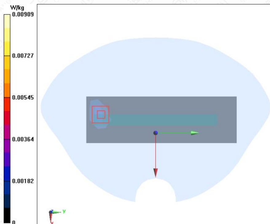
Figure A.1-14 BT 1-DH5 Top Side Mode Low 0mm
