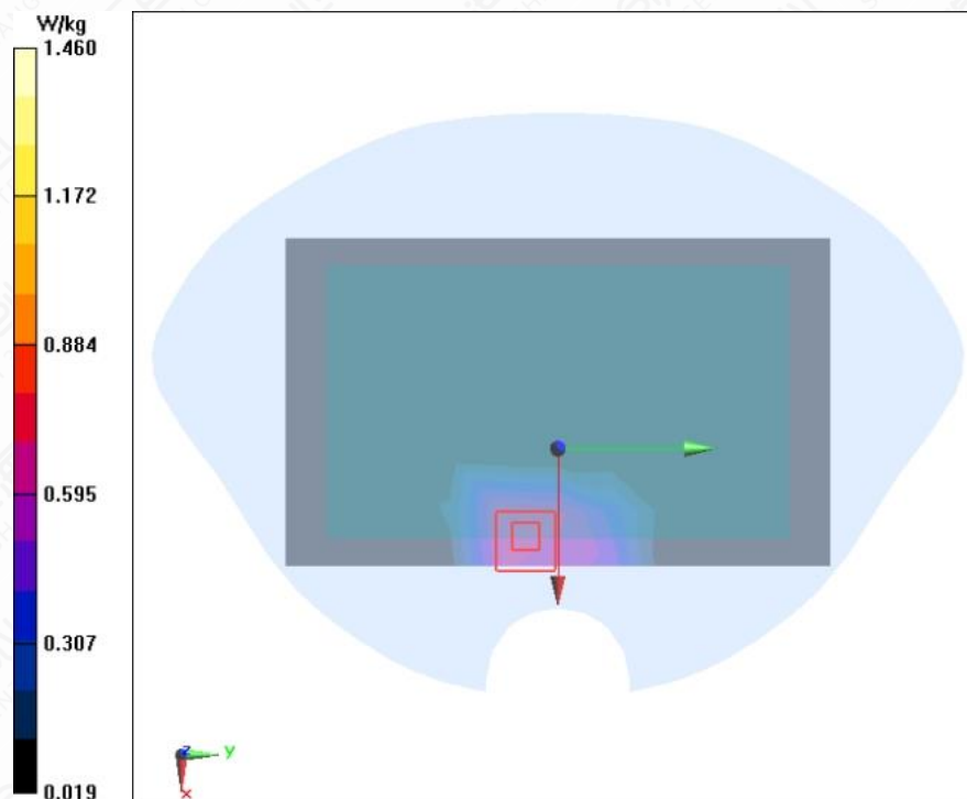
Figure A.1-9 LTE B66 20MHz 1RB 50offset Back Side Mode High 0mm
