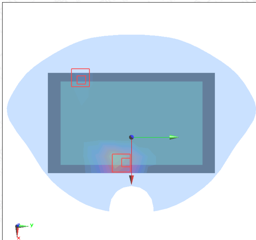
Figure A.1-22 LTE Band 5+Wi-Fi5G Back 0mm
