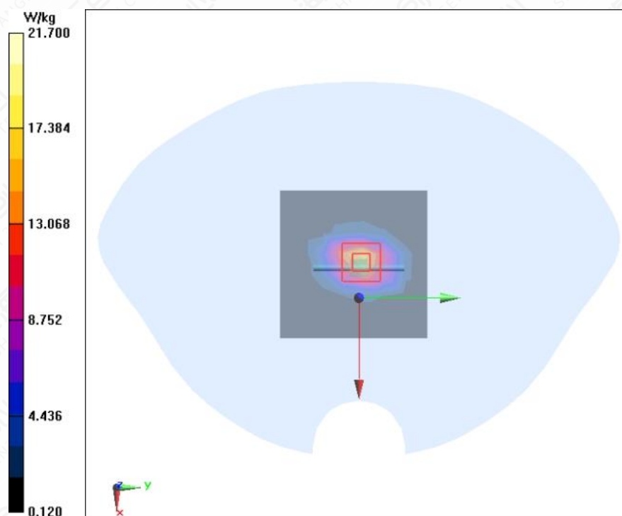
Figure A.2-6 System Check 2450MHz
