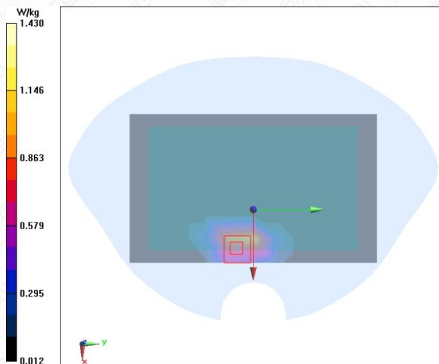
Figure A.1-2 WCDMA BandIV Back Side Mode Middle 0mm
