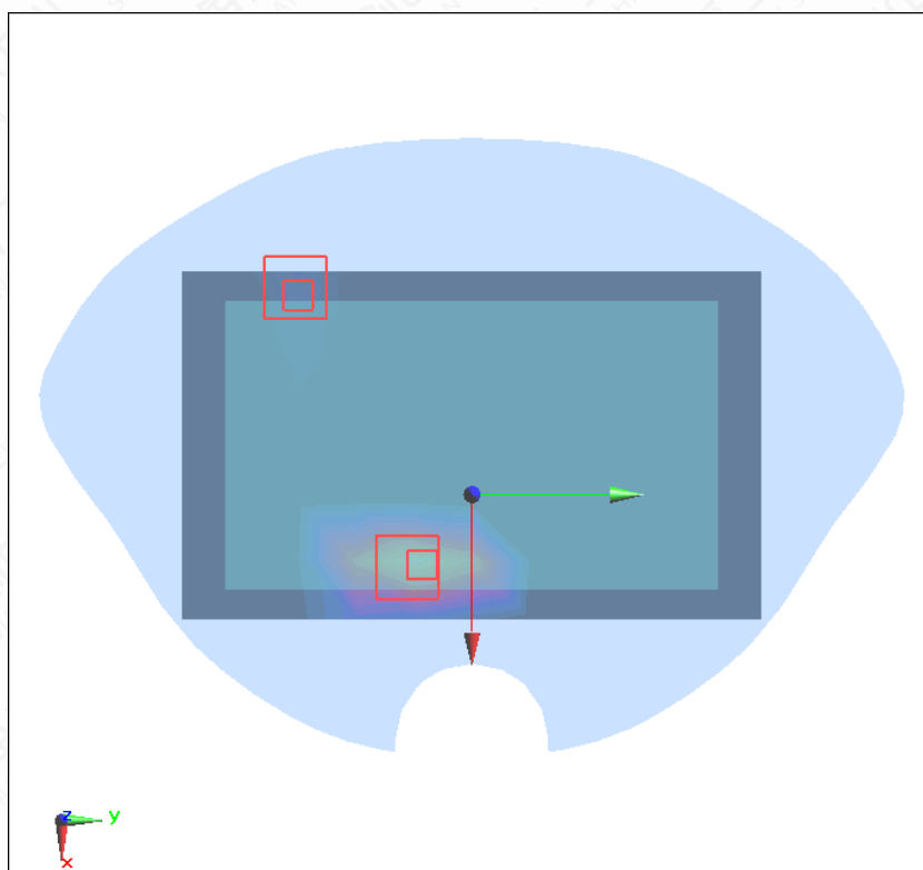
Figure A.1-28 LTE Band 14+Wi-Fi5G Back 0mm
