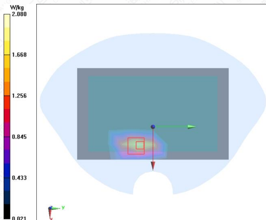
Figure A.1-8 LTE B14 10MHz 1RB 25offset Back Side Mode Middle 0mm
