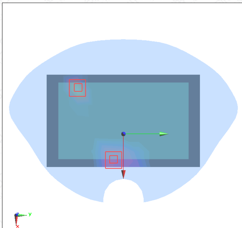
Figure A.1-31 LTE Band 71+Wi-Fi2.4G Back 0mm
