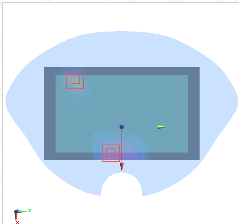
Figure A.1-23 LTE Band 12+Wi-Fi2.4G Back 0mm
