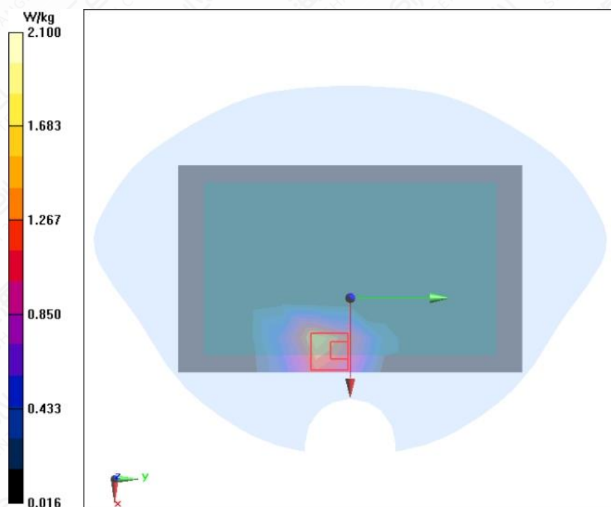
Figure A.1-5 LTE B5 10MHz 1RB 25offset Back Side Mode Low 0mm
