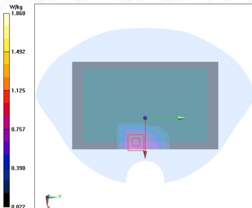
Figure A.1-10 LTE B71 20MHz 1RB 50offset Back Side Mode High 0mm
