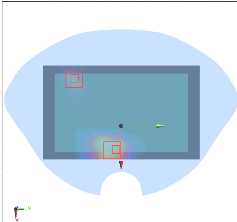
Figure A.1-21 LTE Band 5+Wi-Fi2.4G Back 0mm
