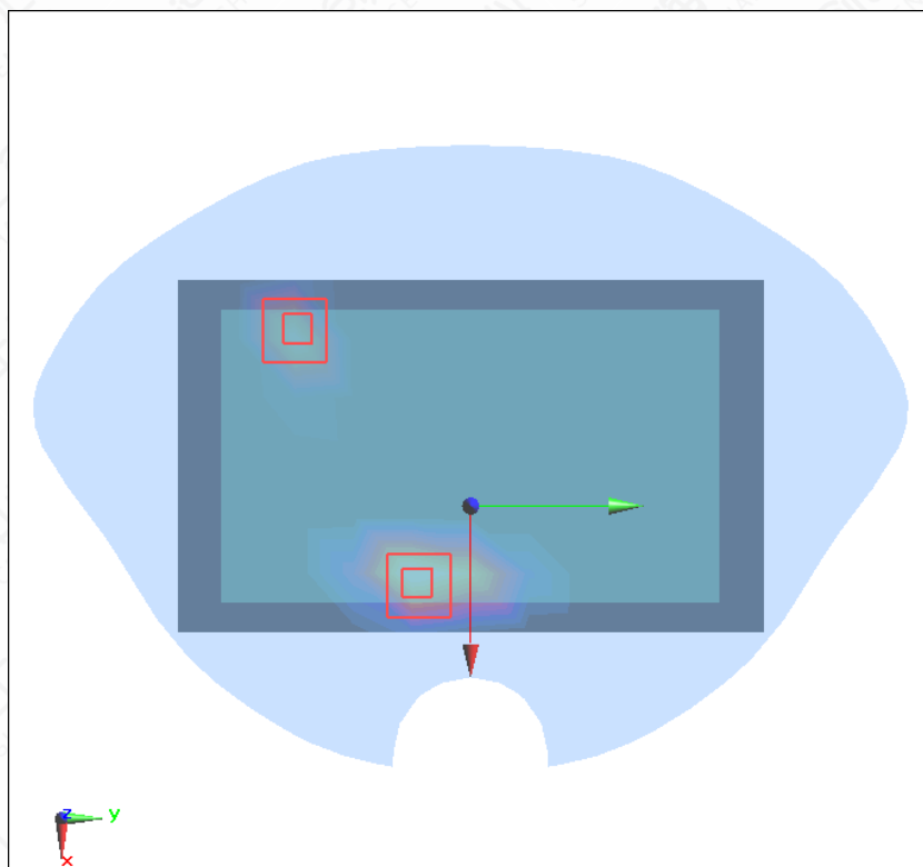
Figure A.1-15 WCDMA Band II +Wi-Fi2.4G Back 0mm
