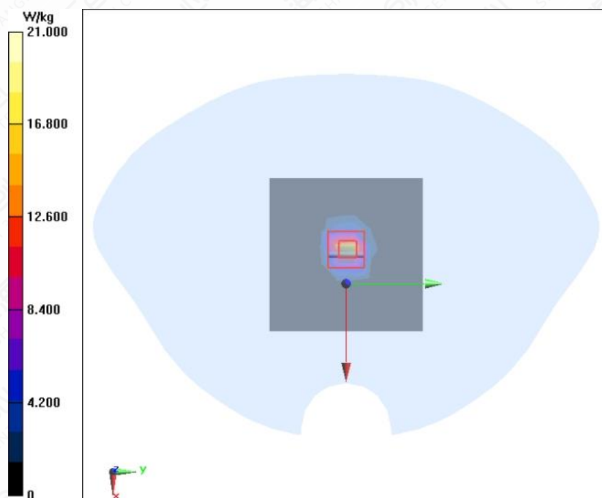
Figure A.2-8 System Check 5800MHz
