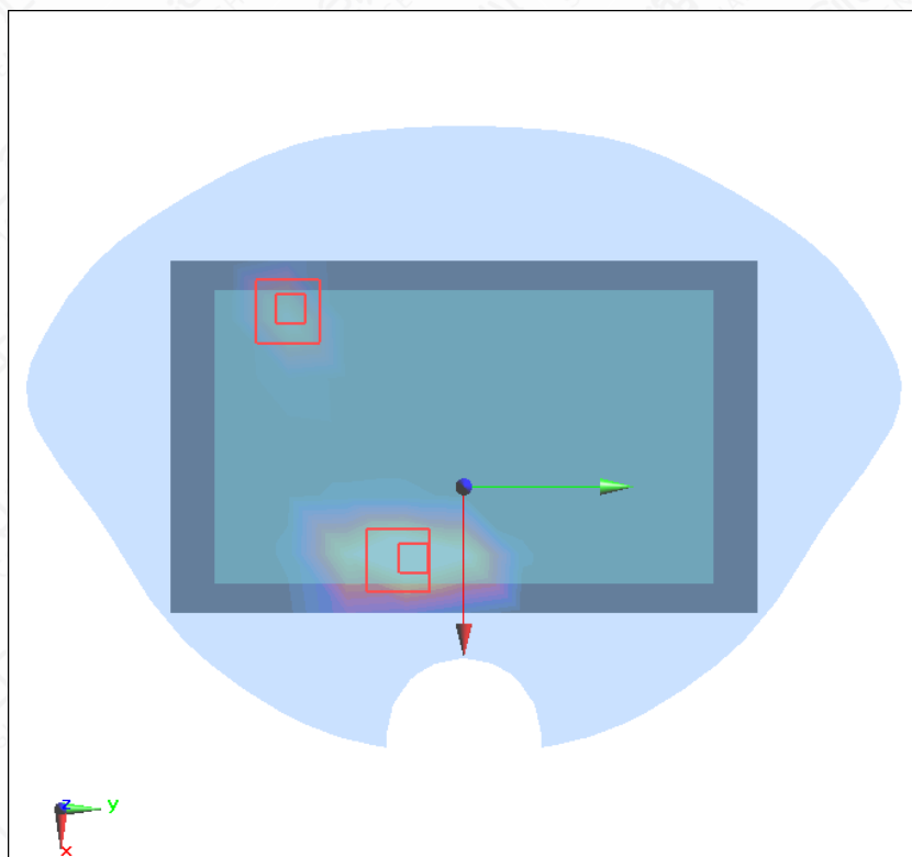
Figure A.1-27 LTE Band 14+Wi-Fi2.4G Back 0mm
