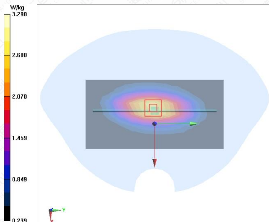
Figure A.2-3 System Check 835MHz
