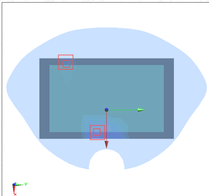
Figure A.1-24 LTE Band 12+Wi-Fi5G Back 0mm
