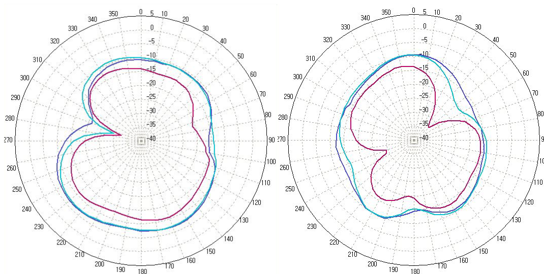
(a) Azimuth Plane (XY) – Vertical Polarization (Class 1/Class2)
