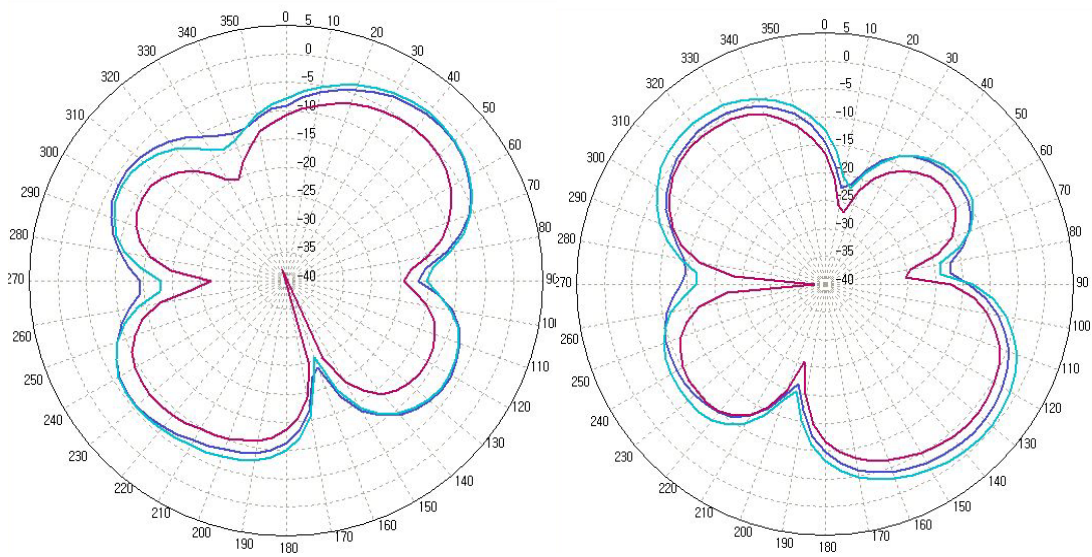
(c) Elevation2 Plane (YZ) – Horizontal Polarization (Class 1)
