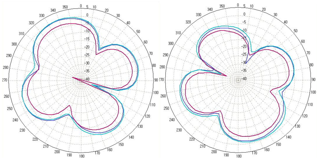
(c) Elevation2 Plane (YZ) – Horizontal Polarization (Class 1)
