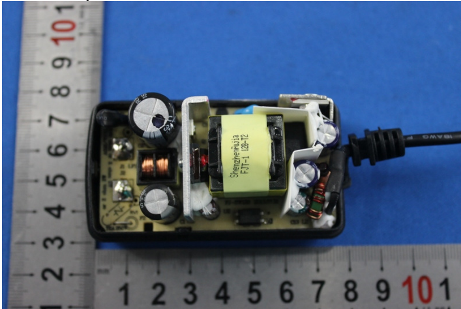
Alternate adapter: FJ-SW1501600N
