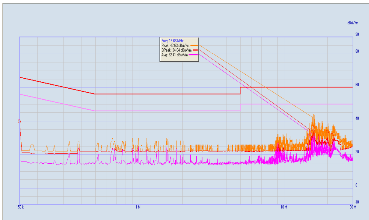
(Plot C: L Phase)
