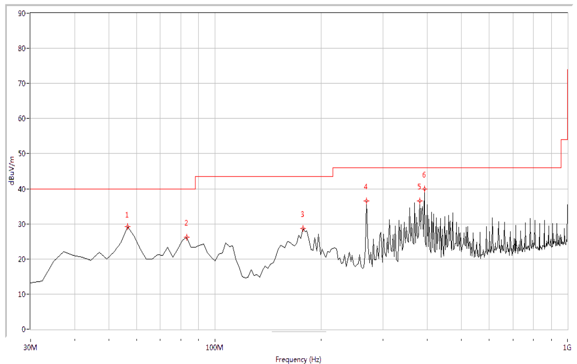
(Plot B: 30MHz – 1GHz, Test Antenna Vertical)
