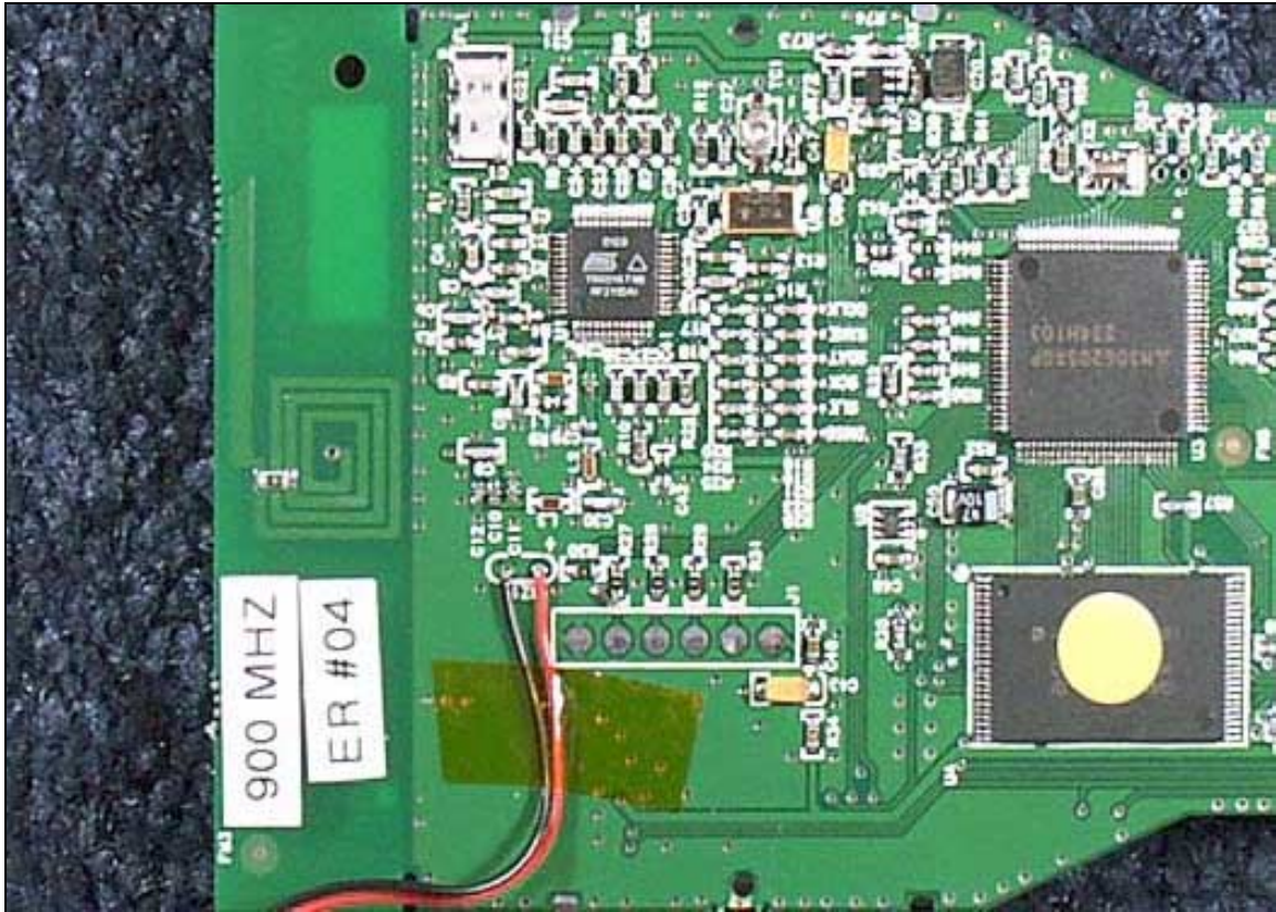
Remote PCB Front Close Up 1
