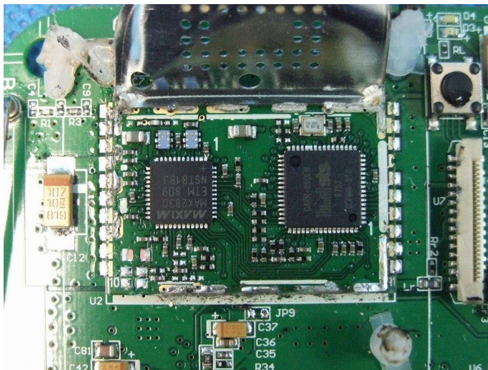
Fig. 6 – PCB view shield removed
