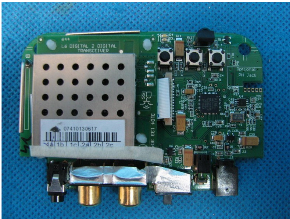
Fig. 2 – PCB view 1
