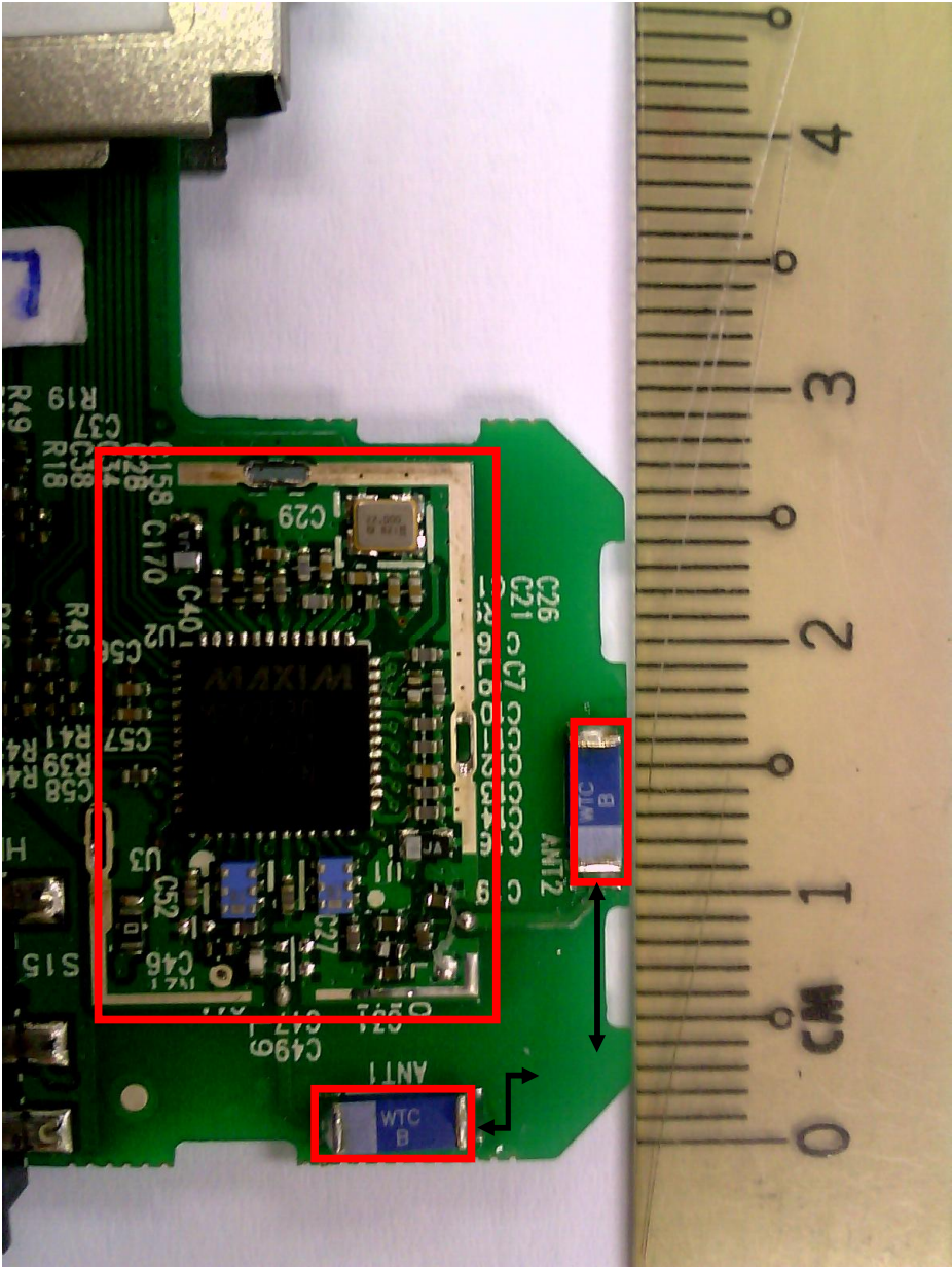
RF Module Circuit with RF Shield Removed RF Antenna
