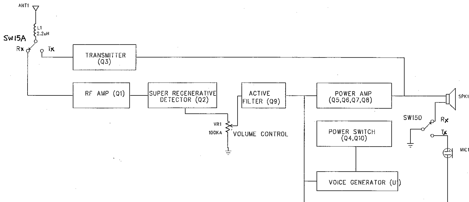
BLOCK DIAGRAM
