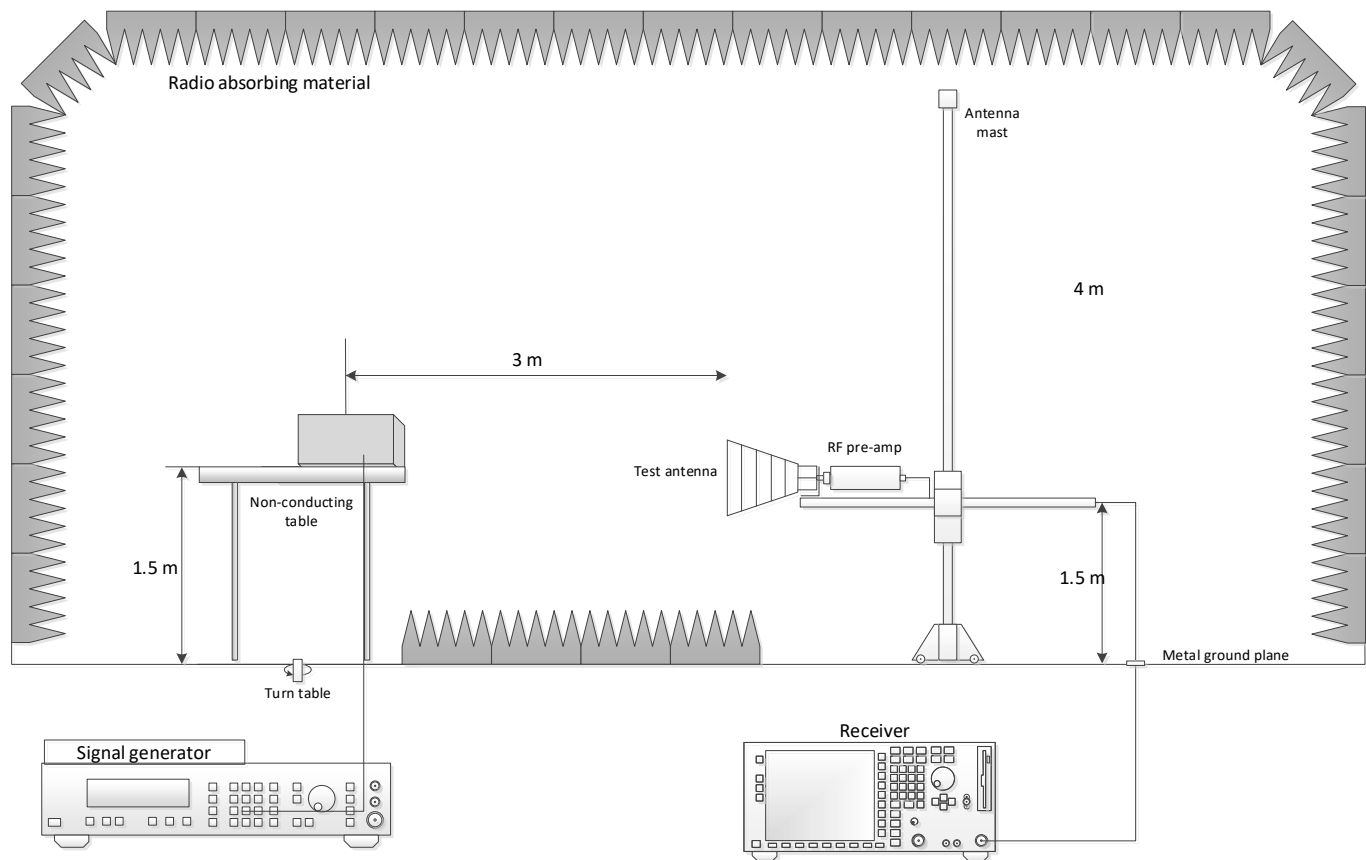
Figure 4.4-1: Test setup diagram
