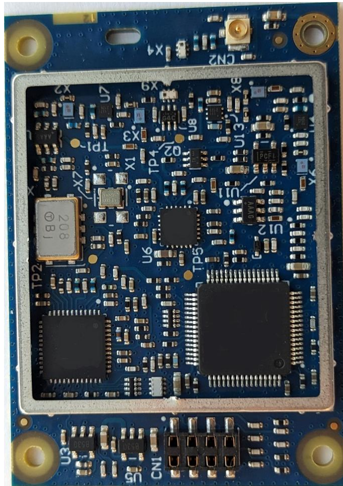
Figure 1 XPD2400 board's top view with shield's lid removed.
