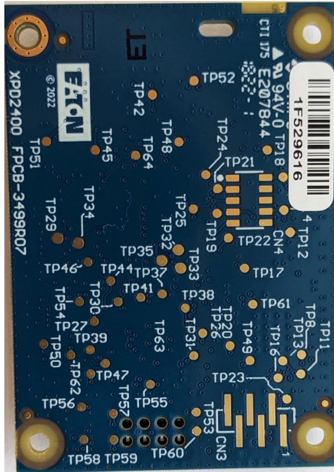
Figure 2 XPD2400 Bottom view.
