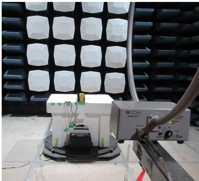
Figure 1: Radiated Emissions 10 kHz – 30 MHz
