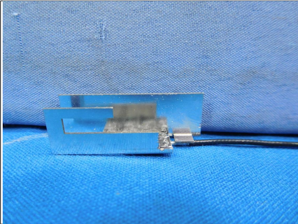
Antenna - 5GHz chain 2 & Bluetooth
