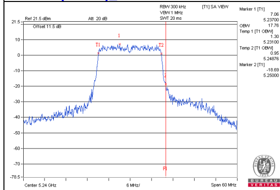
802.11ac(VHT20)_Chain0 / CH48
