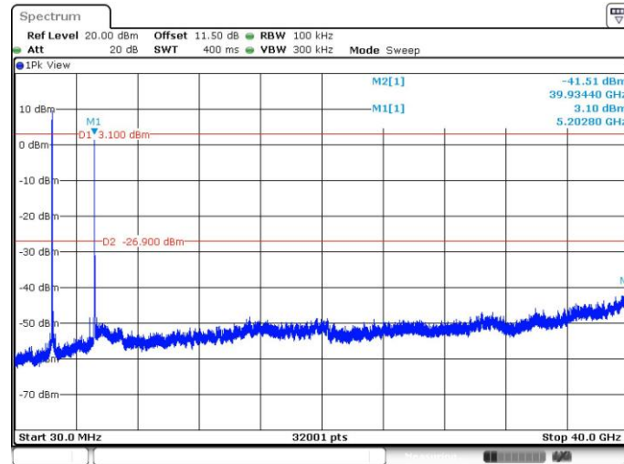
Conducted Emission Plot
