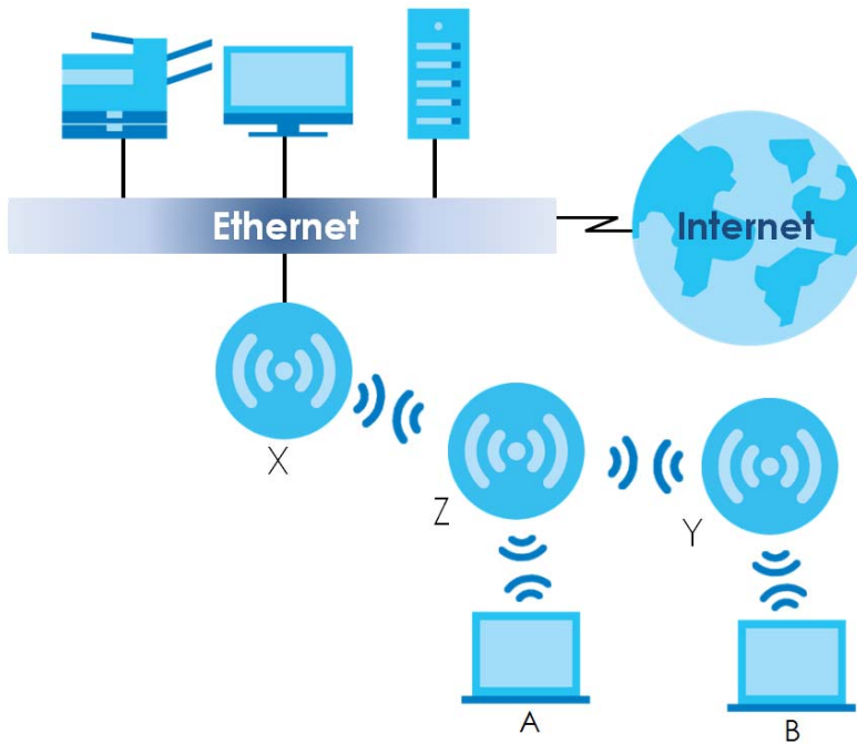
Figure 2 Repeater Application
