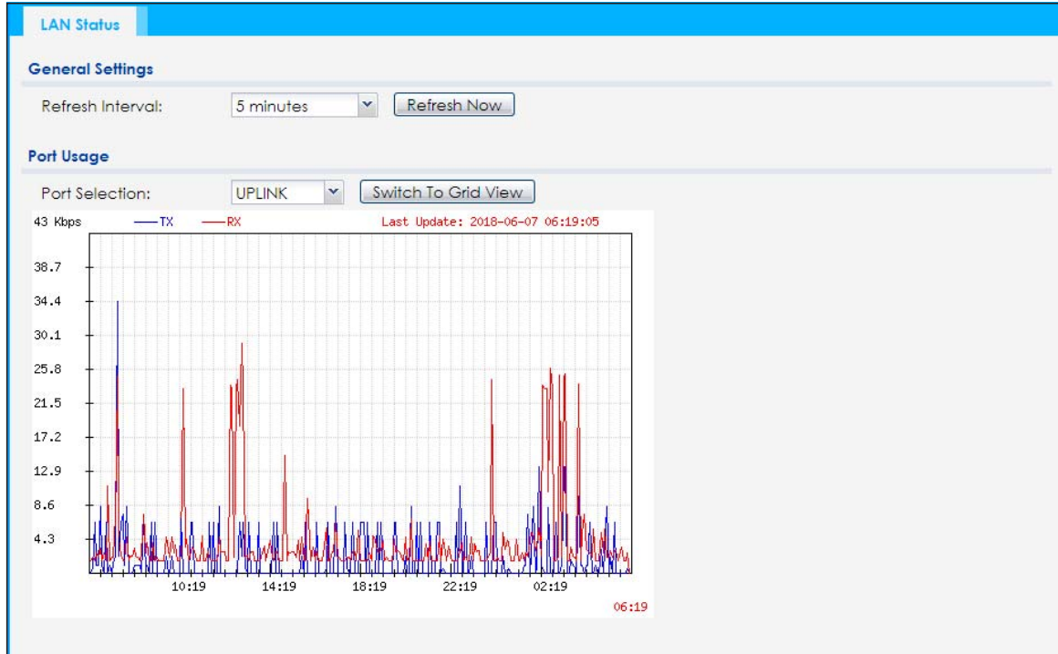
Figure 42 Monitor > Network Status > Switch to Graphic View
