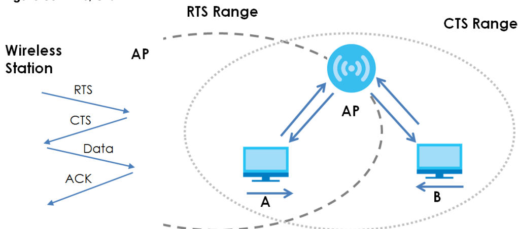
Figure 56 RTS/CTS
