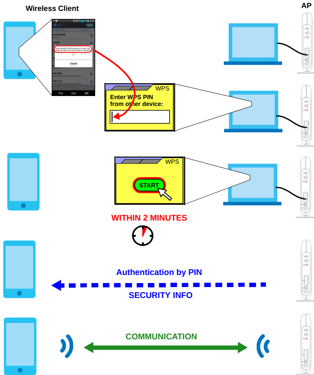
Figure 22 Example WPS Process: PIN Method
