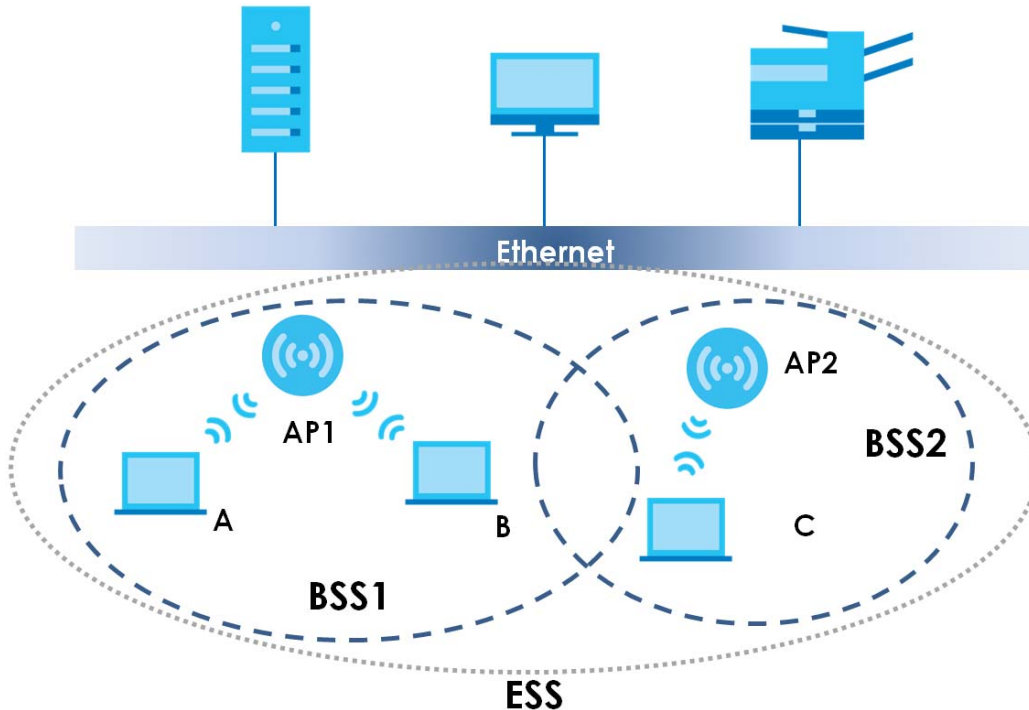
Figure 55 Infrastructure WLAN
