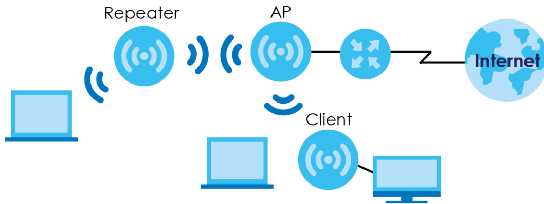
Figure 5 Device Operating Mode Example
