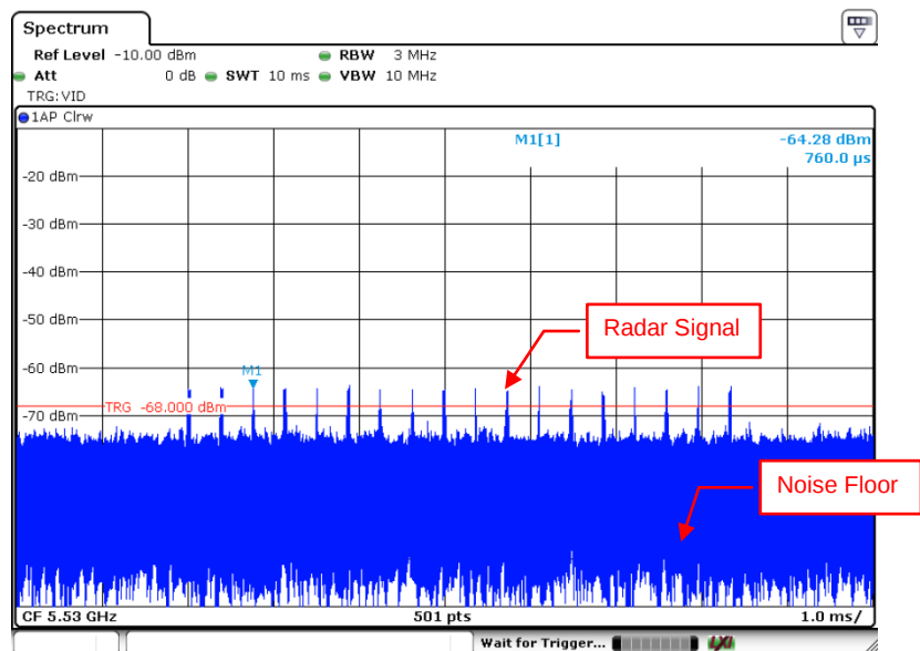
Radar Signal 2
