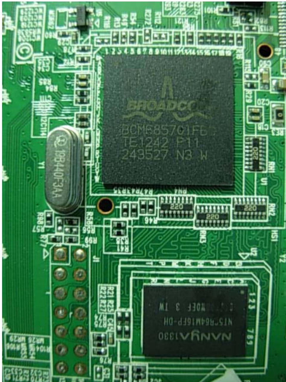
(12) EUT Photo (MB)
