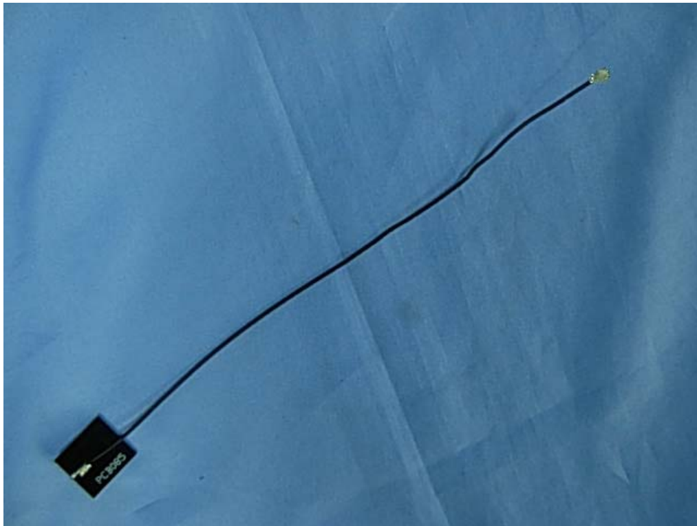
(17) EUT Photo (Right Antenna)
